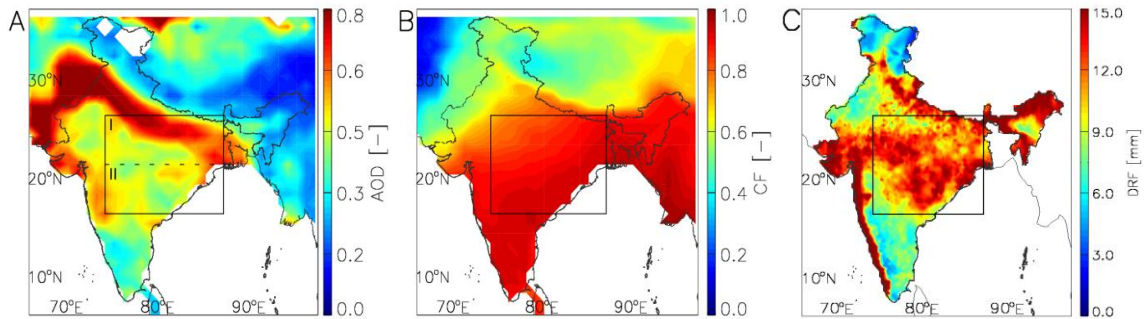
5 Figure 1. Climatological mean of A) aerosol optical depth, B) cloud fraction and C) daily rainfall for June through September 2002-2013. The black square box indicates the Indian summer monsoon region (ISMR) focussed in our analysis. Panel A illustrate the boundaries of regions I and II, used for sub analysis (see the text).
