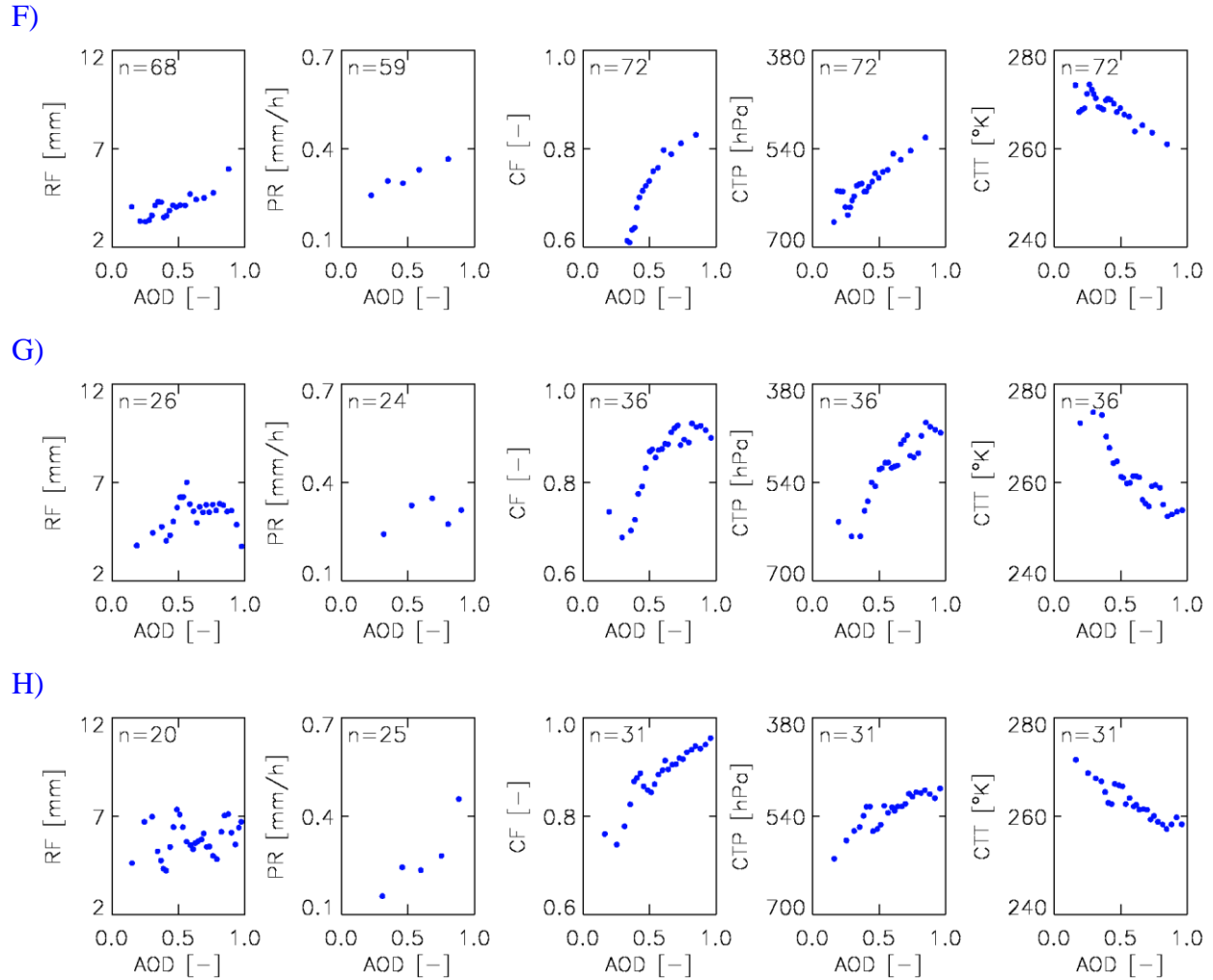
Figure A: Associations of accumulated daily rainfall, precipitation rate, cloud fraction, cloud top pressure and cloud top temperature with AOD for meteorology regime A) R1, B) R2, C) R3, D) R4, E) R5, F) R6, G) R7, H) R8 . The daily collocated measurements of these variables (except PR) with AOD from all the grids within ISMR during JJAS, 2002-2013 are sorted as a function of collocated AOD values (each variable separately), divided into 25 bins of 4 percentile each and averaged. In case of PR-AOD association, the number of sample points were greatly reduced within each regime so the dataset was divided into 5 equal bins of 20 percentile each and samples averaged. The number of samples (n) corresponding to each scatter point are indicated on the plot. The total number of samples used in these separate associations are equal to n times 50.
