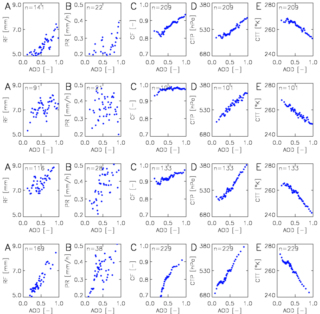
Figure: Associations of daily rainfall (A), precipitation rate (B), cloud fraction (C), cloud top
