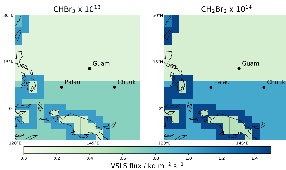
Figure 2. Surface emissions of \text{CHBr}_3 ( 10^{13} \text{kg/m}^2/\text{s} ) and \text{CH}_2\text{Br}_2 ( 10^{14} \text{kg/m}^2/\text{s} ) taken from Liang et al. (2010) for the time and study domain of the CAST and CONTRAST campaigns.
