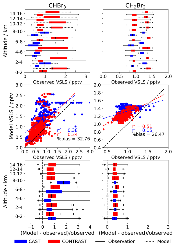
Figure 4. Comparison of model and observed (left panels) \text{CHBr}_3 (pptv) and (right panels) \text{CH}_2\text{Br}_2 (pptv) mole fraction data for CAST (denoted by blue) and CONTRAST (denoted by red). Top panels describe the comparison between model (dotted line) and observed (solid line) values as a box and whiskers plot on 2-km altitude bins. The middle panel describes the model and data comparison as a scatterplot. Pearson correlations ( r^2 ) and percentage biases are shown inset. Black, red, and blue dashed lines denote the 1:1 line, and the best fit linear models for CONTRAST and CAST, respectively. The bottom panel show the relative model error, described as a box and whiskers plot on 2-km altitude bins. The vertical dashed line denote the zero error line.
