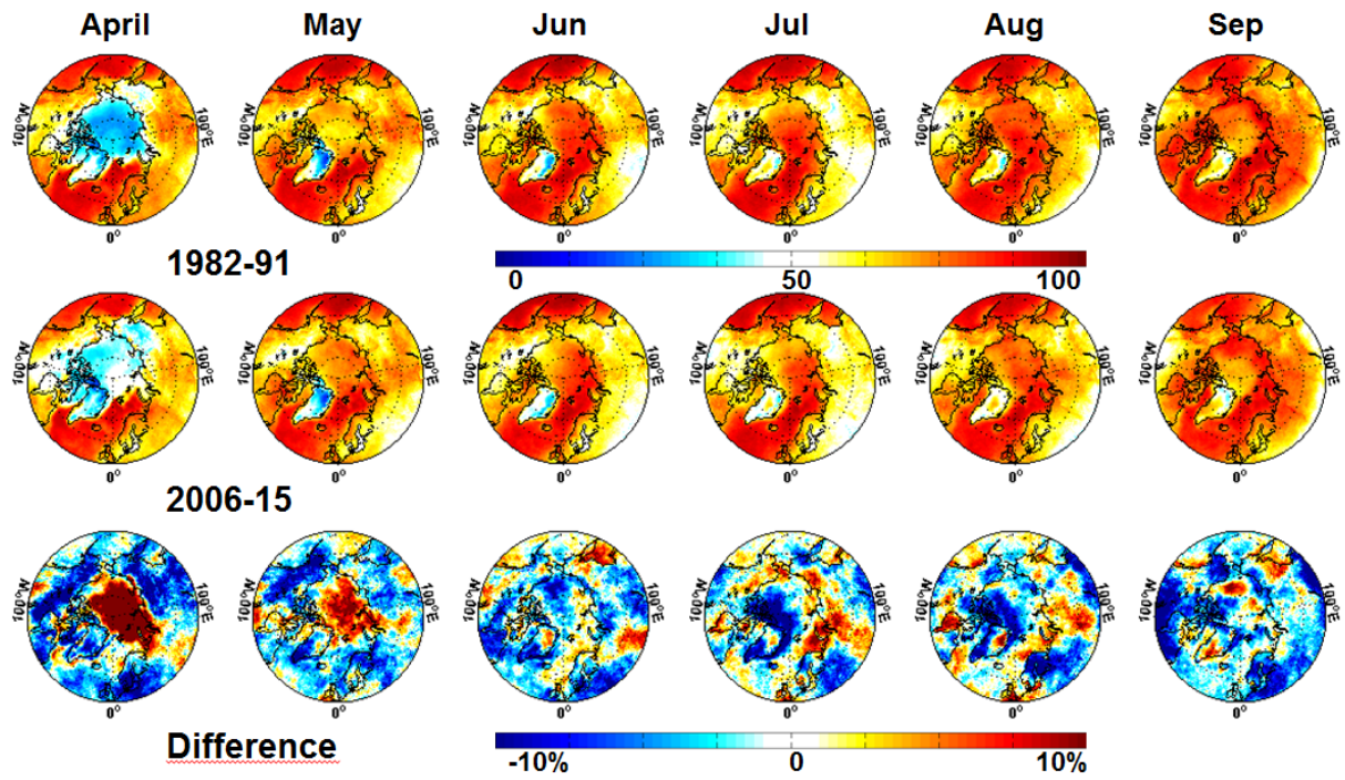
Figure 146: Arctic summer season mean cloudiness for the first CLARA-A2 decade (1982-1991, upper panel) compared to the last decade (2006-2015, middle panel). Difference plot (last minus first decade) shown in the lower panel. All values shown as %.
