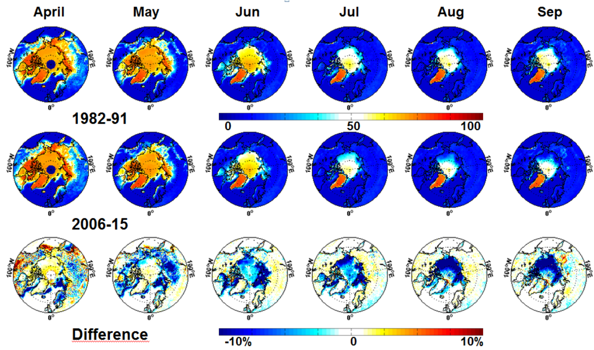
Figure 135: Arctic summer season mean surface albedo for the first CLARA-A2 decade (1982-1991, upper panel) compared to the last decade (2006-2015, middle panel). Difference plot (last minus first decade) shown in the lower panel. All values shown as %.
