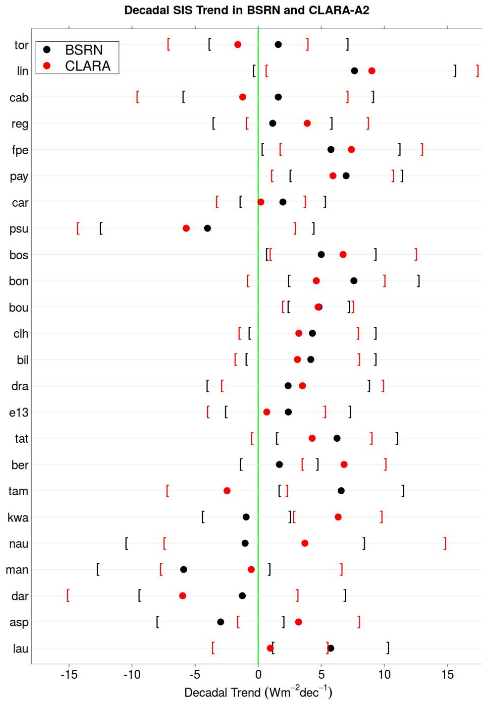
Figure 153: Decadal linear trends derived from the CLARA-A2 surface irradiance data record (red dots) with the corresponding trends derived from measurements obtained from the BSRN (black dots). Trends are shown as W m^{-2} (dec)^{-1} . The parentheses represent the confidence interval of the trends. See text for further details.
