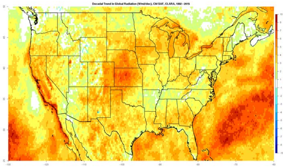
6 | Figure 164: Decadal linear trend of the surface irradiance from 1992 to 2015 based on the CLARA-A2 SIS 7 data record in (a) Central Europe and (b) parts of Northern America. All trends shown as W\ m^{-2}\ (dec)^{-1} .
