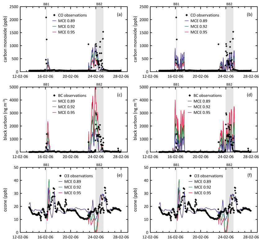
Fig. 2. Figure 6. Simulated CO using a) TAPM-CTM and b) CCAM-CTM, simulated BC using c) TAPM-CTM and d) CCAM-CTM, and simulated O3 using e) TAPM-CTM and f) CCAM-CTM. Coloured lines represent different MCE EF
