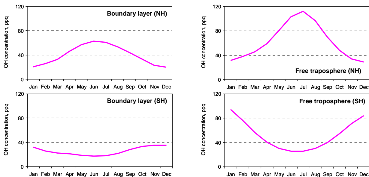
Figure S11. Seasonal variation of OH air concentration in 2013 simulated by MOZART (Emmons et al., 2010): (a) – in the boundary layer (< 1 km) of the Northern Hemisphere; (b) – in the free troposphere (1-10 km) of the Northern Hemisphere; (c) – in the boundary layer (< 1 km) of the Southern Hemisphere; (d) – in the free troposphere (1-10 km) of the Southern Hemisphere.
