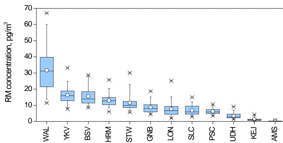
Figure S5. Model ensemble average annual air concentration of RM at selected measurement sites in 2013 simulated with no atmospheric chemistry applied by the models. Site codes are defined in Table S2.
