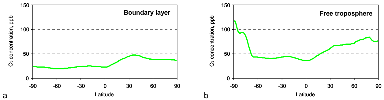
Figure S7. Global zonal-mean distribution of O 3 air concentration in 2013 simulated by MOZART (Emmons et al., 2010): (a) – in the boundary layer (< 1 km); (b) – in the free troposphere (1-10 km).
