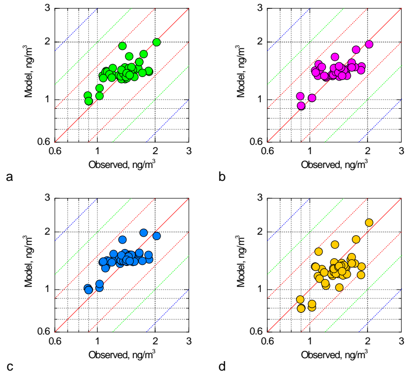
Figure S2. Scatter plots of annual mean GEM air concentration in 2013 measured at selected ground-based sites vs. simulated by different models: (a) – GLEMOS; (s) – GEOS-Chem; (c) – GEM-MACH-Hg; (d) – ECHMERIT. Red solid line depicts the 1:1 ratio; dashed lines show different deviation levels: red – by factor of 1.5, green – by factor of 2, blue – by factor of 3.
