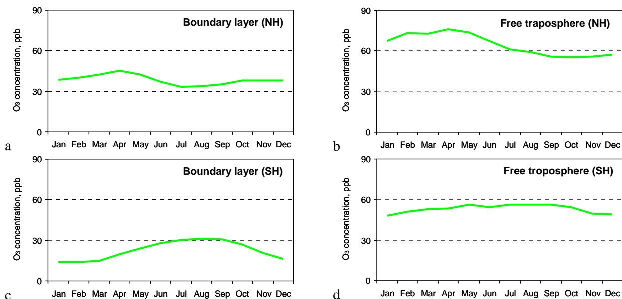
Figure S10. Seasonal variation of O 3 air concentration in 2013 simulated by MOZART (Emmons et al., 2010): (a) – in the boundary layer (< 1 km) of the Northern Hemisphere; (b) – in the free troposphere (1-10 km) of the Northern Hemisphere; . (c) – in the boundary layer (< 1 km) of the Southern Hemisphere; (d) – in the free troposphere (1-10 km) of the Southern Hemisphere.
