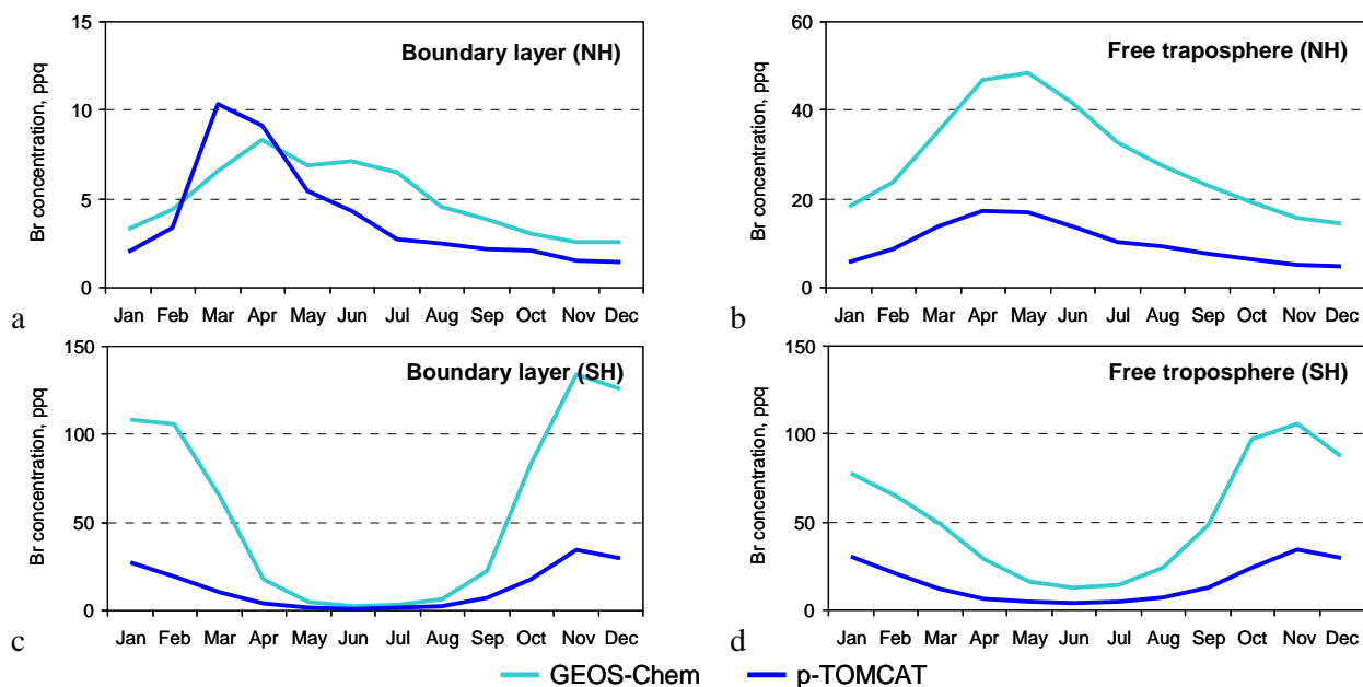
Figure S9. Seasonal variation of Br air concentration in 2013 simulated by GEOS-Chem (Parrella et al., 2012) and p-TOMCAT (Yang et al., 2005; 2010): (a) – in the boundary layer (< 1 km) of the Northern Hemisphere; (b) – in the free troposphere (1-10 km) of the Northern Hemisphere; . (c) – in the boundary layer (< 1 km) of the Southern Hemisphere; (d) – in the free troposphere (1-10 km) of the Southern Hemisphere.
