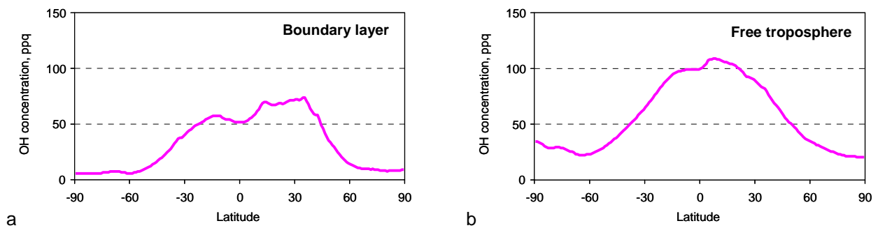
Figure S8. Global zonal-mean distribution of OH air concentration in 2013 simulated by MOZART (Emmons et al., 2010): (a) – in the boundary layer (< 1 km); (b) – in the free troposphere (1-10 km).
