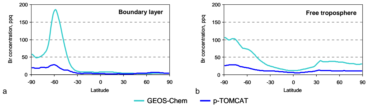
Figure S6. Global zonal-mean distribution of Br air concentration in 2013 simulated by GEOS-Chem (Parrella et al., 2012) and p-TOMCAT (Yang et al., 2005; 2010): (a) – in the boundary layer (< 1 km); (b) – in the free troposphere (1-10 km).
