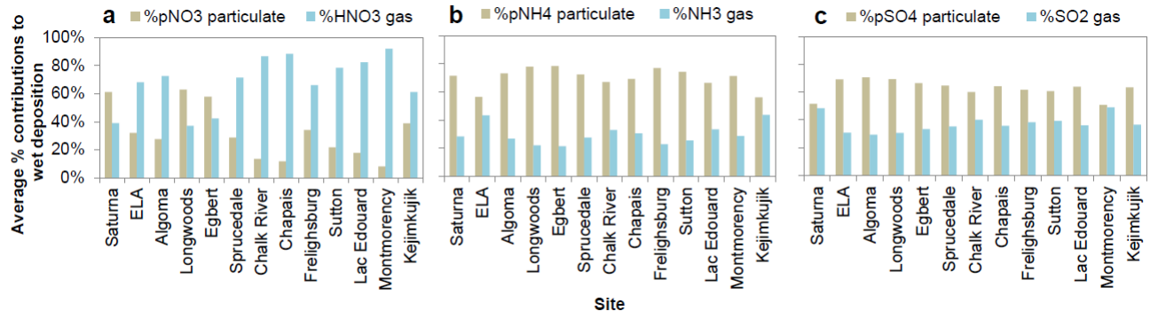
Figure 9: Average percent contributions of gas and particulate-phase species to nitrate (a), ammonium (b), and sulfate (c) wet deposition.
