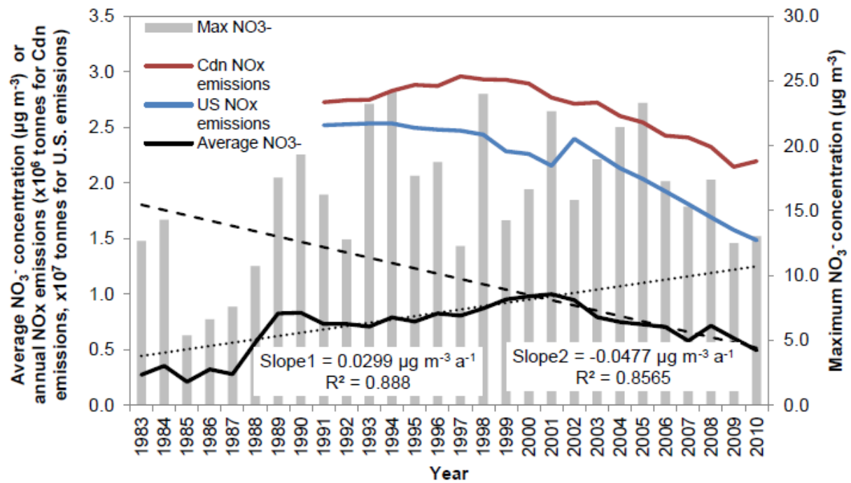
Figure 3: Temporal trends of annual atmospheric \text{NO}_3^- and annual \text{NO}_x emissions. Slope1 refers to the regression line for \text{NO}_3^- between 1991 and 2001 (positive trend, 3.6% increase), while Slope2 is for the period between 2001 and 2010 (negative trend, 6.5% decrease). Between 1991 and 1997, \text{NO}_x emissions in Canada (Cdn) increased by 8.5%. Between 1997 and 2010, Cdn \text{NO}_x emissions decreased by 25.8%.
