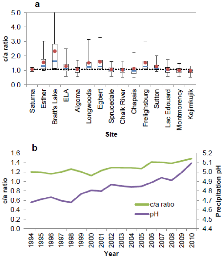
Figure 5: Geographical patterns of cation/anion ( c/a ) ratio (a) and temporal trends of annual average c/a ratio and precipitation pH (b). In (a), the blue line indicates the median; the red dot indicates the mean; the box and whiskers include the interquartile range and the 5 th to 95 th percentile range, respectively; the dotted line is the overall median among the sites.
