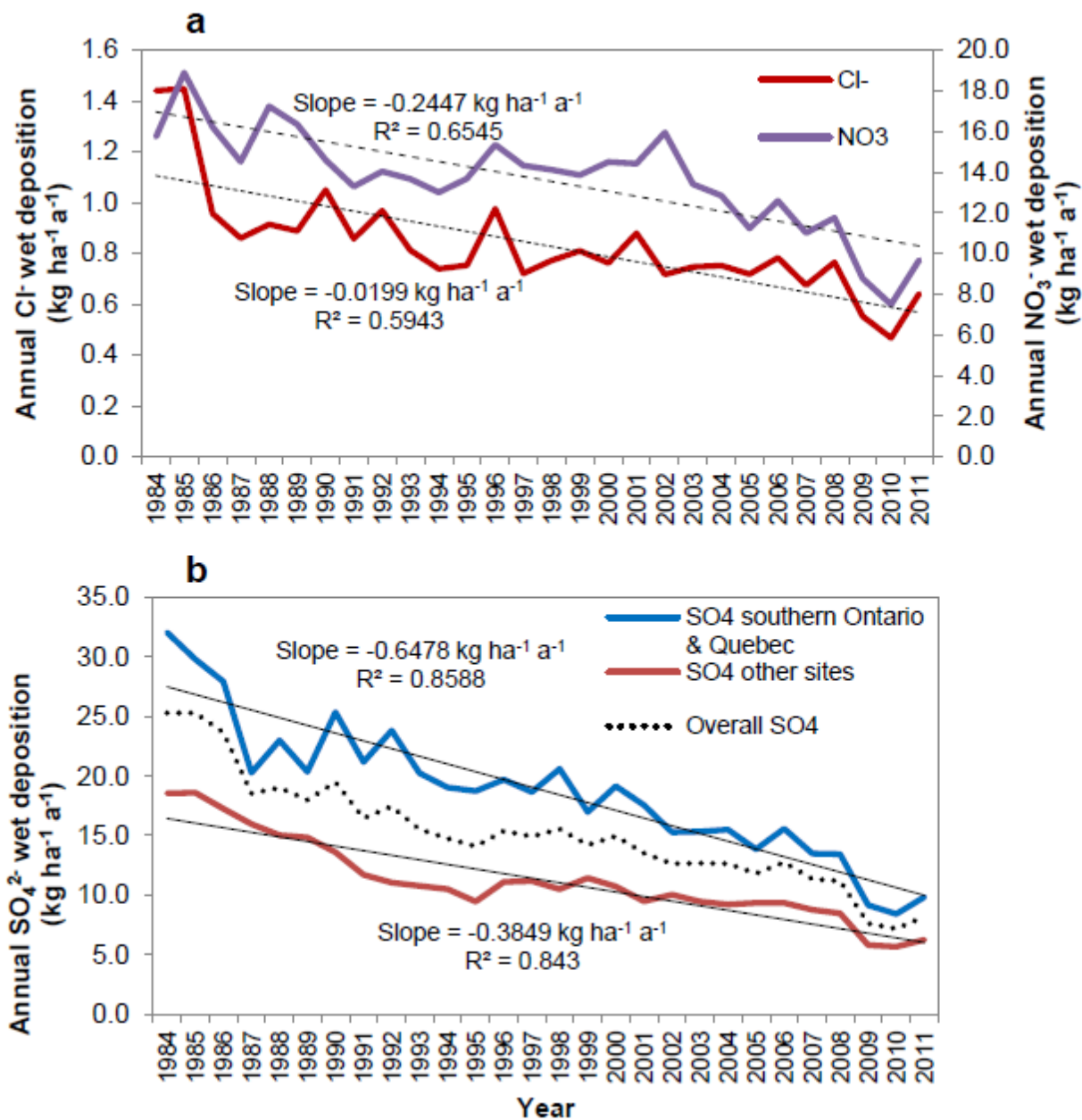
Figure 7: Temporal trends of annual wet deposition of Cl - and NO 3 - (a) and SO 4 2- (b).
