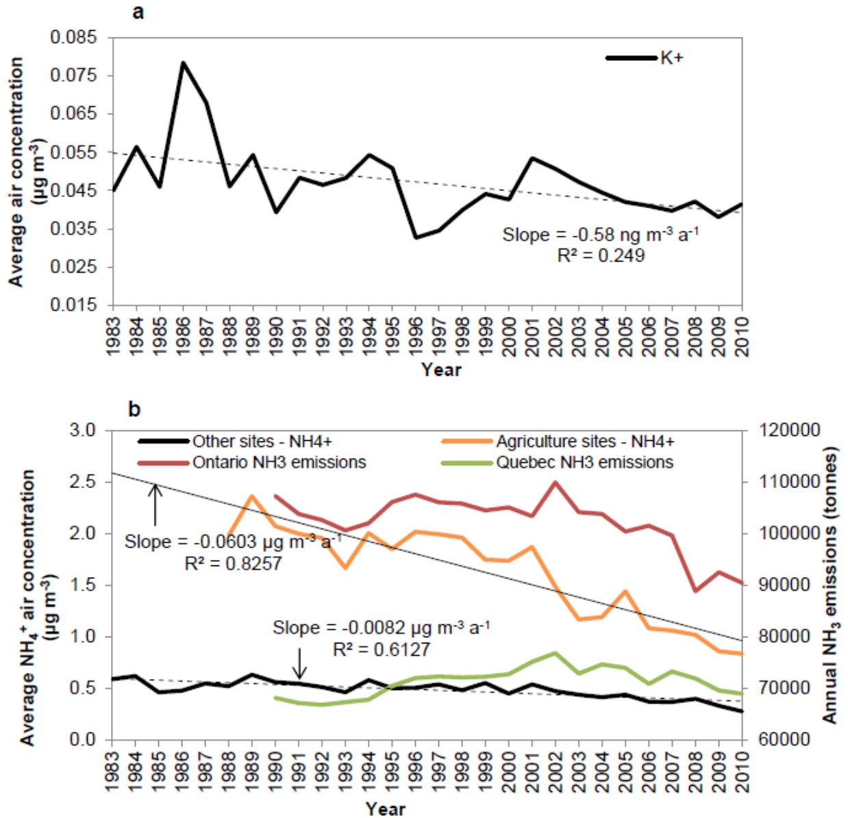
Figure 2: Temporal trends of annual average atmospheric K + (a) and atmospheric NH 4 + and annual ammonia emissions (b). In (b) between 2002 and 2010, atmospheric NH 4 + at agricultural sites decreased by 6.3% while ammonia emissions in Ontario and Quebec decreased by 2.4% and 1.1%, respectively.
