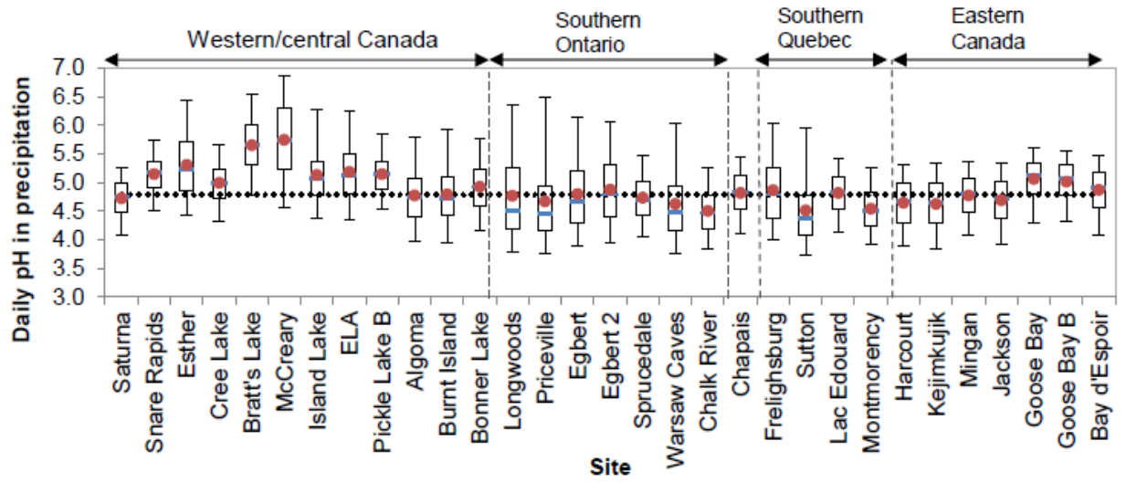
Figure 8: Geographical patterns of precipitation pH. See Fig. 6 caption.
