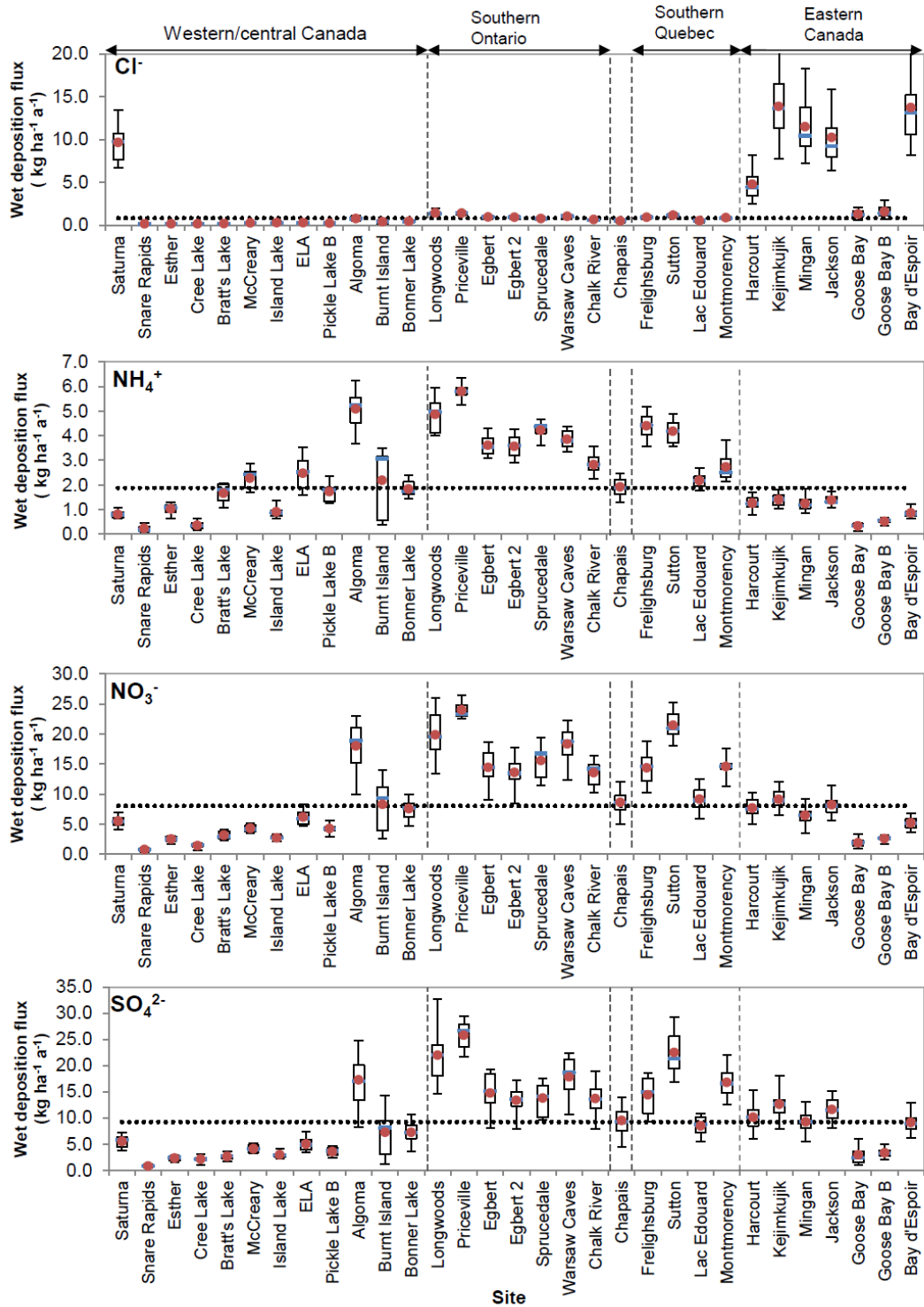
Figure 6: Geographical patterns of the annual wet deposition of ions. Sites are arranged in order from western to eastern Canada. The blue line indicates the median; the red dot indicates the mean; the box and whiskers include the interquartile range and the 5 th to 95 th percentile range, respectively; the dotted line is the overall median among the sites.
