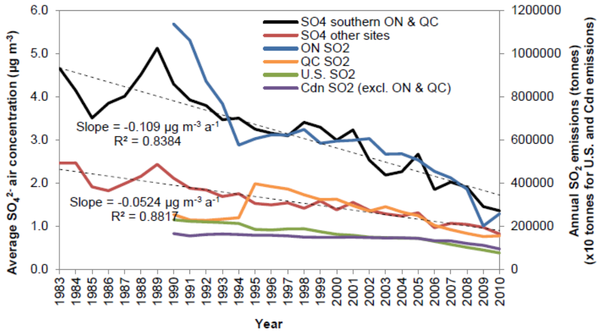
Figure 4: Temporal trends of annual average atmospheric SO 4 - and annual SO 2 emissions. ON and QC refer to the province of Ontario and Quebec, respectively. Between 1990 and 2010, atmospheric SO 4 - decreased by 4.5% at southern Ontario (ON) and Quebec (QC) sites and by 3.6% at other sites. Over the same period, SO 2 emissions decreased by 1.8% in Canada (Cdn) and 4.3% in the U.S.
