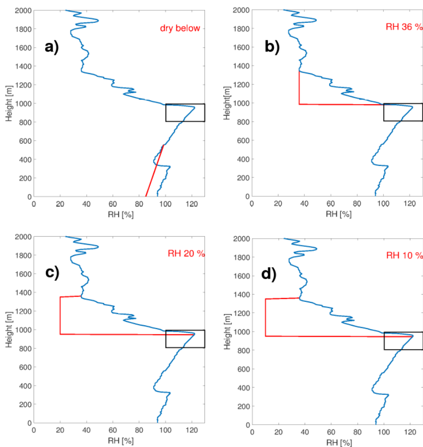
Figure 2. RH profiles for the sensitivity experiment SensMoist simulations. Modified parts of the RH profile are shown in red. The initial RH profile is in blue. (a) RH profile for the simulation with dry-air advection below the cloud. (b) shows the RH profile of the simulation with the dry-air advection above the cloud with the RH of 36 %, (c) and (d) show simulations with the dry-air advection above the cloud with the RH of 20 % and 10 %, respectively. Black box marks the vertical extent of the liquid cloud layer of the control simulation.
