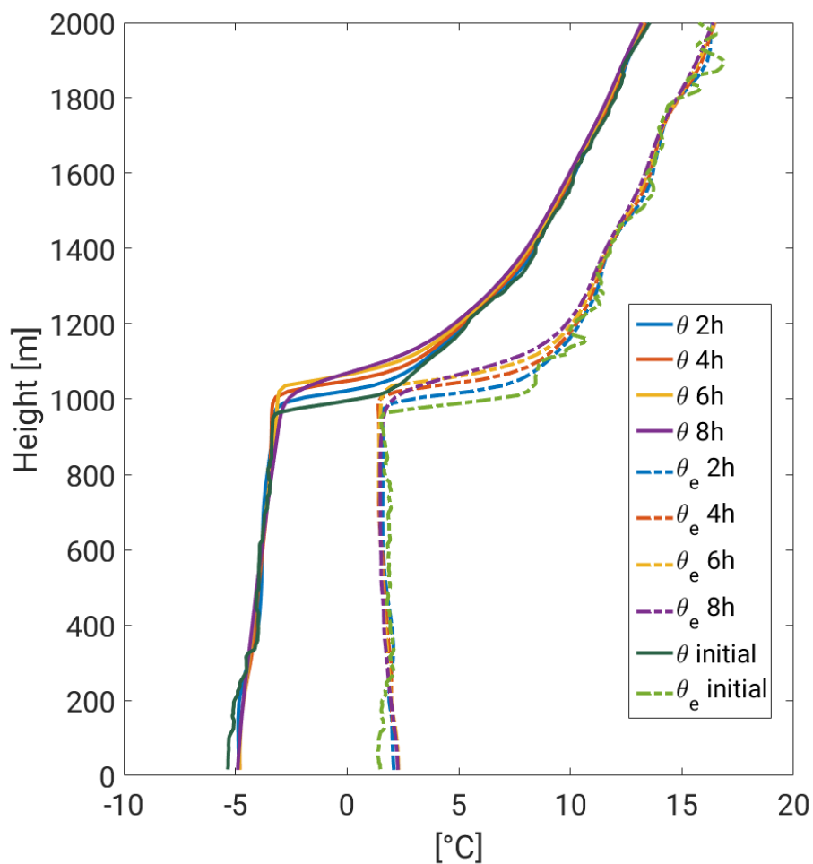
Figure 9. \theta (left) and \theta_e (right) profiles of the initial conditions (dark green and green) and after 2 h (blue), 4 h (orange), 6 h (yellow) and 8 h (purple) after the start of the SensIce simulation with an ice crystal concentration 101^{-1} .
