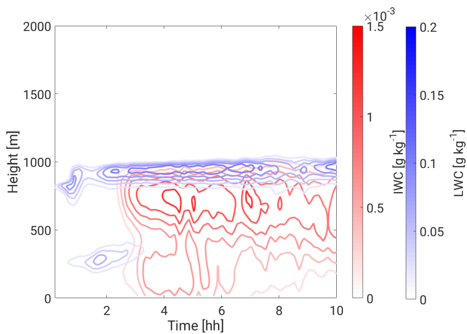
Figure 6. Mean values of LWC (blue) and IWC (red) for the SensMoist simulation with the RH of 10% above the cloud top.
