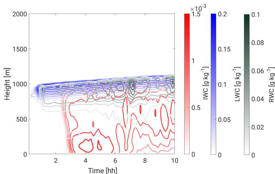
Figure 4. Mean values of LWC (blue), IWC (red) and RWC (green) for the control simulation.
