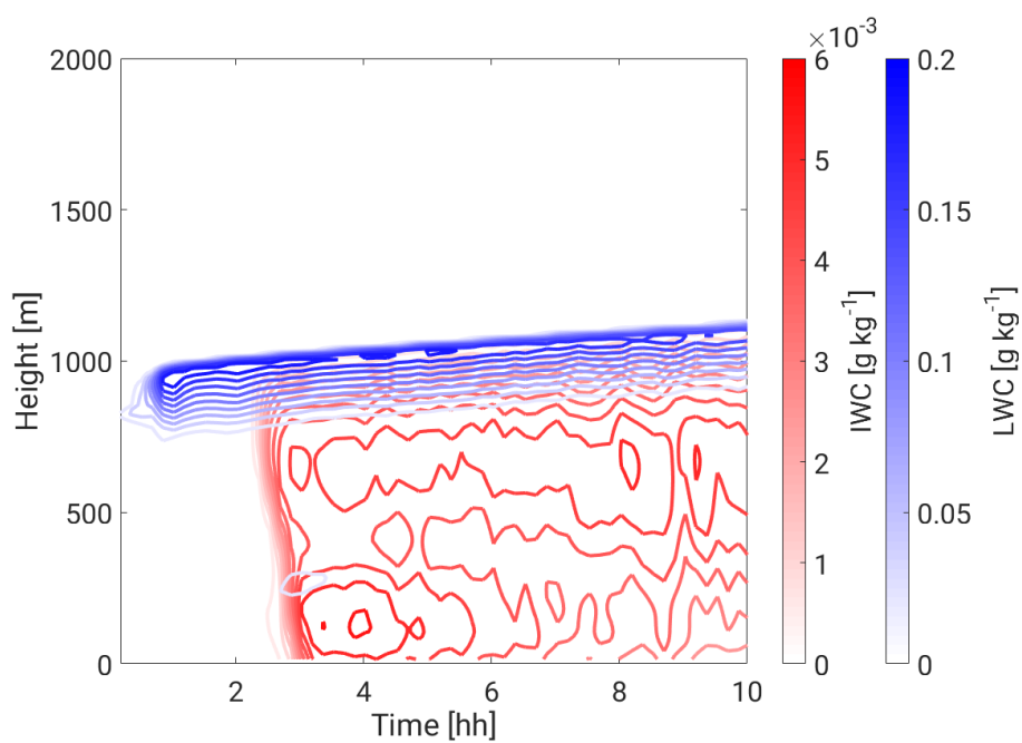
Figure 8. Mean values of LWC (blue) and IWC (red) of the SensIce simulation with an ice crystal concentration value of 11^{-1} .
