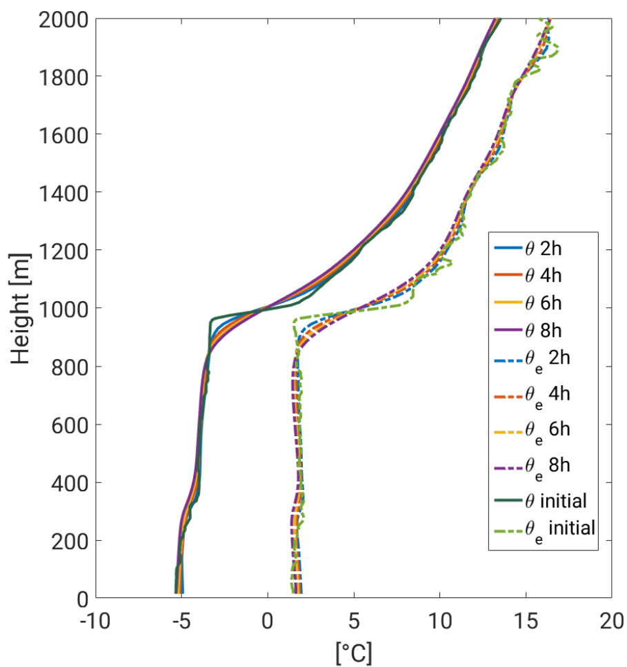
Figure 10. \theta (left) and \theta_e (right) profiles of the initial conditions (dark green and green) and after 2 h (blue), 4 h (orange), 6 h (yellow) and 8 h (purple) after the start of the SensCDNC simulation with a decreased CDNC of 2 \text{ cm}^{-3} .
