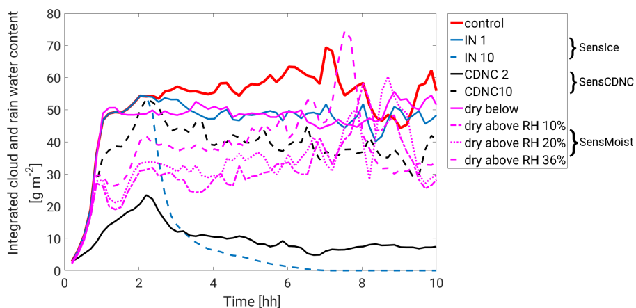
Figure 5. The domain-averaged LWP (including cloud droplets and rain) for the control simulation (red), the simulation of dry-air advection below the cloud (pink solid), the simulations of dry-air advection above the cloud top with a RH of 36 % (pink dashed), a RH of 20 % (pink dotted) and a RH of 10 % (pink dash-dotted), the simulations with an ice crystal concentration of 11^{-1} (blue solid) and 101^{-1} (blue dashed), the simulation with a CDNC of 10 \text{ cm}^{-3} (black dashed) and a CDNC of 2 \text{ cm}^{-3} (black solid).
