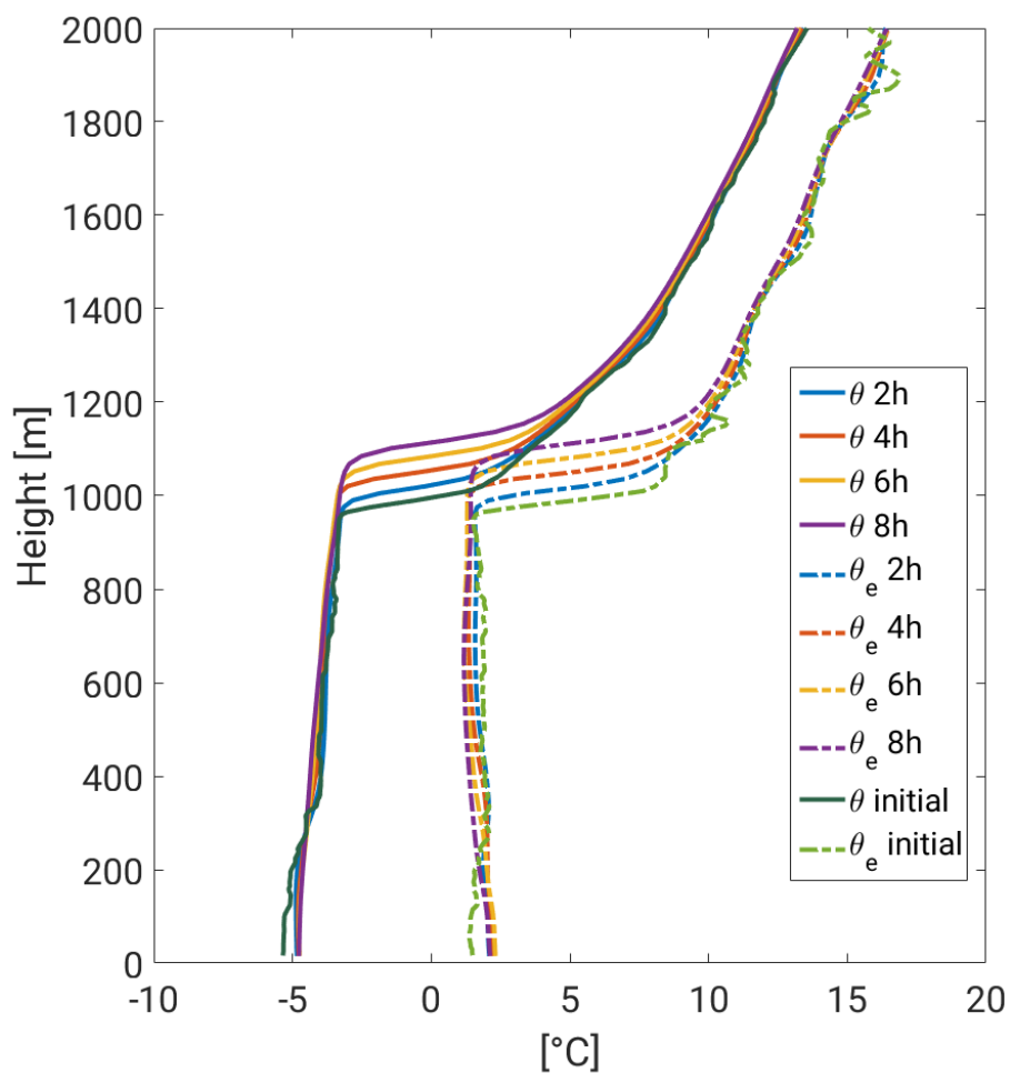
Figure 3. \theta (left) and \theta_e (right) profiles of the initial conditions (dark green and green), and after 2 h (blue), 4 h (orange), 6 h (yellow) and 8 h (purple) from the start of the control simulation.
