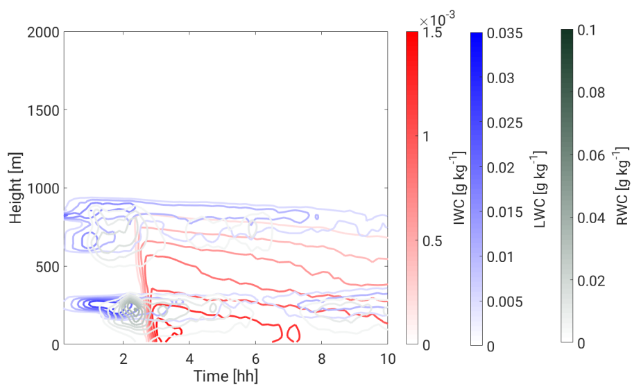
Figure 11. Mean values of LWC (blue), IWC (red) and RWC (green) of the SensCDNC simulation with 2 \text{ cm}^{-3} CDNC.
