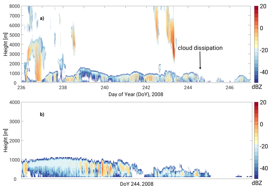
Figure 1. Radar reflectivity factor (colours, dBZ) contour time series for the period DoY 236 to 246 during 2008 (a) and for DoY 244 (b).
