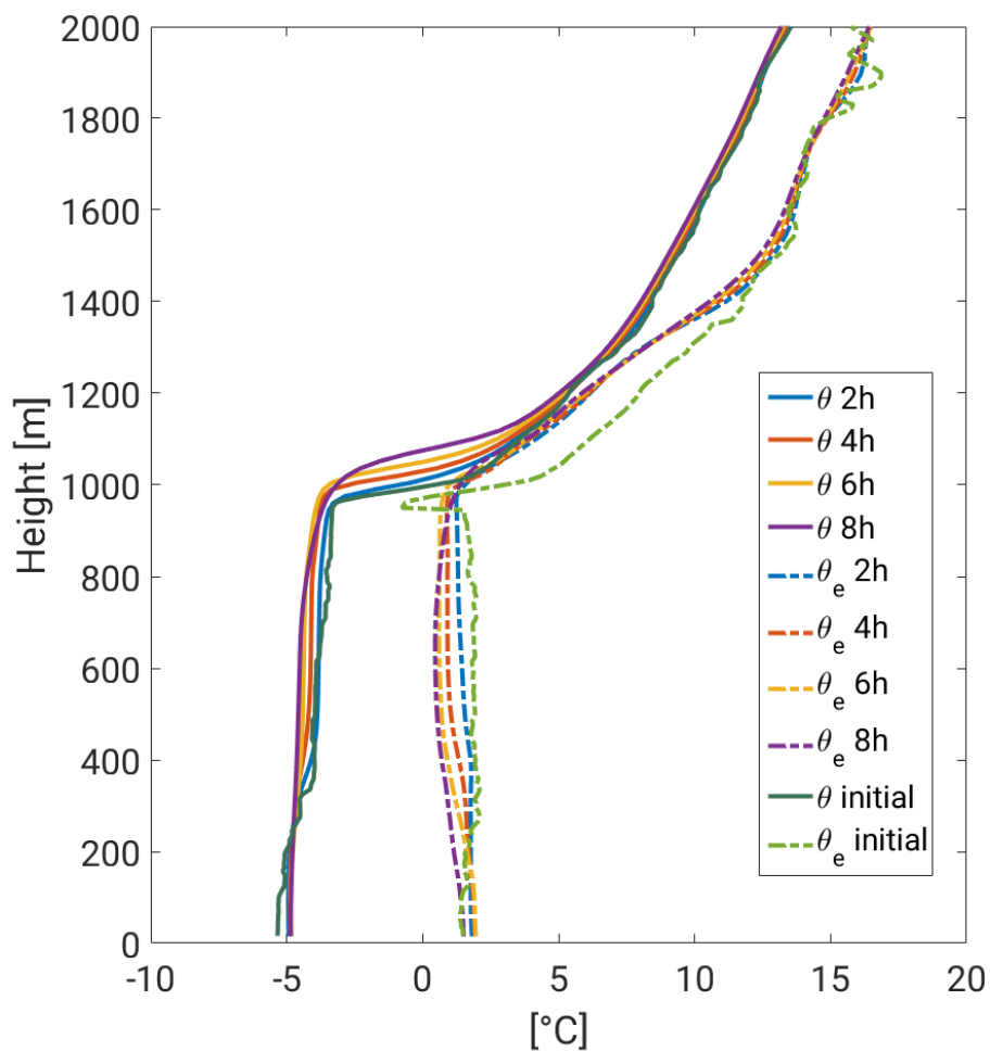
Figure 7. \theta (left) and \theta_e (right) profiles of the initial conditions (dark green and green) and after 2 h (blue), 4 h (orange), 6 h (yellow) and 8 h (purple) after the start of the SensMoist simulation with a RH of 10 %.
