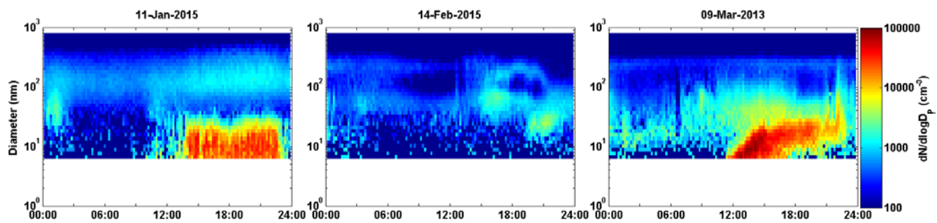
465 Figure 3. Examples of the time evolution of the aerosol size distribution in Puijo for (a) an undefined day characterized by a burst in the number concentrations of the small particles which doesn't have the characteristics of a typical NPF event day (b) a typical undefined day, and (c) a clear NPF event day.
