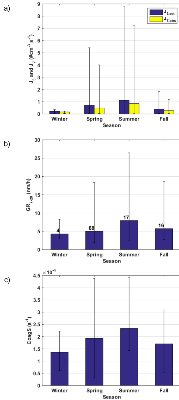
480 Figure 5. Seasonal mean values of different parameters for NPF days at Puijo: a) estimated formation rates of 3-nm particles ( J_{3,est} ) and observed formation rates of 7-nm particles ( J_{7,obs} ). b) growth rate of the particles within size range 7-20 nm c) coagulation sink ( CoagS ) of 7-nm particles. The height of the bars shows the mean values of data points (i.e. mean values
