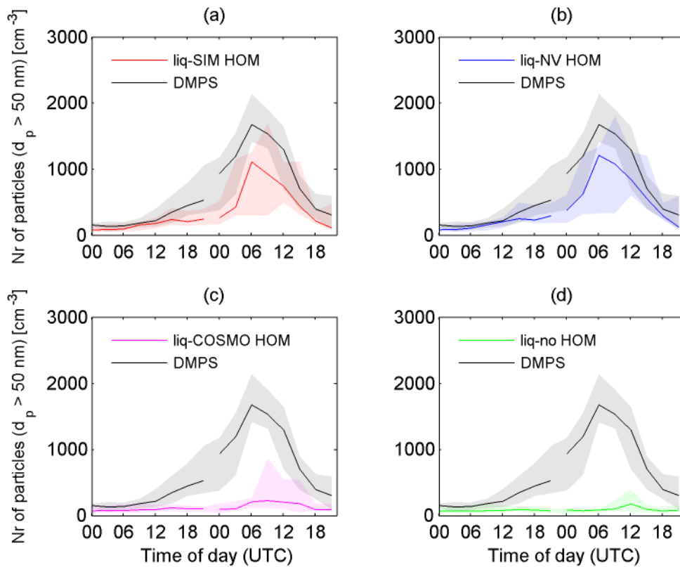
5 Figure 5. Median number of particles above 50 nm of all chosen NPF-events at Pallas (from midnight at the day of the event to the evening the day after the start of the event) together with the 25 and 75 percentiles (shaded areas). The black lines are the median DMPS-data from Pallas. The colored lines in (a)-(c) are the modeled median number of particles above 50 nm, using different methods to estimate the vapor pressures of the HOMs (see table 1). In (d), HOMs are excluded.
