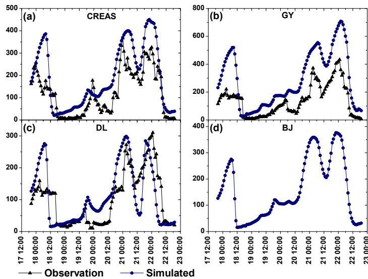
Figure 8. (a)-(c): Comparisons of the observed (black solid triangles) and simulated (blue dot-line) hourly PM_{2.5} concentrations at the CRAES, GY, and DL stations; (d): Hourly variations in the average PM_{2.5} concentrations over Beijing Municipality.
