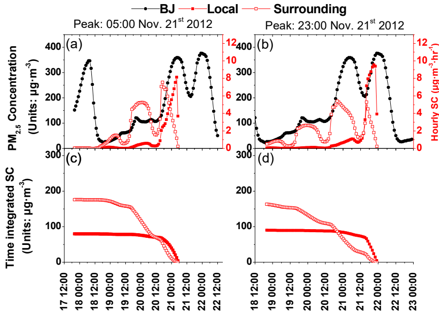
670 Figure 11. Hourly variations of surface PM_{2.5} concentrations in Beijing and sensitivity coefficients of surface PM_{2.5} concentration peaks in Beijing to local and surrounding primary PM_{2.5} sources. The left and right panels correspond to PM_{2.5} concentration peaks at 05:00 LT and at 23:00 LT on the 21st of November 2012, respectively. (a–b) Hourly variations of Beijing PM_{2.5} concentrations (black solid dot-line) and hourly instantaneous sensitivity coefficients to local (red closed squares) and surrounding (red open squares) emission sources. (c–d) The time-integrated sensitivity coefficients to local (red closed squares) and surrounding (red open squares) emission sources. 675
