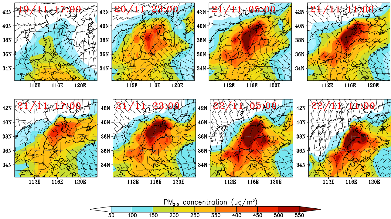
Figure 9. Variations of simulated surface PM 2.5 concentrations and wind field distributions.
