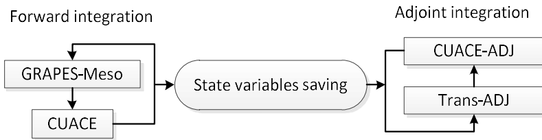
Figure 4. Operational processes of the GRAPES-CUACE aerosol adjoint
