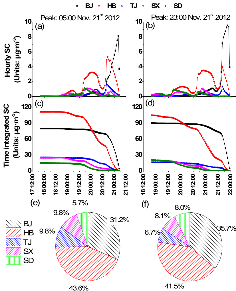
565 Figure 9. Sensitivity coefficients of surface PM_{2.5} concentration peaks in Beijing to primary emission sources from local Beijing and each of the surrounding provinces. The left and right panels correspond to PM_{2.5} concentration peaks at 05:00 LT and at 23:00 LT on 21 November 2012 respectively. (a–b) illustrate hourly instantaneous sensitivity coefficients to emission sources from local Beijing, Hebei province, Tianjin city, Shanxi province and Shandong province. (c–d) show the time-integrated sensitivity coefficients to local and surrounding provincial emission sources. (e–f) are the contribution ratios of emission sources from each 570 surrounding province to PM_{2.5} concentration peaks.
