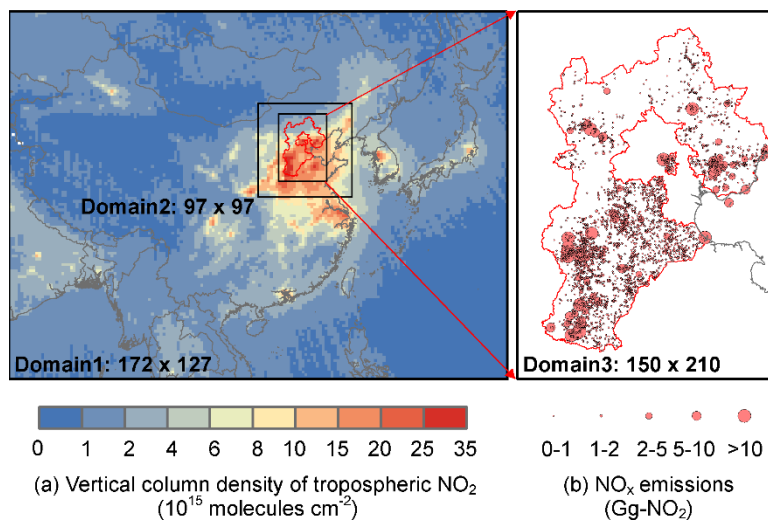
435 Figure 1. Triple-nested domains of the CMAQ simulation: (a) spatial extent of triple-nested domains with OMI-derived NO 2 column densities (Boersma et al., 2011) in background; (b) domain 3 with NO x emissions from point sources in HB-EI inventory.
