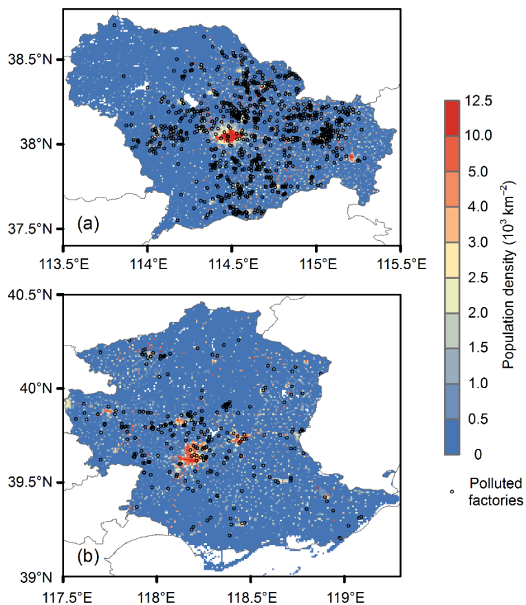
Figure 4. The spatial distributions of polluted industries and population in (a) Shijiazhuang and (b) Tangshan.
