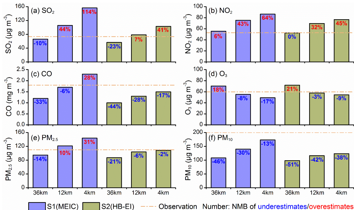
Figure 6. Evaluations against in situ measurements for atmospheric modeling using MEIC and HB-EI inventories at 36 km, 12 km and 4 km. The air pollutants used for evaluation include (a) SO 2 , (b) NO 2 , (c) CO, (d) O 3 , (e) PM 2.5 , and (f) PM 10 .
