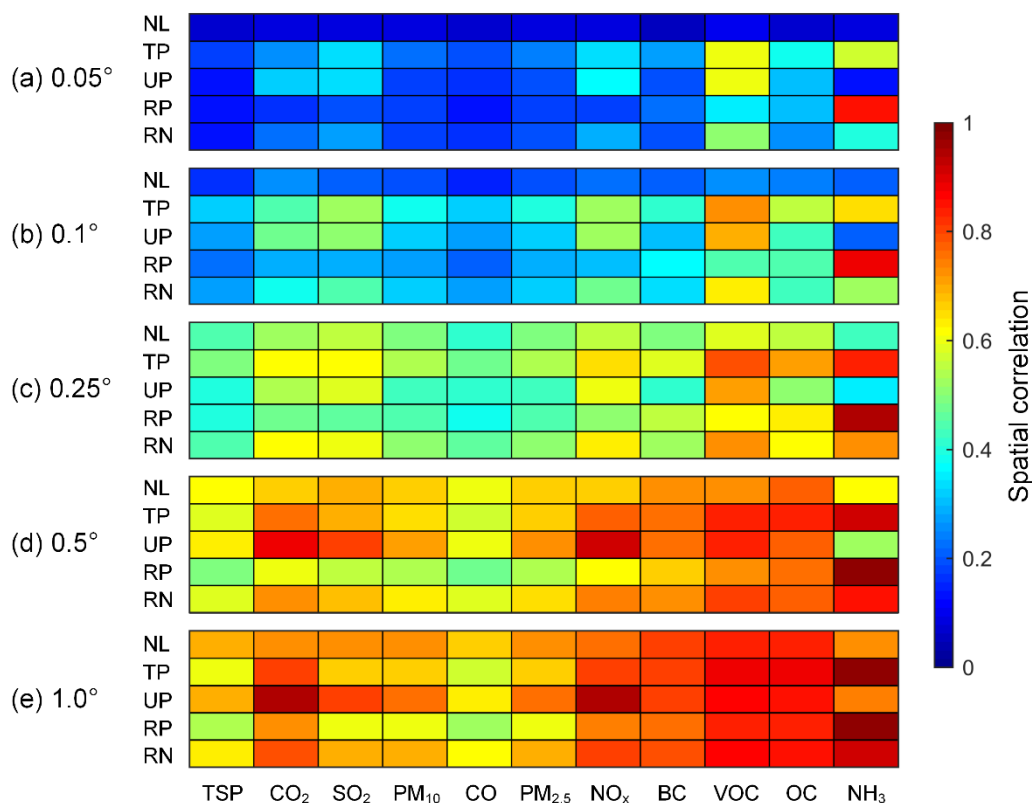
Figure 8. Spatial correlations between gridded emissions of HB-EI and various spatial proxies at the resolutions of (a) 0.05 °, (b) 0.1 °, (c) 0.25 °, (d) 0.5 ° and (e) 1.0 °. The pollutants are sorted according to descending contribution of point-source emissions from left to right. NL: nighttime light ( http://ngdc.noaa.gov/eog/dmsp/downloadV4composites.html ); TP: total population; UP: urban population; RP: rural population (population data (Oak Ridge National Laboratory, 2013) with urban/rural extents (Schneider et al., 2009); RN: road network (Zheng et al, 2014).
