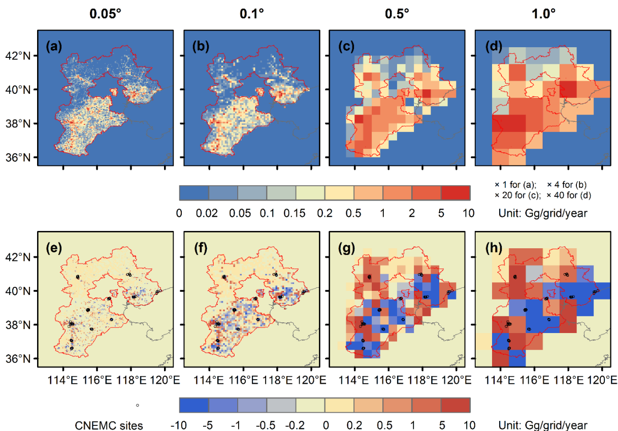
440 Figure 3. Comparison of the spatial distributions of gridded emissions from HB-EI and MEIC at multiple resolutions. (a–d) present \text{NO}_x emission distributions in HB-EI, and (e–h) present the differences between the two inventories (MEIC subtracted from HB-EI).
