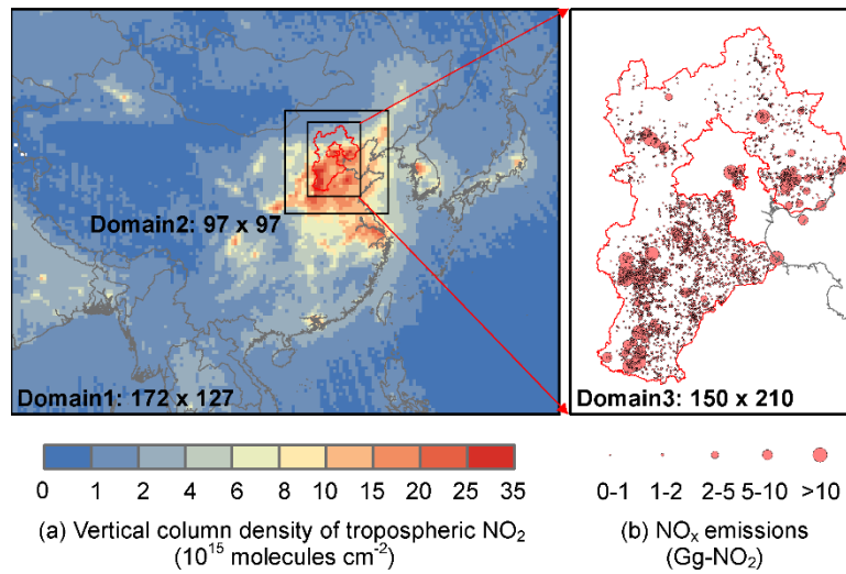
440 Figure 1. Triple-nested domains of the CMAQ simulation: (a) spatial extent of triple-nested domains with OMI-derived NO 2 column densities (Boersma et al., 2011) in background; (b) domain 3 with NO x emissions from point sources in HB-EI inventory.
