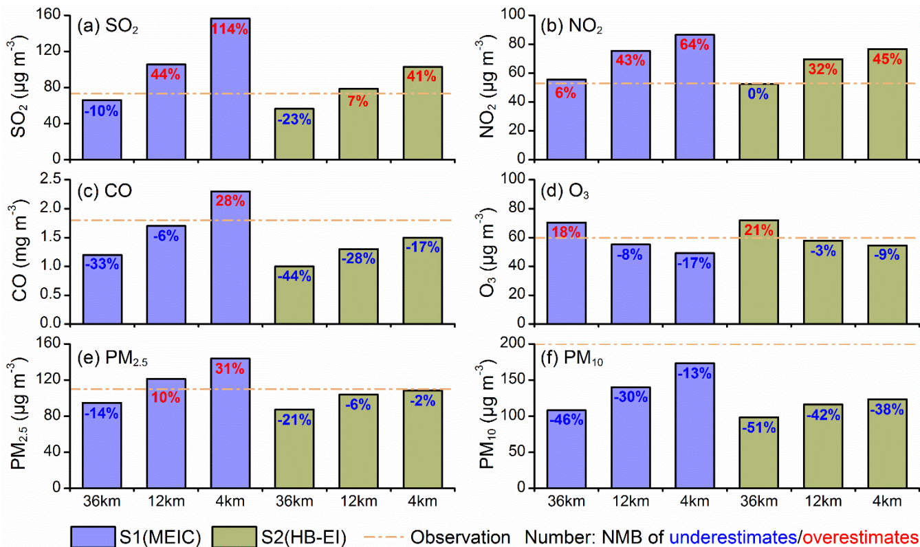
455 Figure 6. Evaluations against in situ measurements for atmospheric modeling using MEIC and HB-EI inventories at 36 km, 12 km and 4 km. The air pollutants used for evaluation include (a) SO 2 , (b) NO 2 , (c) CO, (d) O 3 , (e) PM 2.5 , and (f) PM 10 .
