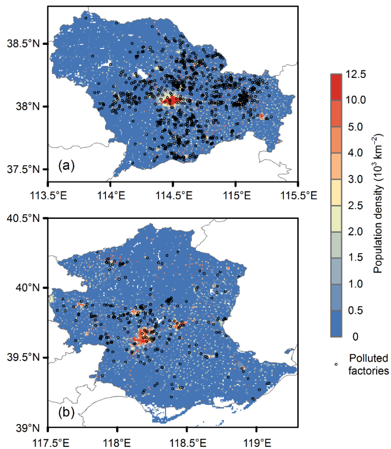
450 Figure 4. The spatial distributions of polluted industries and population in (a) Shijiazhuang and (b) Tangshan.
