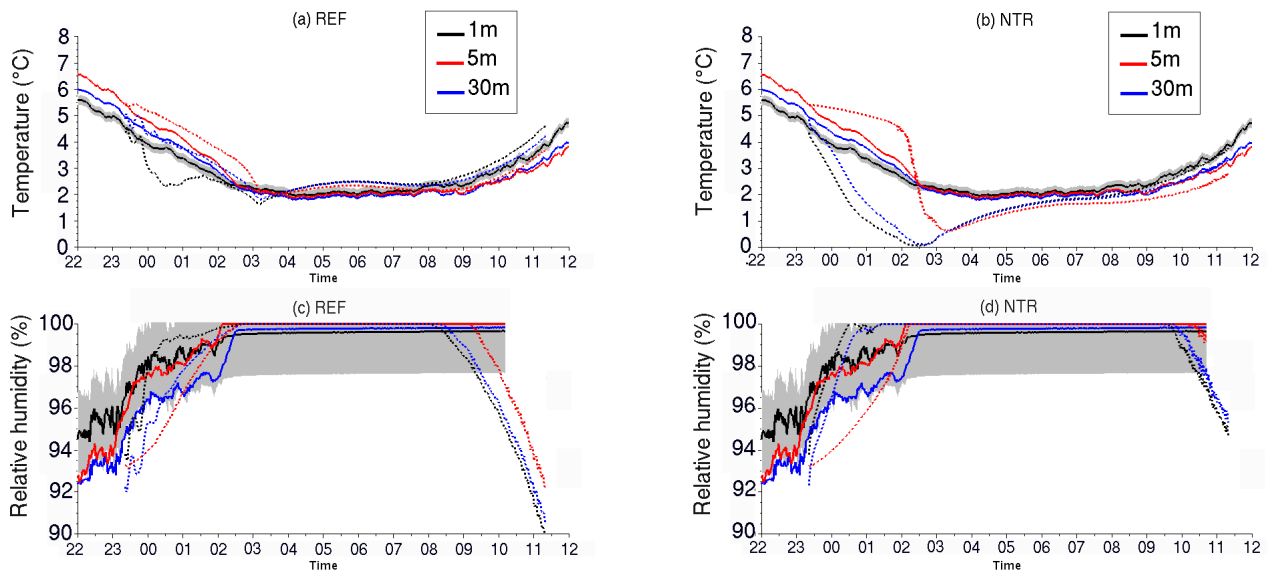
Figure 2. Observed (solid lines) and simulated (dashed lines) temporal evolution of temperature (a and b) and relative humidity (c and d) at 1m, 5m and 30m for the REF (a and c) and the NTR (without trees) (b and d) simulations. Simulated fields are averaged over the horizontal area located downstream of the tree barrier (blue contour area of Fig. 1b). Grey shaded areas represent the error bar for the observational curves.
