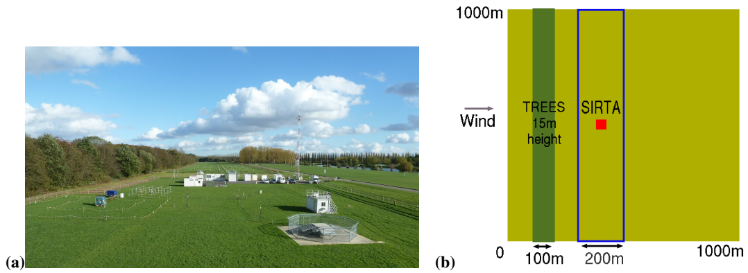
Figure 1. View of the measurement site (a) and modelling domain (b) with the tree barrier. All the simulated averaged results are presented in the blue contour area.
