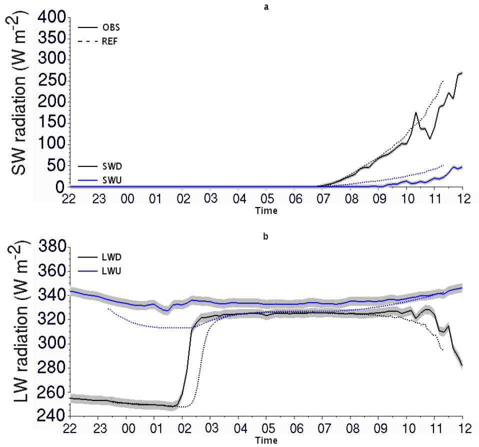
Figure 4. Observed (solid lines) and simulated (dotted lines, with the REF simulation) temporal evolution of downward and upward (at 1m) shortwave (a) and longwave (b) radiation fluxes (in W/m^2 ). Simulated fields are averaged over the horizontal area located downstream of the tree barrier (blue contour area of Fig. 1b). Grey shaded areas represent the error bar for the observational curves.
