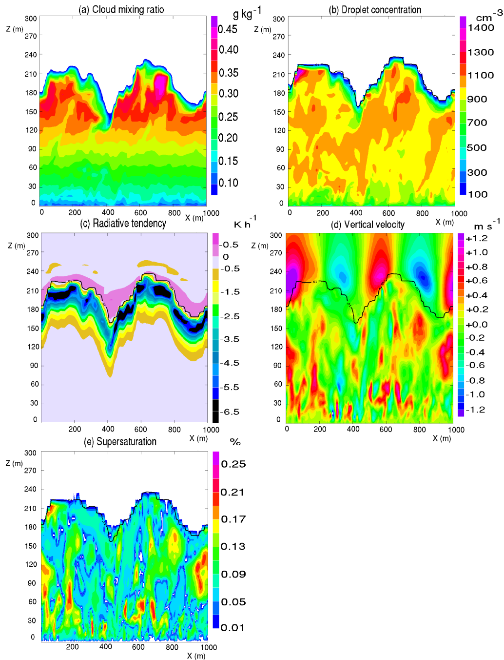
Figure 9. Vertical cross-section at Y=500\text{m} at 0620 UTC for the REF simulation: (a) cloud mixing ratio (in \text{g kg}^{-1} ), (b) droplet concentration (in \text{cm}^{-3} ), (c) radiative tendency (in \text{K h}^{-1} ), (d) vertical velocity (in \text{m s}^{-1} ) and (e) maximum of supersaturation (in %) with the isoline of r_c = 0.01 \text{ g kg}^{-1} superimposed.
