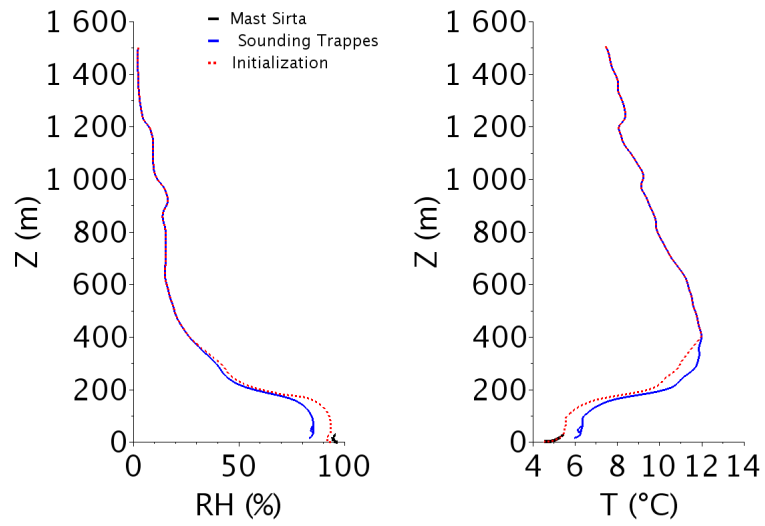
Figure A.1. Relative humidity (in %) and temperature (in C ) vertical profiles at 2320 UTC on 14 November 2011 observed at the Sirta mast (in black) and by the Trappes radiosounding (in blue) and used for the REF initialization.
