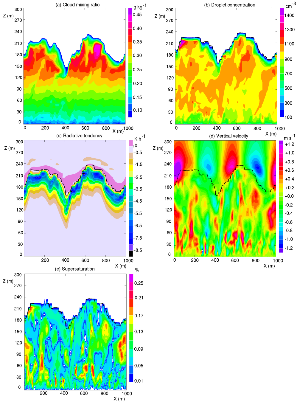
Figure 9. Vertical cross-section at Y=500\text{m} at 0620 UTC for the REF simulation: (a) cloud mixing ratio (in \text{g kg}^{-1} ), (b) droplet concentration (in \text{cm}^{-3} ), (c) radiative tendency (in \text{K h}^{-1} ), (d) vertical velocity (in \text{m s}^{-1} ) and (e) maximum of supersaturation (in %) with the isoline of r_c = 0.01 \text{ g kg}^{-1} superimposed.
