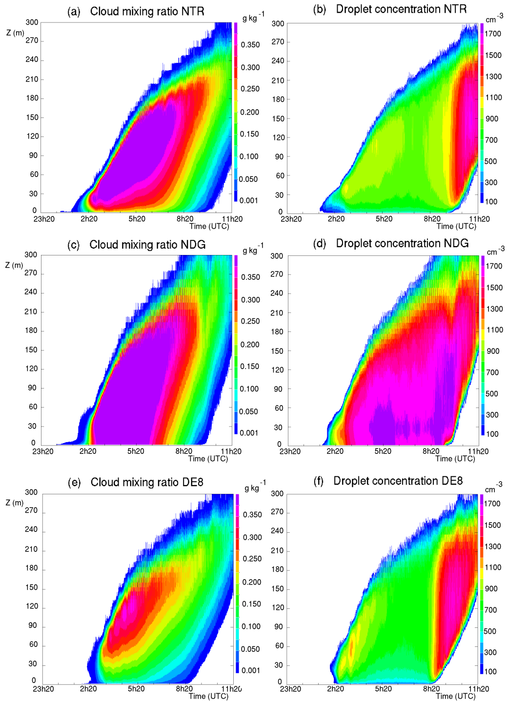
Figure 10. Temporal evolution of simulated vertical profiles of cloud mixing ratio (a, c and e, in g kg -1 ) and droplet concentration (b, d and f, in cm -3 ) for NTR, NDG and DE8 simulations. Fields are averaged over the horizontal area located downstream of the tree barrier (blue contour area of Fig. 1b).
