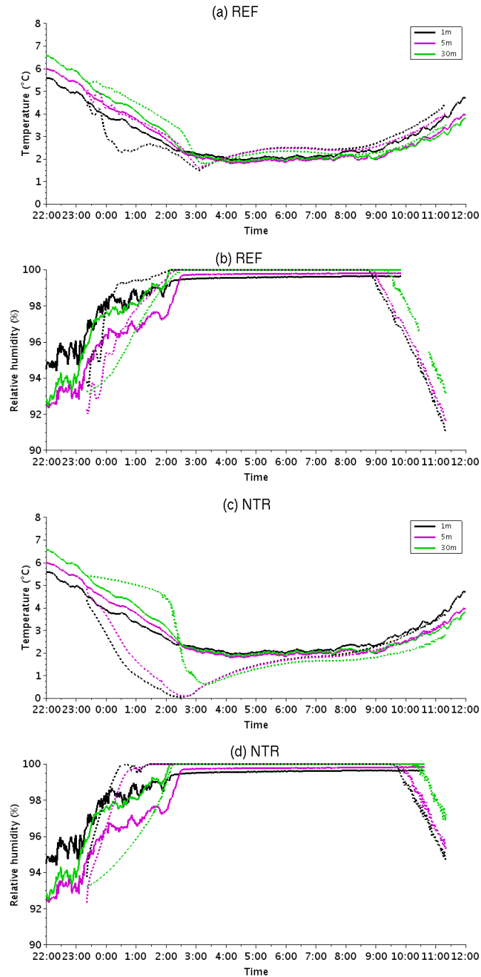
Figure 2. Observed (solid lines) and simulated (dashed lines) temporal evolution of temperature (a and c) and relative humidity (b and d) at 1m, 5m and 30m for the REF (a and b) and the NTR (without trees) (c and d) simulations. Simulated fields are averaged over the horizontal area located downstream of the tree barrier (blue contour area of Fig. 1b).
