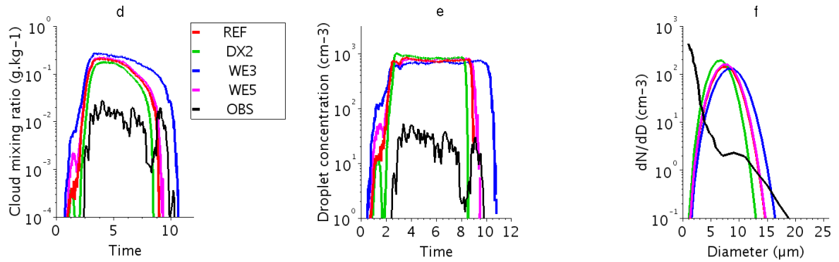
Figure 13. Time series of cloud mixing ratio (a and d, in \text{g.kg}^{-1} ), droplet concentration (b and e, in \text{cm}^{-3} ), and droplet size distribution (c and f, in \text{cm}^{-3} ) at 0520 UTC and 3 m agl observed (in black), and simulated (in colour). Simulated fields are averaged over the horizontal area located downstream of the tree barrier (blue contour area of Fig. 1b).
