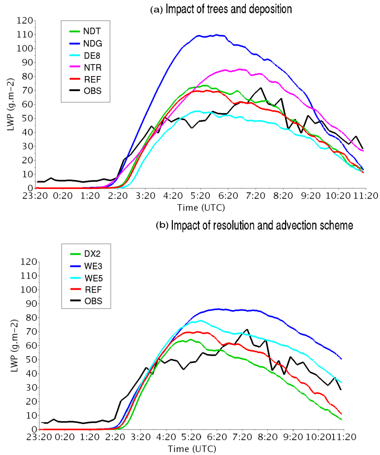
Figure 15. Time series of LWP (in \text{g m}^{-2} ) observed (in black), and simulated (in colour) for the different simulations. Simulated fields are averaged over the horizontal area located downstream of the tree barrier (blue contour area of Fig. 1b).
