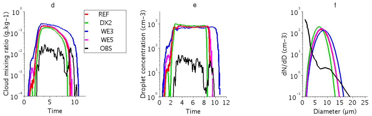
Figure 13. Time series of cloud mixing ratio (a and d, in g.kg -1 ), droplet concentration (b and e, in cm -3 ), and droplet size distribution (c and f, in cm -3 ) at 0520 UTC and 3 m agl observed (in black), and simulated (in colour). Simulated fields are averaged over the horizontal area located downstream of the tree barrier (blue contour area of Fig. 1b).
