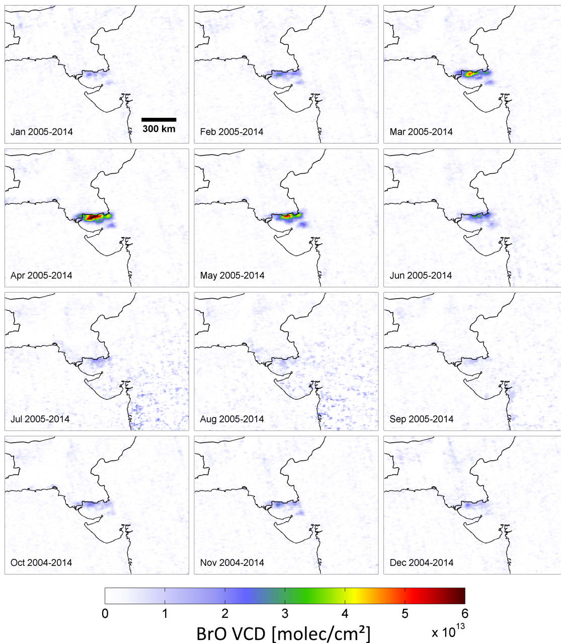
Figure 3. Seasonal variation of monthly mean BrO VCDs with CF < 30% over the Rann of Kutch as seen by OMI during 2004-2014. While maximum VCDs are clearly detected in April/May for the Great and Little Rann, only small enhancements can be seen during wintertime. Results during the monsoon season (July-September) include less measurements due to increased cloud frequency leading to a higher noise level, especially in the south-eastern part of the shown region. Please note that OMI data are only available since October 2004, i.e. no data for January-September 2004 are included.
