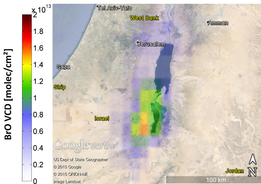
Figure 10. Averaged BrO VCD over the Dead Sea as seen by OMI during summer months 2005-2014 (April–October). A clear enhancement of the BrO VCDs can be seen over the southern part of the Dead Sea, confirming former ground-based observations by (Hebestreit et al., 1999), (Matveev et al., 2001) and (Tas et al., 2005).
