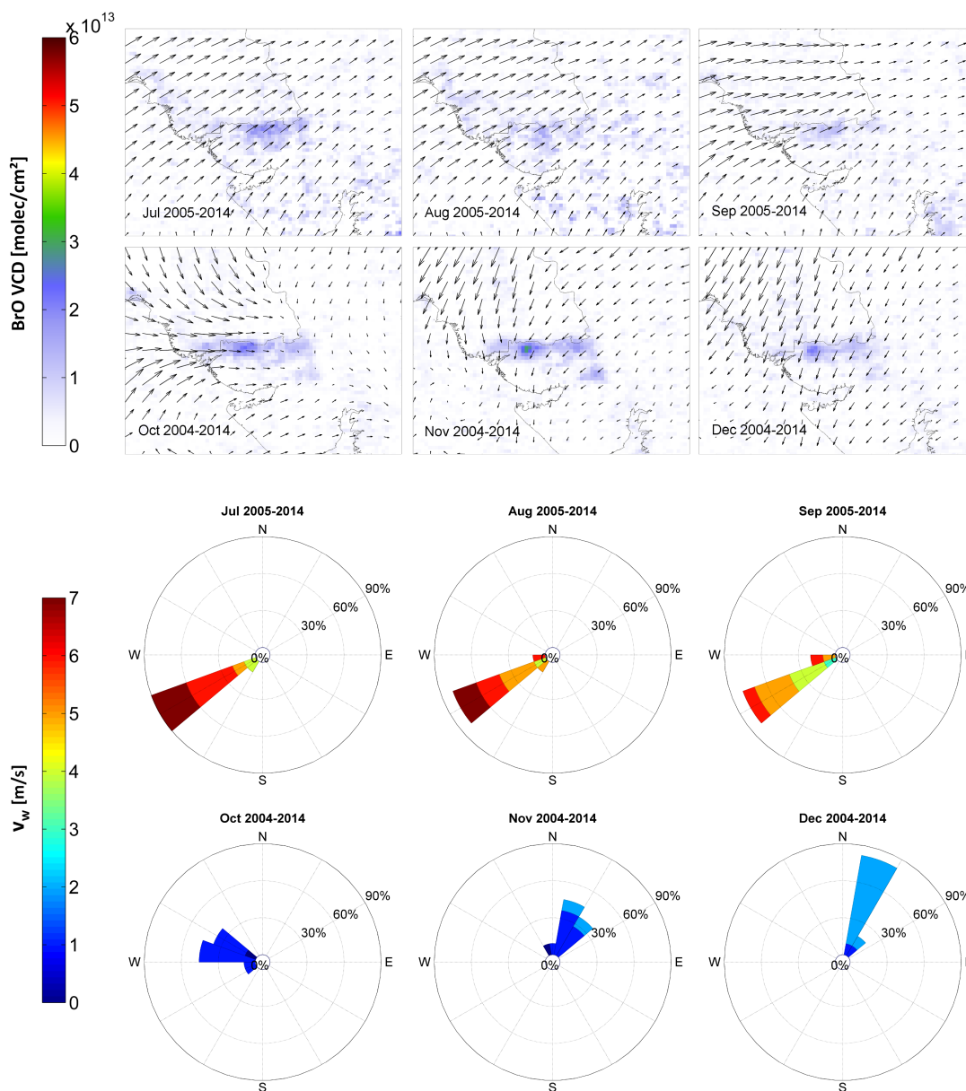
Figure 8. Same as in Figure 7, but for July to December 2004–2014. The area is mainly affected by strong southwestern winds during monsoon months (>7 m/s). After the monsoon, the wind speed rapidly drops ( \approx 2 m/s) and the wind direction changes from west (October) to northeast during wintertime.
