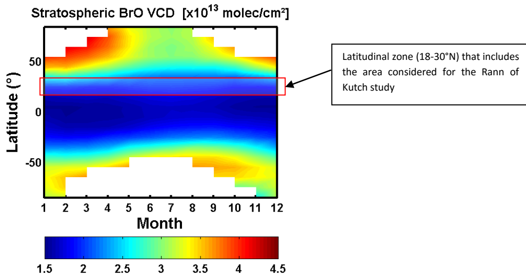
Figure Z2: Monthly zonal averaged stratospheric BrO VCD during the time of the GOME overpass and based on the BASCOE climatology (adapted version of Figure 13 in Theys et al., 2009). The typical stratospheric BrO VCD within the latitudinal band that was considered within our study (18-30°N; indicated by the red rectangle) is about 2.5 \times 10^{13} molec/cm 2 and shows no significant annual variation.
