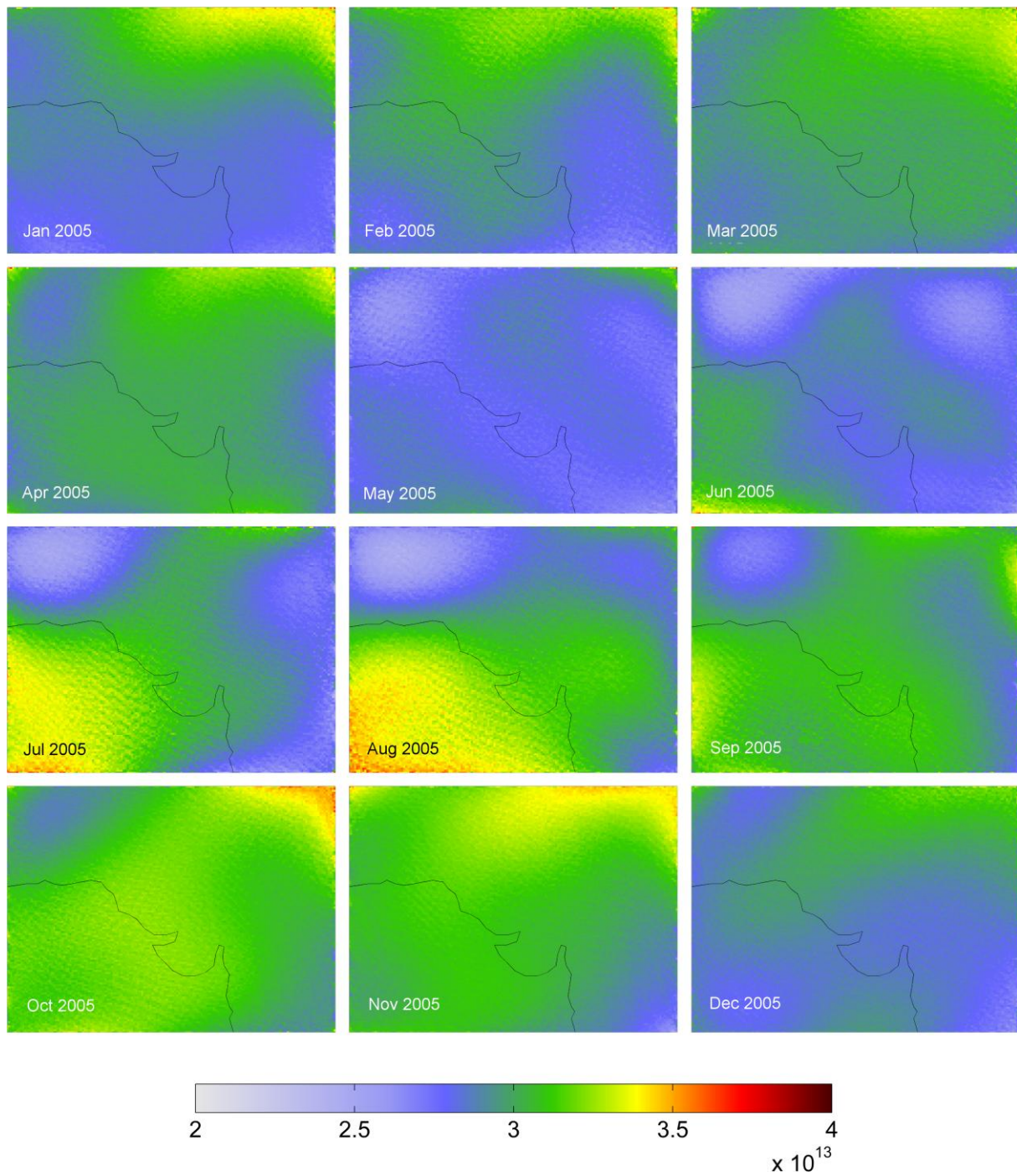
Figure Z1: Monthly mean estimation of the stratospheric BrO VCD during 2005 as a result from the 2D spatial polynomial approach. The stratospheric BrO variation takes place at much larger spatial scales compared to the variations of the tropospheric BrO enhancement observed over the Rann of Kutch (please compare to Figure 7 in the Supplementary Material).
