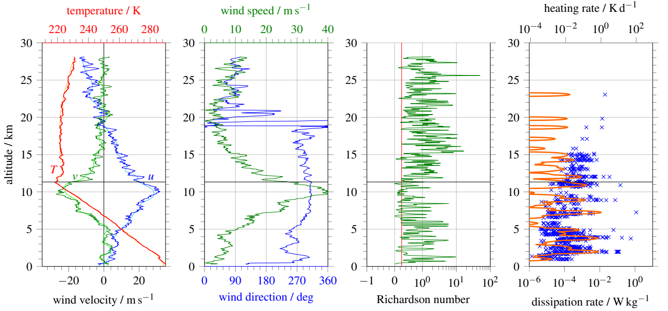
Figure 5. Same as Figure 1, but for the flight from K hlungsborn at 11/12 Jul 2015. The dissipation profile excludes the lowermost 550 m due to disturbances from the launch procedure (dereeling of the payload suspension).
