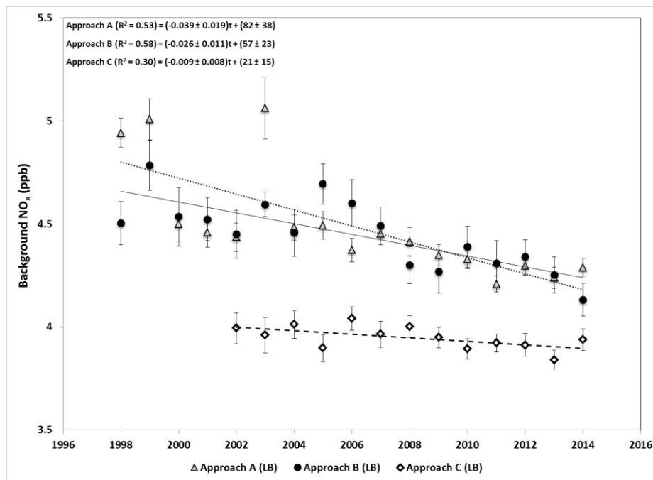
Figure S22: Temporal trends in lower bound of background \text{NO}_x
