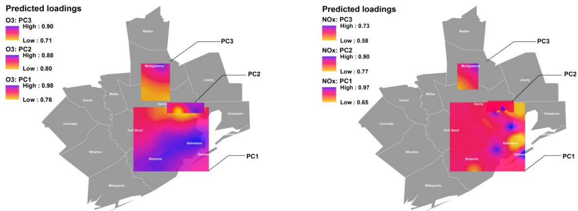
Figure 2: Spatial interpolation of normalized squared loadings from the highly correlated sites with the first three components in terms of O 3 (left) and NO x (right). Range is from 0 to 1.
