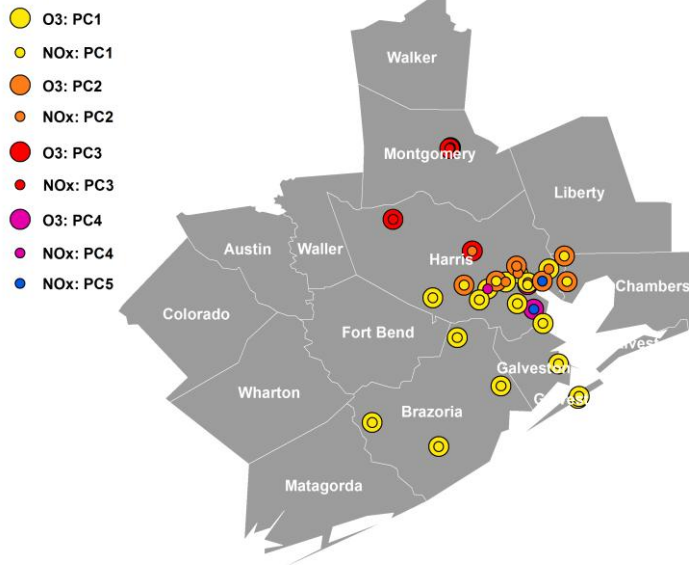
Figure 1: Distinct clustering of principal components. The cluster in yellow is PC1-O 3 and PC1-NO x . The cluster in orange is PC2-O 3 and PC2-NO x , and so on. Smaller circles represent NO x clusters.
