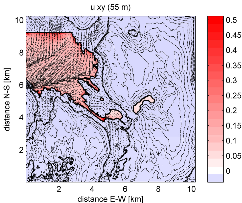
5 Figure 4: The 55 m wind field from case 3 together with H_s [ K m s^{-1} ]. The figure shows the mean fields over the last 15 min of the 12 h simulation time. Wind vectors point into the flow direction. The wind-vector in the upper right corner indicates the scale of the wind vector length. It shows a wind speed of 3 m s^{-1} . The 55 m topographic line is indicated by the thick black dashed line. The water-land interface is shown by the thick solid line.
