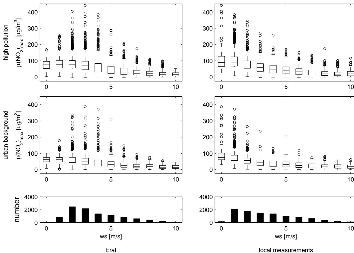
Figure 1: \text{NO}_2 concentrations at the two air quality reference stations in Bergen against the 10 m wind speeds (ws) over the Bergen valley from Eral and from local measurements inside the valley between 2003 and 2013. Eral data are available every 3 hours. \text{NO}_2 concentrations and the local measured winds represent hourly means. The \text{NO}_2 concentrations are the 3-hourly maxima and the local wind data are the 3-hourly means around the three-hour time steps. Only wintertime data (Nov-Feb) are included. The edges of the boxes are the 25th and 75th percentiles. Lines inside the boxes show the median. The maximum whiskers length is 1.5 times the distance between the 25th and 75th percentiles or the maxima and minima of the data. Outliers with higher or lower concentration values than that are shown as circles. The lower panels show the number of simultaneously valid wind and pollution measurements within each wind speed bin.
