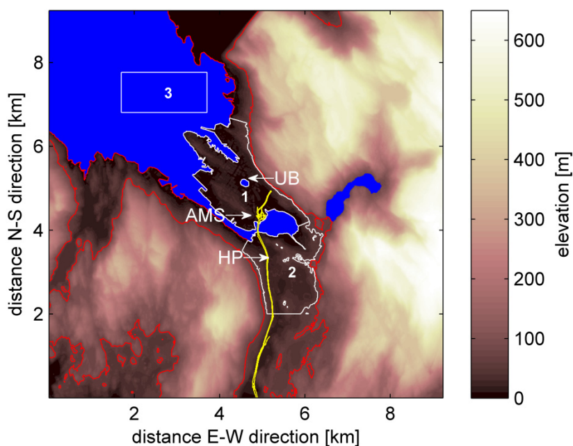
5 Figure 2: Topographic map of the computational domain for the model simulations. Blue colour indicates water. The white contour line marks the areas 1 and 2 selected for averaging of the wind and passive tracer concentration. The red contour line marks the area of passive tracer emissions in most of the experiments. Both lines are overlapping along the coast. The yellow line represents the main street along the valley, eventually disappearing into a tunnel after having crossed the valley. White arrows indicate the positions of the wind measurements (AMS), and the UB and HP reference stations for \text{NO}_2 air pollution. The area for averaging of the 2 m temperature over the fjord in Table 1 is marked as area 3; averaging of the 2 m temperature over the city centre is done separately over areas 1 and 2.
