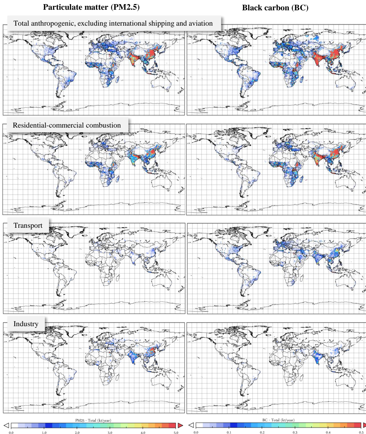
Figure 5. Global distribution of emissions of PM 2.5 (left) and BC (right) in 2010 [Gg year -1 per grid] from land-based sources, ECLIPSE V5a; the scale is the same across sectors but there is a factor ten between PM 2.5 and BC
