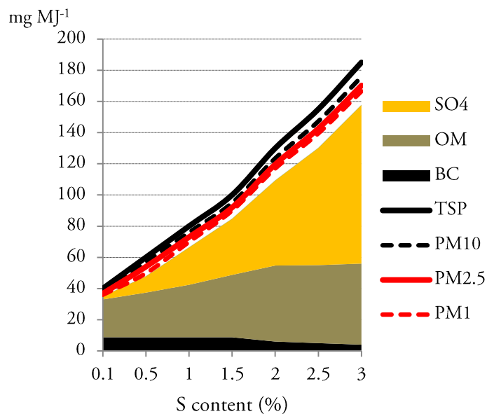
Figure 2. Particulate matter emission factors for shipping used in the GAINS model
