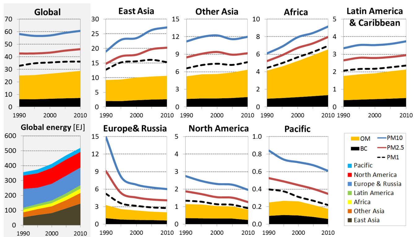
Figure 3. Global and regional emissions of PM species [Tg] and global energy consumption [EJ] in the period 1990-2010, ECLIPSE V5a.
