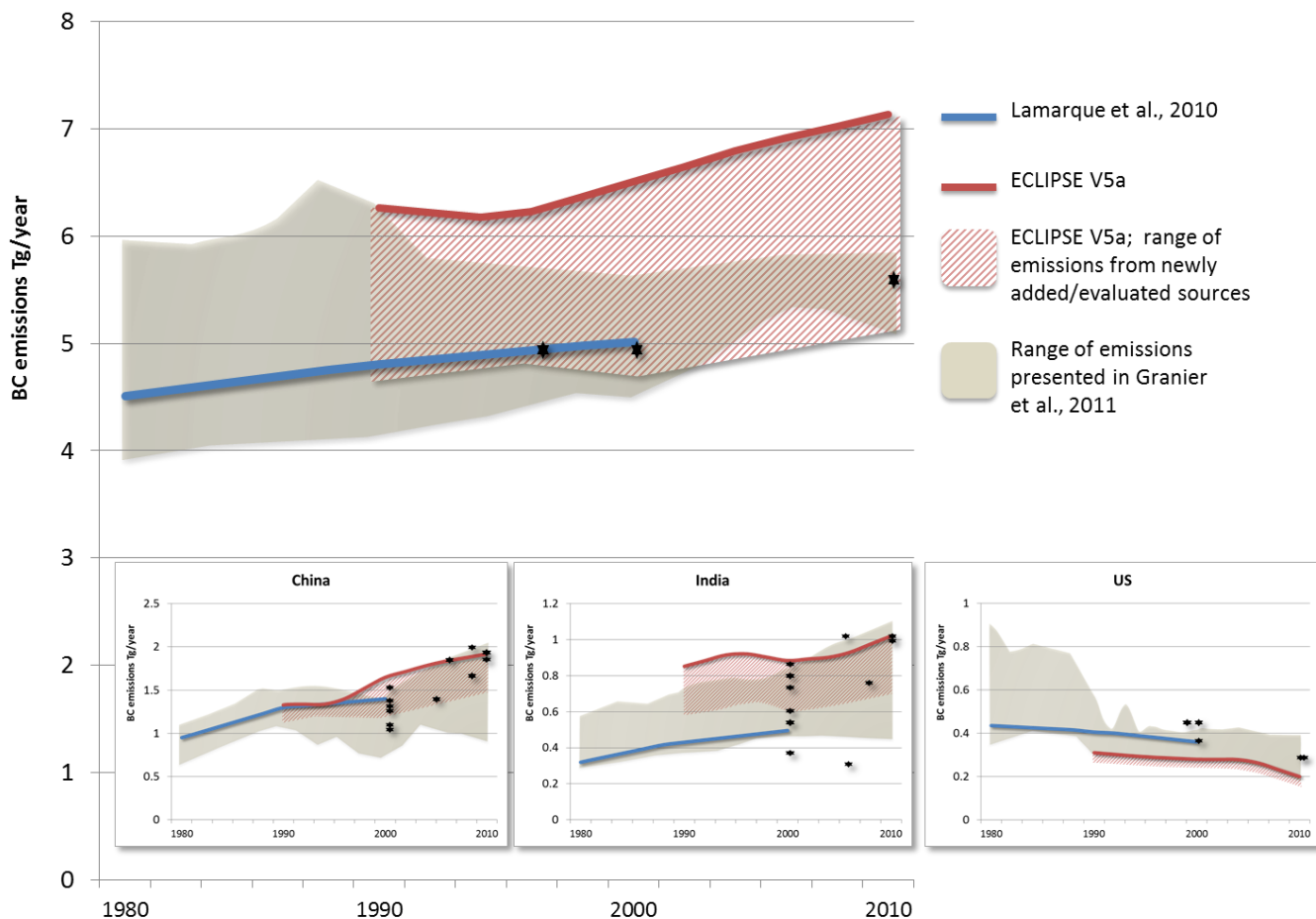
Figure 7. Comparison of black carbon emission in this work (ECLIPSE V5a) with Lamarque et al. (2010) and Granier et al. (2011)
