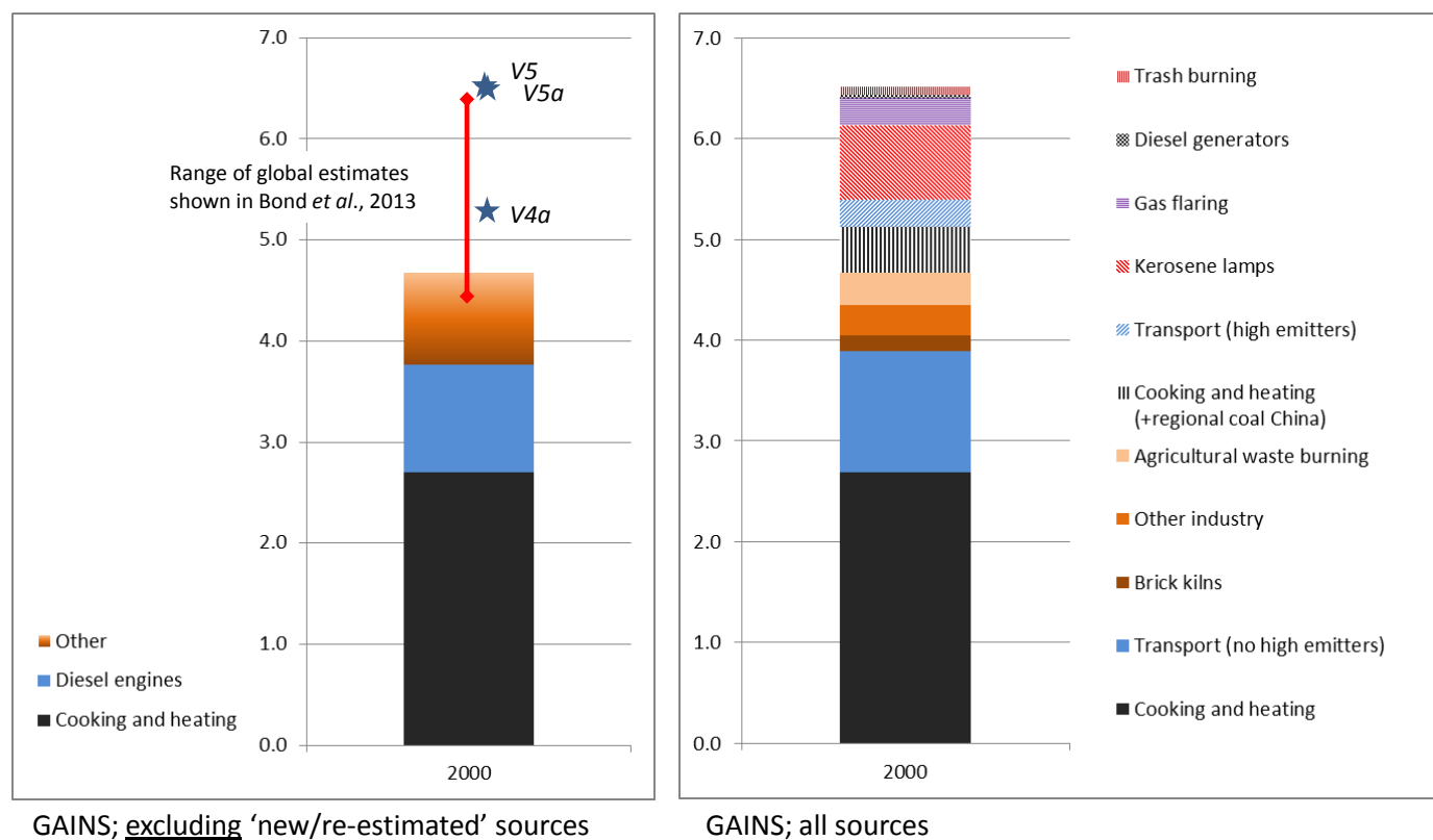
5 Figure 6. Source-sector distribution of global anthropogenic emission of BC estimated with the GAINS model (ECLIPSE V5a) for the year 2000, Tg year -1
