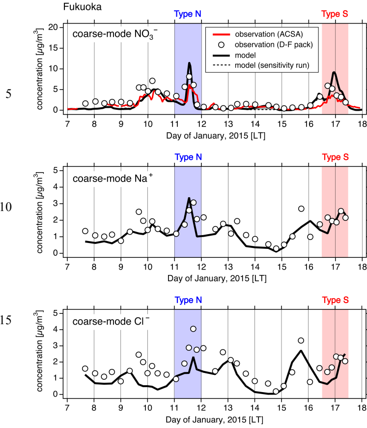
5 10 15 20 Figure 7: Temporal variation of coarse-mode \text{NO}_3^- , \text{Na}^+ , and \text{Cl}^- at Fukuoka during January 7-17, 2015. Blue and red shading show the type N and S patterns focused on in this study. Red lines indicate coarse-mode \text{NO}_3^- observations by ACSA and open circles indicate D-F pack observation. Black lines indicate the base case simulation and dotted black lines indicate the sensitivity simulation in which the anthropogenic emissions from Japan were switched off; the differences between these results shown in gray represent local contributions.
