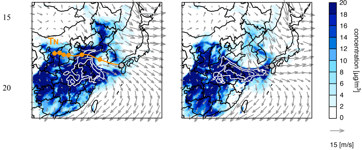
Figure 9: Simulated spatial distribution for (a) \text{SO}_4^{2-} and (b) \text{NO}_3^- during type N pattern. Contours shown by white lines for \text{NO}_3^- represent 40 and 60 \mu\text{g}/\text{m}^3 . The 72 h HYSPLIT backward trajectory from Fukuoka is overlaid with orange lines with circles at 12 h intervals. (Left) 21:00 LT, January 10, 2015, when the air mass left China, and (right) 15:00 LT, January 11, 2015, when the air mass reached Fukuoka.
