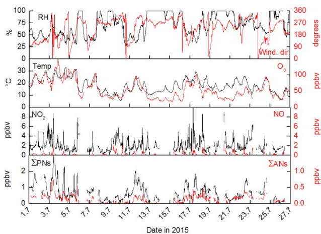
Fig. 2. NOTOMO 2015: Time-series of relative humidity (RH), wind direction, temperature and the mixing ratios of O 3 , NO 2 , NO, ΣPNs, and ΣANs. The NO mixing ratios were calculated assuming photo-stationary state as described in the text.
