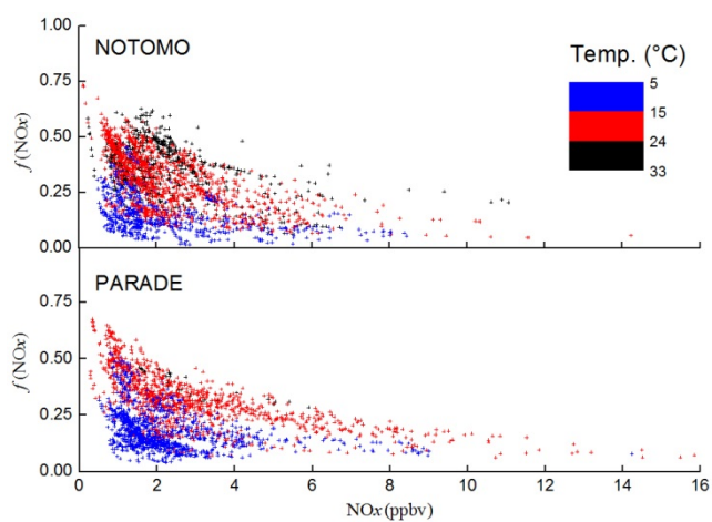
Fig. 3. The fraction of \text{NO}_x sequestered as organic nitrates f(\text{NO}_x) = \frac{[\Sigma\text{PNs}] + [\Sigma\text{ANs}]}{([\Sigma\text{PNs}] + [\Sigma\text{ANs}] + [\text{NO}_x])} as a function of \text{NO}_x for the NOTOMO and PARADE campaigns, both colour coded for temperature.
