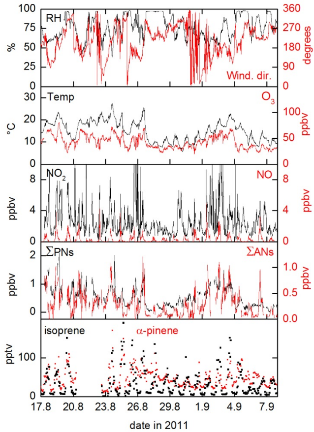
Fig. 1. PARADE 2011: Time-series of relative humidity (RH), wind direction, temperature, and the O 3 , NO 2 , NO, ΣPNs, and ΣANs mixing ratios. The lowest panel shows the mixing ratios of isoprene (black datapoints) and α-pinene (red datapoints).
