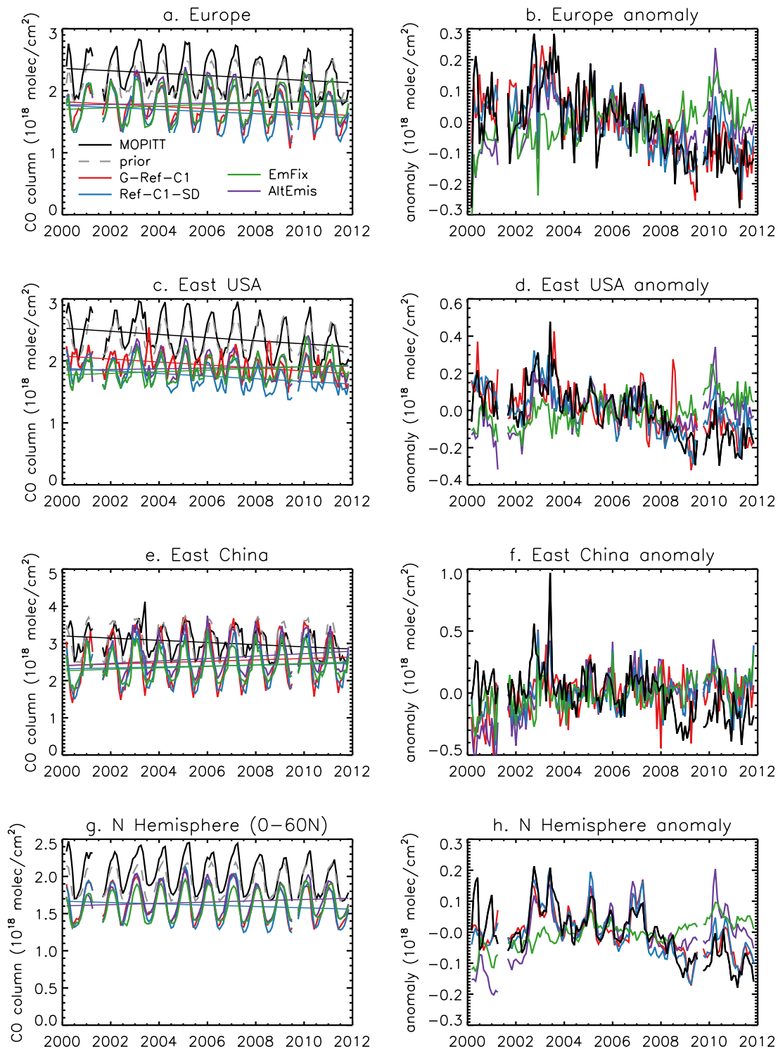
Supplemental Figure S1: The time series (left column) and de-seasonalized monthly anomalies (right column) of the CO column from MOPITT (black), the MOPITT a priori (gray), and simulated by G-Ref-C1 (red), Ref-C1-SD (blue), EmFix (green), and AltEmis (purple) for 2000-2011.
