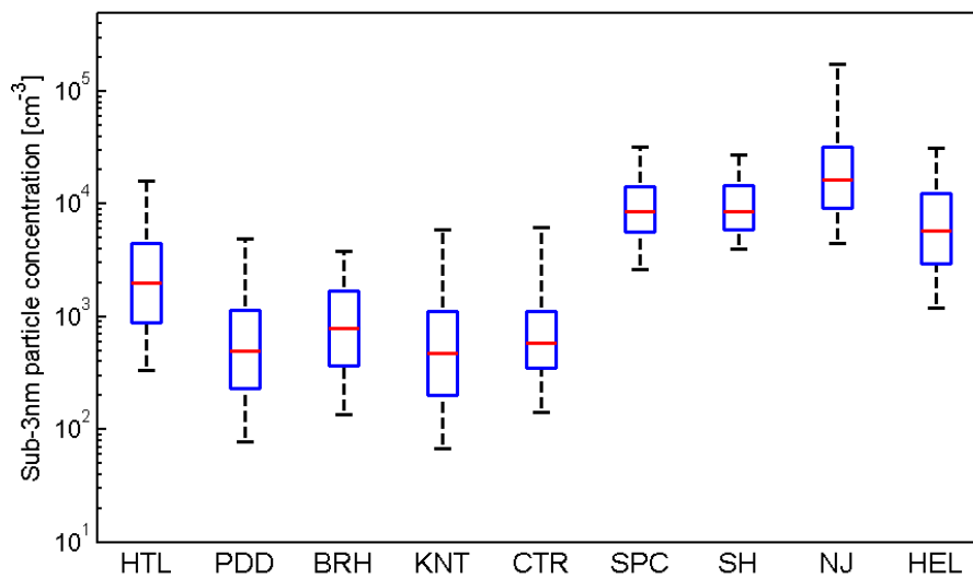
Figure 2. The variation of sub-3 nm particle concentration at different measurements sites. The red lines show the medians, the blue boxes indicate the 25th and 75th percentiles, and the vertical bars show the 5th and 95th percentiles.
