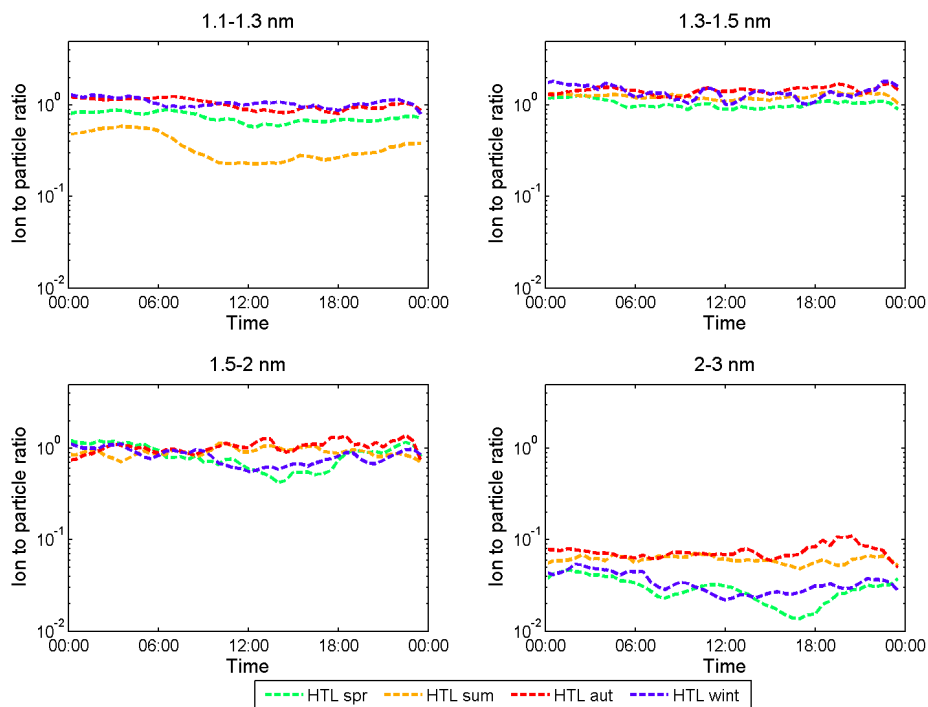
Figure 9. The median diurnal variation of the ratio of ion concentration to the total particle concentration in four size bins (1.1–1.3 nm, 1.3–1.5 nm, 1.5–2 nm, and 2–3 nm) in Hyytiälä in 2011 and 2015–2016. The data are divided into different seasons: spring (spr), summer (sum), autumn (aut), and winter (wint).
