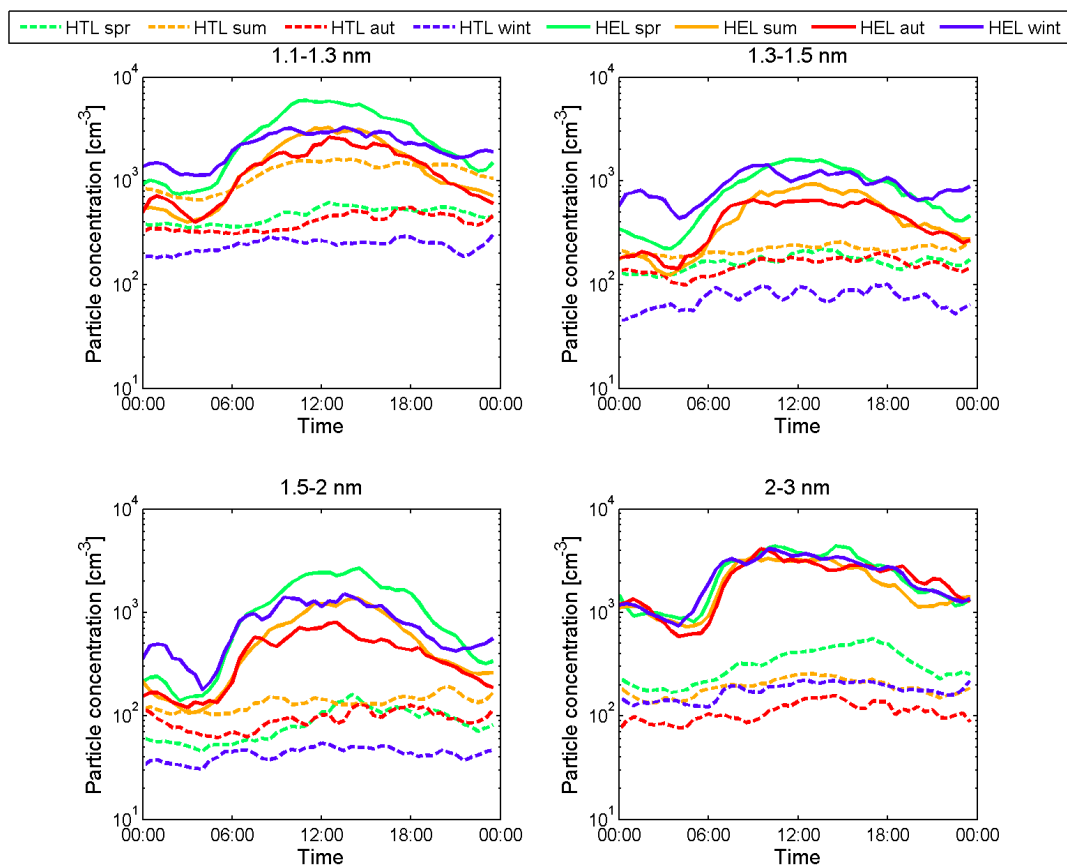
Figure 6. The median diurnal variation of particle concentration in four size bins (1.1–1.3 nm, 1.3–1.5 nm, 1.5–2 nm, and 2–3 nm) in Hyytiälä (HTL; dashed lines) in 2011 and 2015–2016 and in Helsinki (HEL; solid lines) in 2015. The data are divided into different seasons: spring (spr), summer (sum), autumn (aut), and winter (wint).
