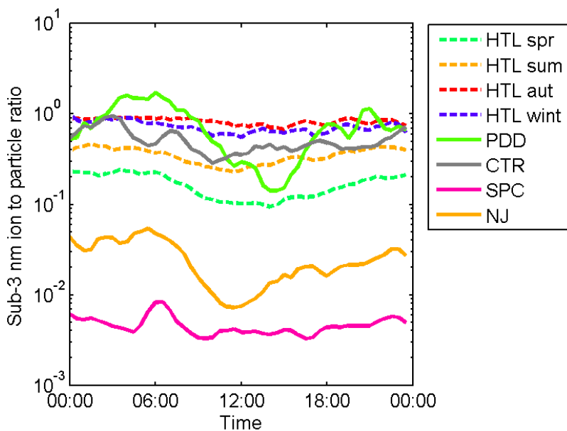
Figure 8. The median diurnal variation of the ratio of sub-3 nm ion concentration to the total particle concentration during different measurement campaigns. The data from Hyytiälä (HTL) are divided into different seasons: spring (spr), summer (sum), autumn (aut), and winter (wint).
