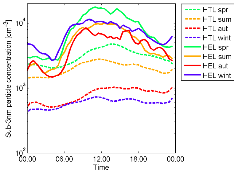
Figure 5. The median diurnal variation of sub-3 nm particle concentration in Hyytiälä (HTL; dashed lines) and in Helsinki (HEL; solid lines) in different seasons: spring (spr), summer (sum), autumn (aut), and winter (wint).
