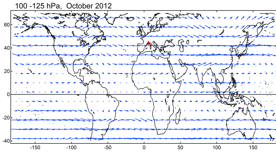
Fig. 2. Figure AR2.1bottom. Wind field at 100-125 mBar level from ERA-Interim reanalysis during October 2012.
