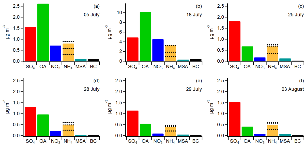
Figure 5 - As in Fig. 4 but for measurements taken inland over the southwest peninsula of the UK.
