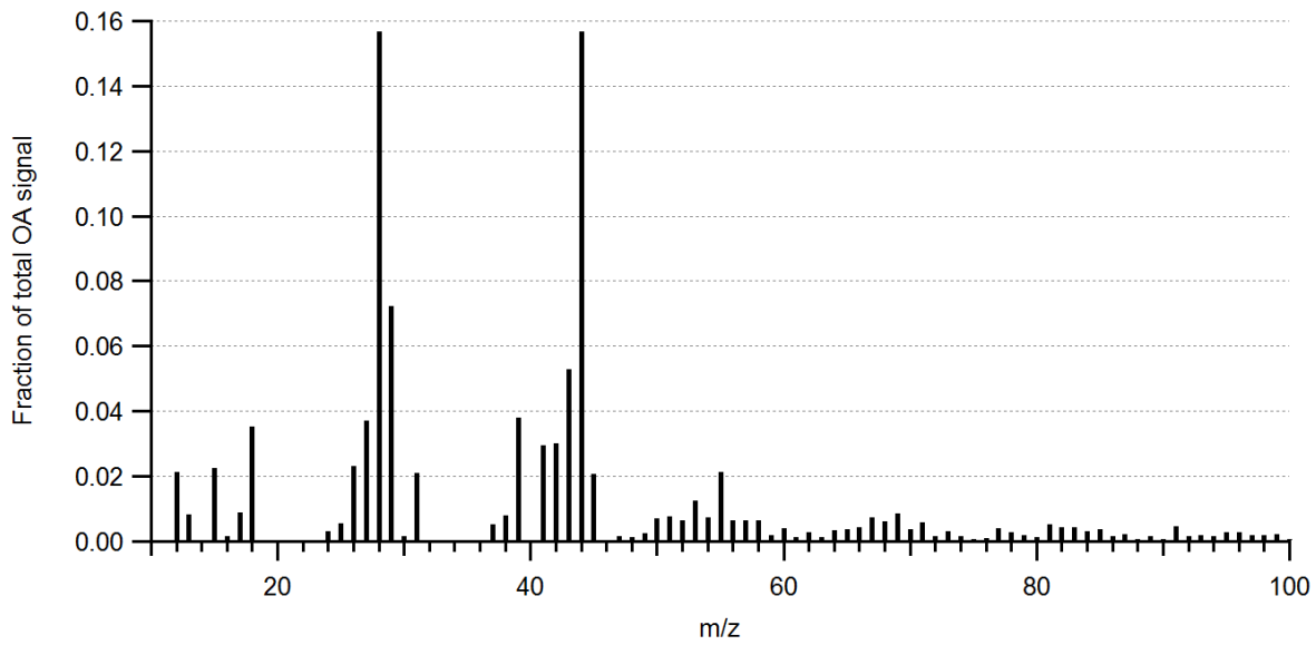
Figure 6 – Normalised mass spectrum of marine OA measured over the NW coast on 05 July.
