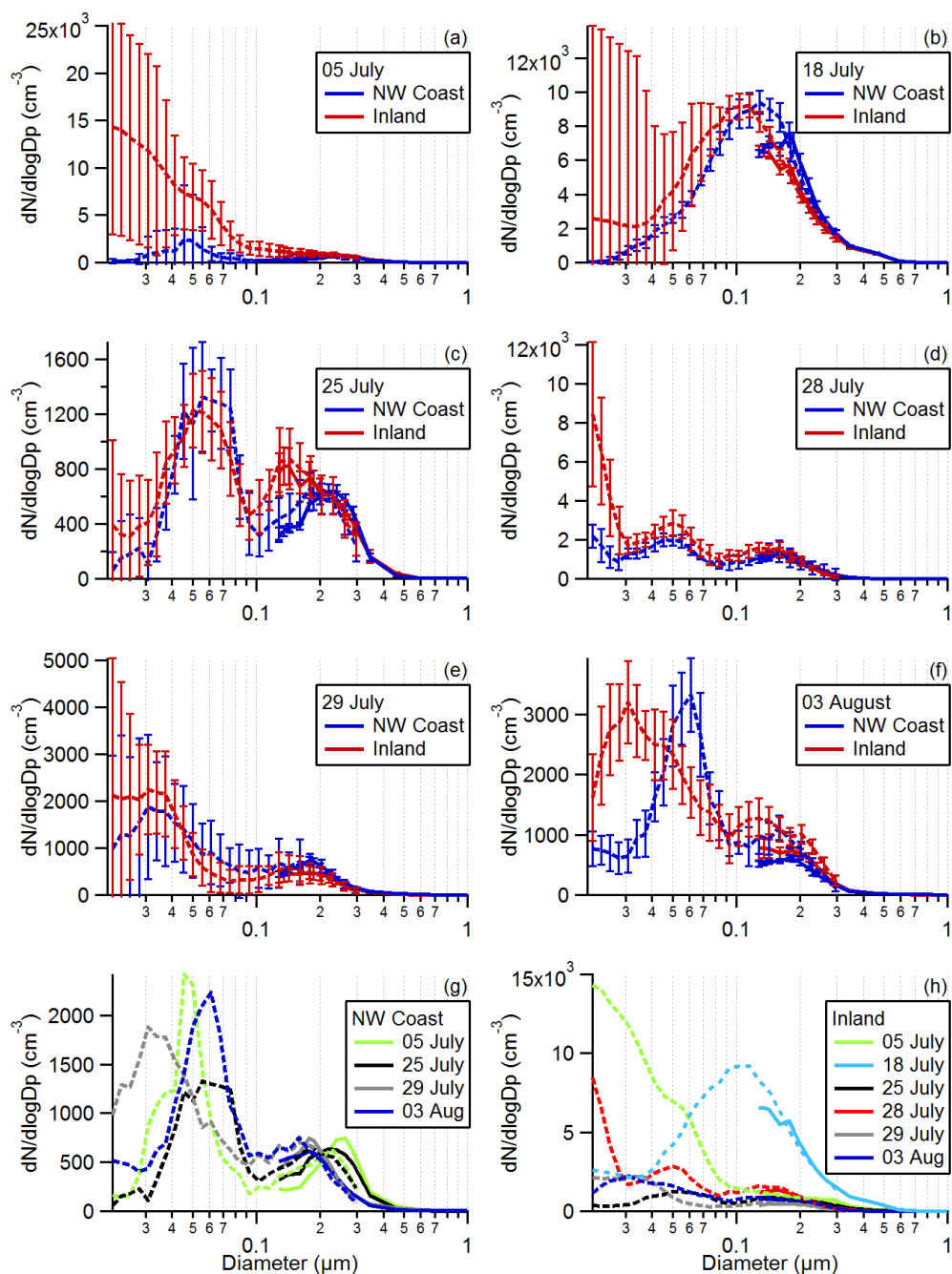
Figure 3 – Submicron aerosol size distributions measured by the SMPS (dashed lines) and PCASP (solid lines) probes aboard the BAe-146. Panels (a) – (f) show the inland and NW coast distributions for each of the case study flights, while panels (g) and (h) show comparisons of all the NW coast and inland distributions respectively. The error bars in panels (a) – (f) show the standard deviations over each measurement period.
