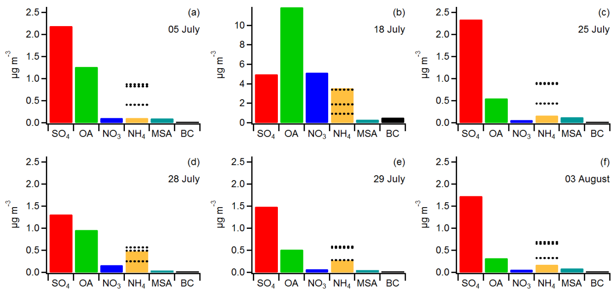
Figure 4 - Aerosol composition measured over the NW coast during the six case study flights. The definitions of each chemical species are given in the text. The lower and middle dashed lines show the concentration of \text{NH}_4 required to neutralise the \text{SO}_4 to ammonium bisulphate and sulphate respectively. The top dashed line shows the concentration of \text{NH}_4 required to fully neutralise all measured inorganic components. The reader should consult the text for discussion of the \text{NO}_3 measurements.
