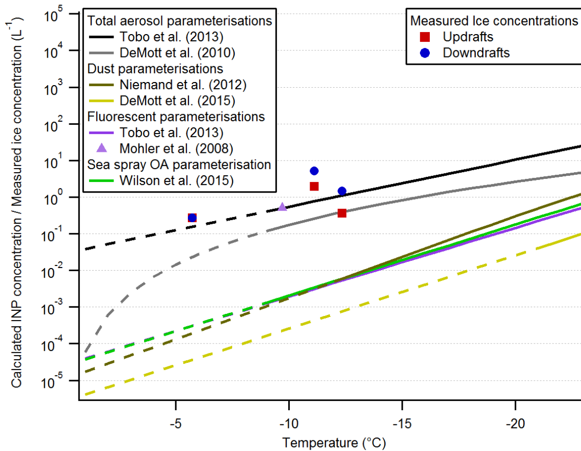
Figure 10 - Comparison of INP calculations using different parameterisations. The solid lines show the temperature ranges in which the INP parameterisations are deemed valid, while the dashed lines are extrapolations. The inland aerosol measurements were used as input for the parameterisations, other for Wilson et al. (2015) where the marine OA concentration was used. The blue and red markers show measured first ice concentrations from Taylor et al. (2015) at different cloud top temperatures.
