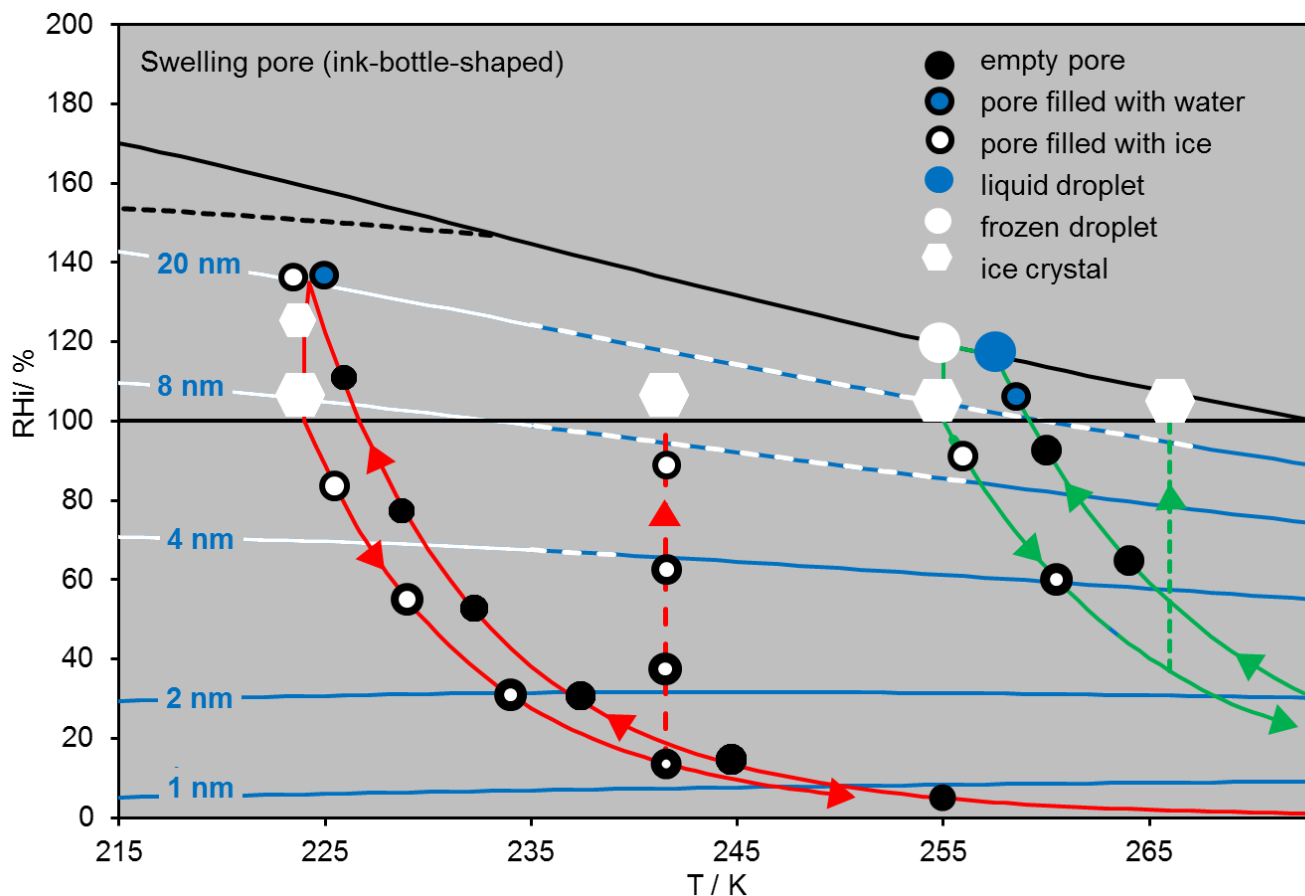
Figure 3. Wet trajectory (green line) and dry trajectory (red line) of a particle with a swelling ink-bottle shaped pore with a cavity of 20 nm and a pore opening that reacts to RH changes. Solid lines: Adiabatic cooling, followed by adiabatic heating; dashed lines: increase of RH at constant temperature. The black horizontal line denotes ice saturation; the black sloped line indicates RH_i/T conditions for water saturation (parameterization of Murphy and Koop, 2005). The black dashed line gives homogeneous ice nucleation according to Koop and Zobrist (2009). The white/blue lines delimit the onset of pore filling, which were calculated using the inverse Kelvin equation (Eq. 1). Pores with diameters given on the lines are filled at RH_i values above the line and empty below the line. The white portion denotes pore ice, the blue one pore water, and the dashed portion pore water or pore ice depending on the particle history.
