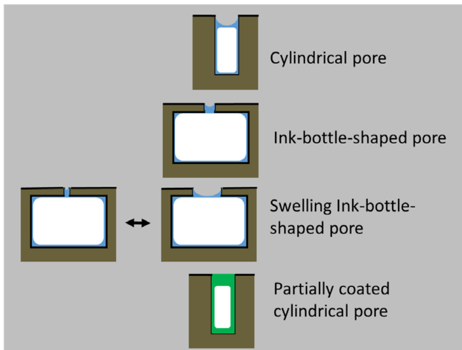
Figure 4. Pore types investigated for their capability to pre-activate. The pores are sketched in pre-activated state with ice inside. Colour code: white – ice; blue – water; green – concentrated solution; brown – pore wall. Note that at the wall and in the opening, a quasi-liquid layer of water or in case of the coated pore of concentrated solution is present.
