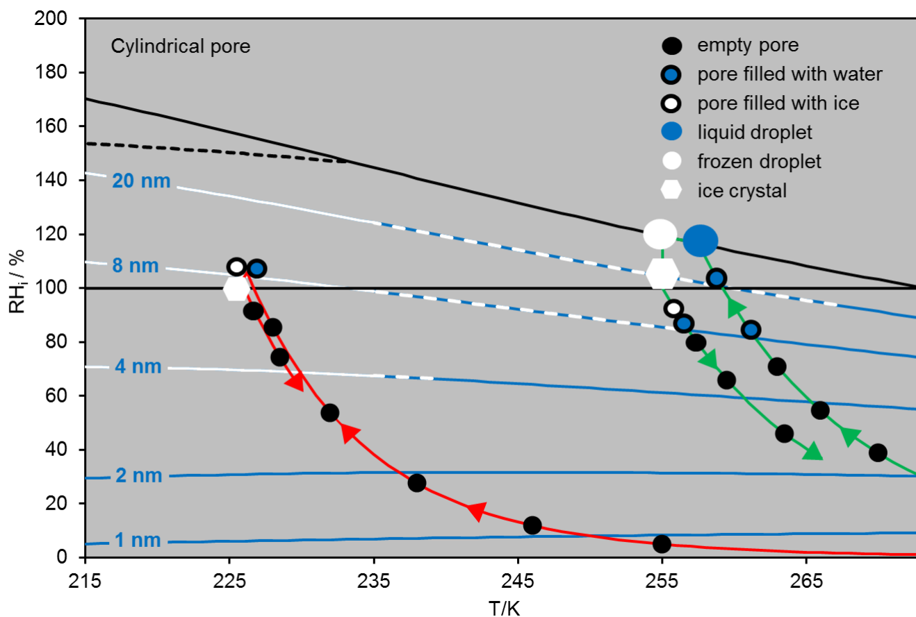
Figure 1. Wet trajectory (green line) and dry trajectory (red line) of a particle with a cylindrical pore of 8 nm diameter. Adiabatic cooling, followed by adiabatic heating. The black horizontal line denotes ice saturation; the black sloped line indicates RH_i/T conditions for water saturation (parameterization of Murphy and Koop, 2005). The black dashed line gives homogeneous ice nucleation according to Koop and Zobrist (2009). The white/blue lines delimit the onset of pore filling, which were calculated using the inverse Kelvin equation (Eq. 1). Pores with diameters given on the lines are filled at RH_i values above the line and empty below the line. The white portion denotes pore ice, the blue one pore water, and the dashed portion pore water or pore ice depending on the particle history.
