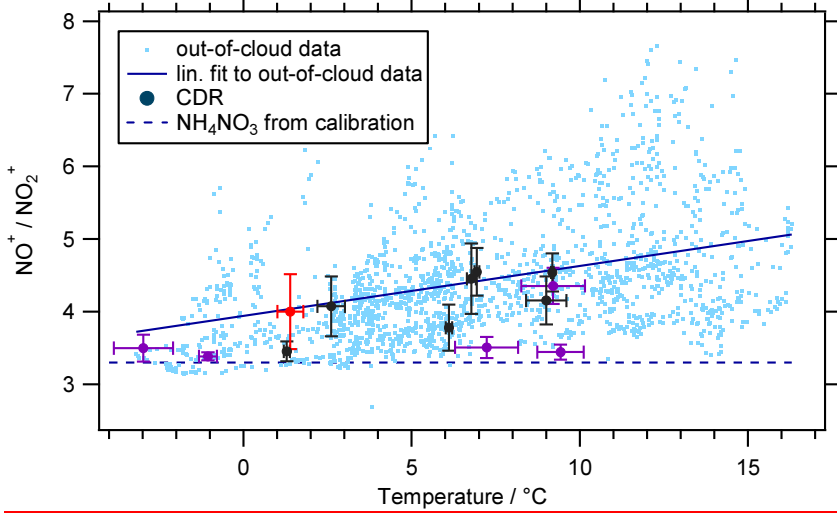
5 Figure 11: Ratio of \text{NO}^+ (m/z 30) to \text{NO}_2^+ (m/z 46) measured using the C-ToF-AMS as a function of temperature. Out-of-cloud data represent 15min averages, CDR data are averaged over the full cloud events, error bars denote standard deviation. The solid line is a linear fit to the out-of-cloud data, the dashed line shows the ratio obtained during calibration with pure \text{NH}_4\text{NO}_3 . The CDR data are color coded. Black: nighttime cloud events, purple dark grey : day and night, light grey-red : daytime event.
