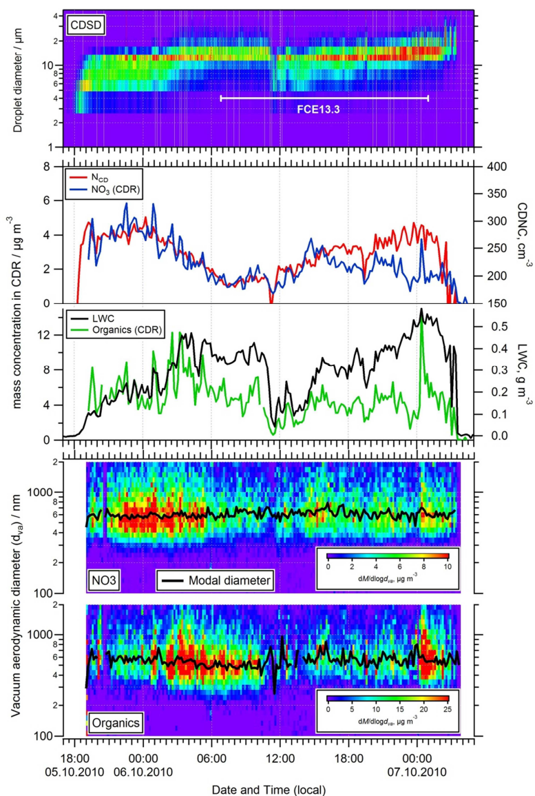
Figure 12: Example of the temporal evolution of cloud and residue properties on 06 October 2010. Upper panel: Cloud droplet size distribution (CDS) measured with the FSSP; Second panel: Cloud droplet number concentration (CDNC) measured with the FSSP along with nitrate mass concentration in cloud drop residues (CDR); Third panel: Liquid water content (LWC) measured by the PVM along with organic mass concentration in CDR; Forth and fifth panel: mass size distributions and modal diameter of nitrate and organics in CDR. All data represent 10min averages except for the CDS which is given on a 5sec time base.
