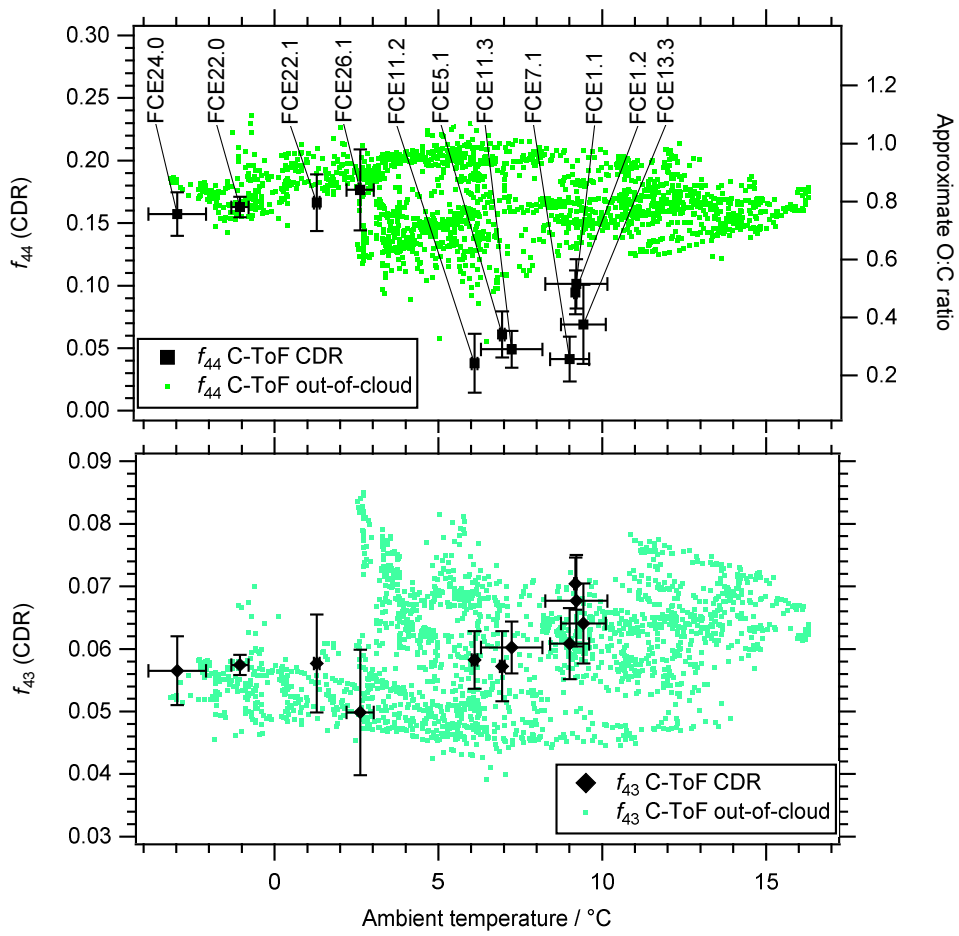
Figure 9: Upper panel: Ratio m/z44 to total organics ( f_{44} ) of cloud droplet residues (CDR) and out-of-cloud aerosol (both measured with the C-ToF-AMS) as function of temperature. The approximate O:C ratio inferred from f_{44} is given on the right axis. Lower panel: same graph but for f_{43} .
