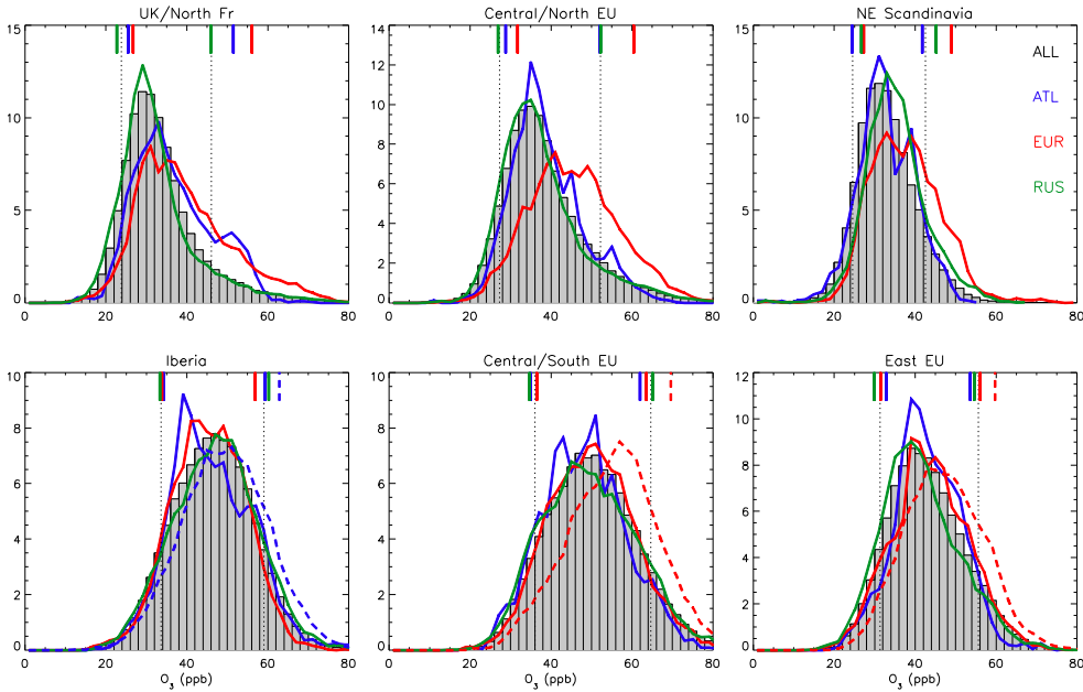
5 Figure 5: Spring (upper panels) and summer (lower panels) probability frequency distributions (%) of MDA8 O 3 for the six regional boxes presented in Figure 2 under different synoptic situations. Grey bars denote the 1998-2012 seasonal climatology. Solid lines correspond to days with block centres over the Atlantic (blue), European (red) and
