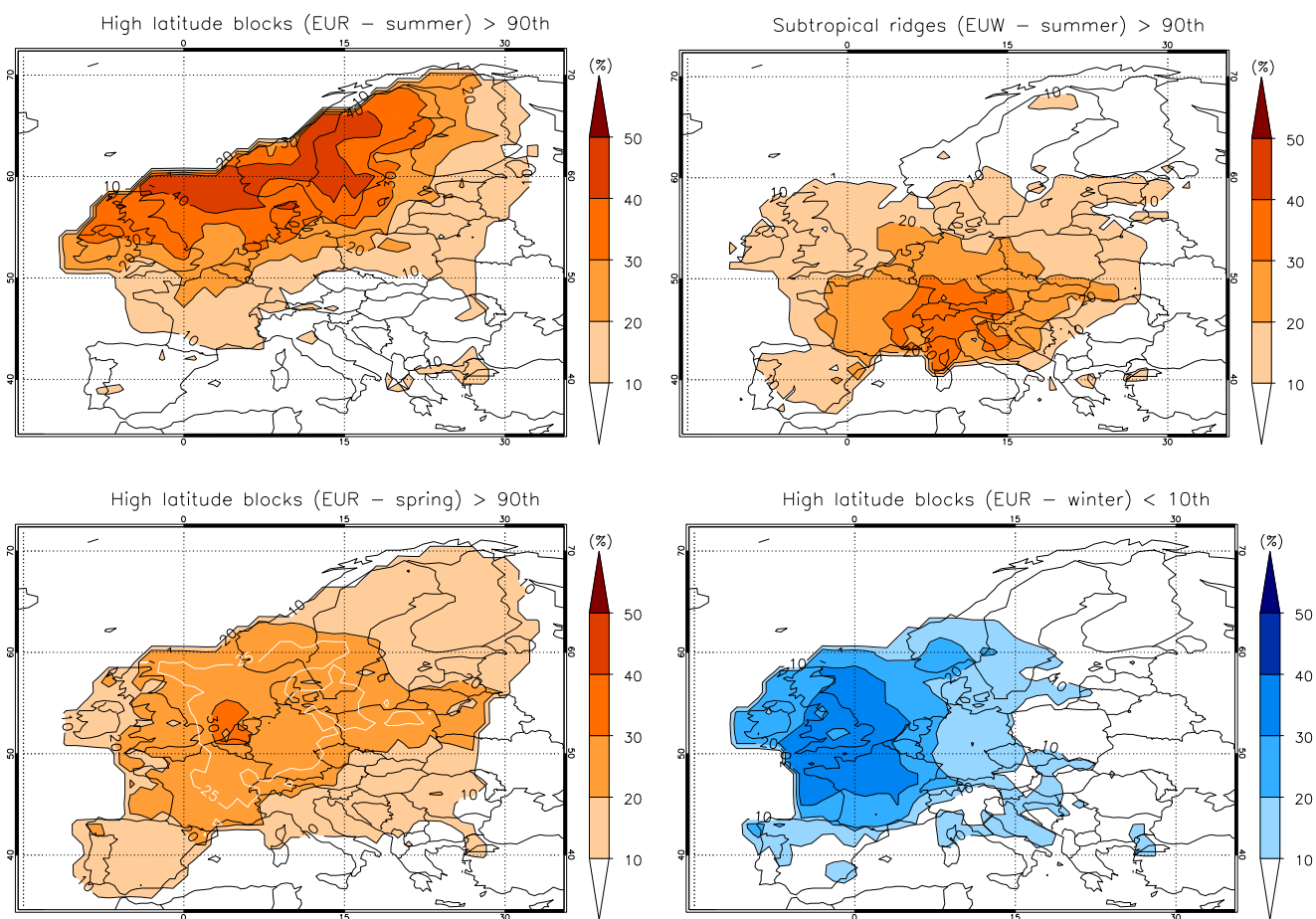
5 Figure 7: Percentage of EUR blocking days in summer (upper left) and spring (bottom left) as well as of days with ridges over the west of the EUR sector in summer ( 0^{\circ} – 15^{\circ} E, upper right) for which MDA8 O_3 is above the local 90 th percentile of its seasonal distribution. The lower right panel also shows the percentage of EUR blocking days with MDA8 O_3 below the 10 th percentile of its seasonal distribution in winter.
