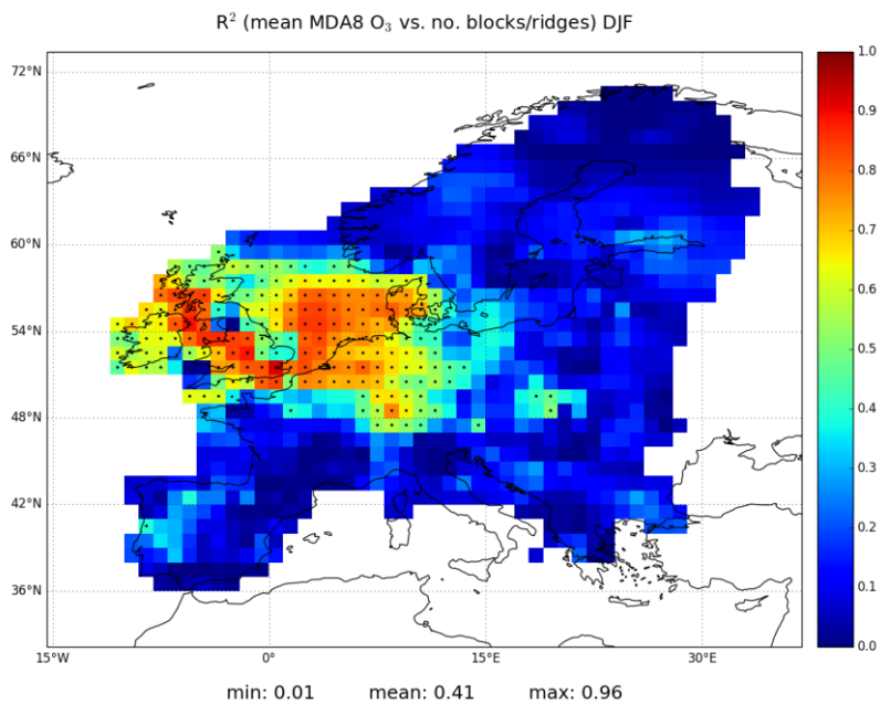
5 Figure 13: Coefficient of determination ( R^2 ) of two multiple linear models predicting the number of exceedances of the 90 th O_3 percentile in summer (top panel, Eq. 1) and the winter mean O_3 mixing ratios (bottom panel, Eq. 2) over each grid cell as a function of the interannual variability of blocks and ridges. Stippling indicates the locations where the multiple linear fits are significant at the 5 % level (F-test).
