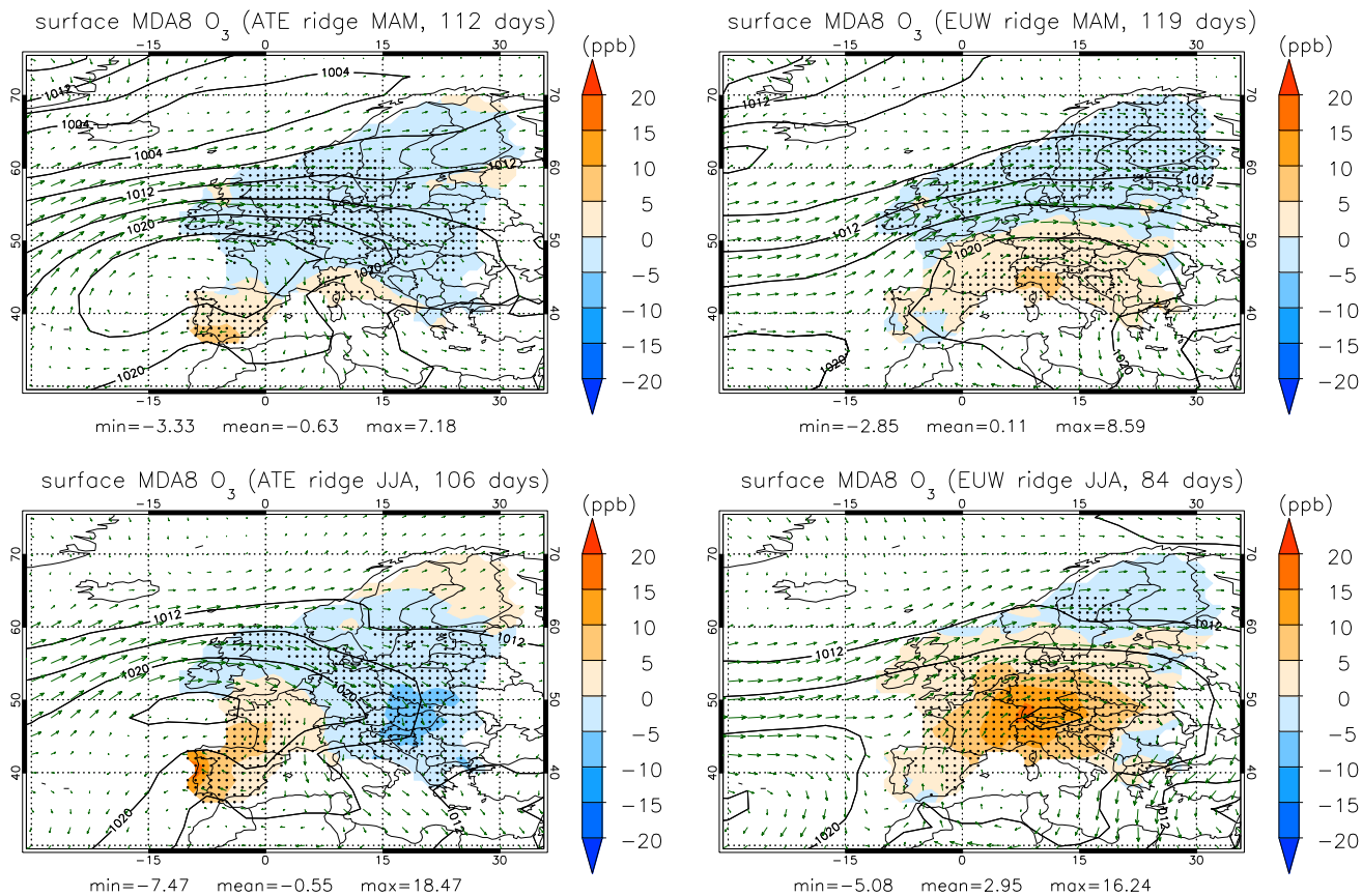
5 Figure 8: As Figure 4 but for subtropical ridges with centres over the East Atlantic (15°–0° W, left) and the west of the EUR sector (0°–15° E, right) in spring (top) and summer (bottom).
