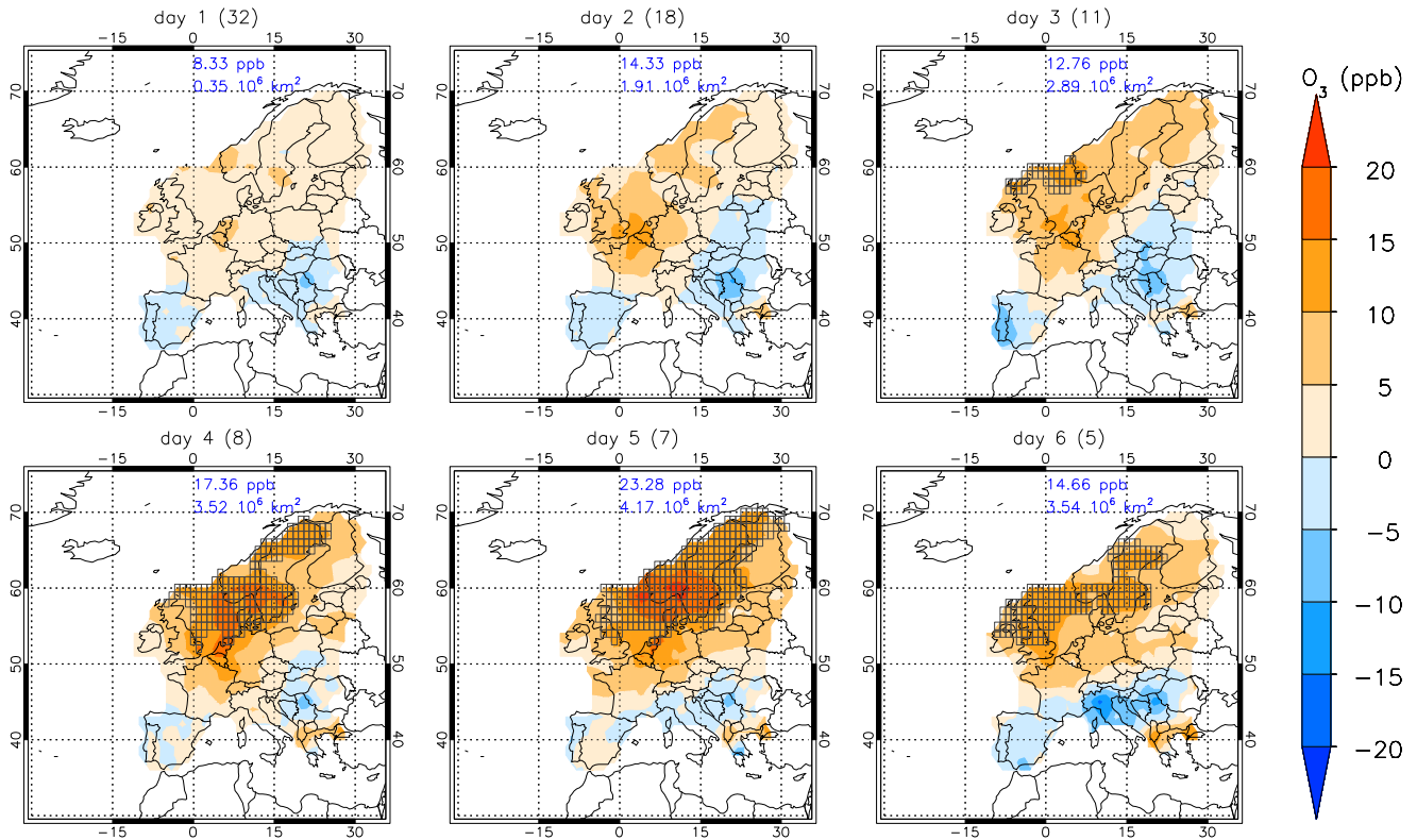
10 Figure 6: Evolution of MDA8 O 3 anomalies under the influence of EUR blocking in summer. The panels show, from left to right and from top to bottom, the average anomalies on the first six days a block is in the sector. The total number of blocks considered is given in brackets on the top of each panel. The maximum anomaly found (ppb) and the total area with anomalies higher than 5 ppb (km 2 ) are also indicated in blue colour. Grey open squares indicate grid cells where the ozone composite under blocking exceeds the 90 th percentile of the summer distribution.
