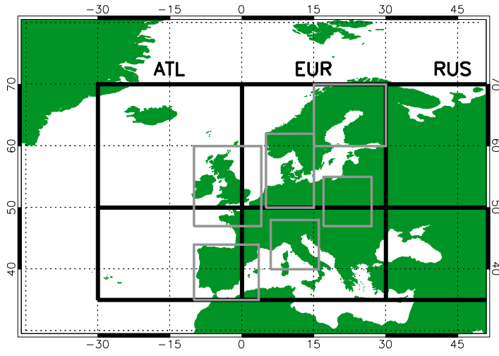
5 Figure 2: Longitudinal sectors considered for the identification of the centres of high latitude blocks (northern black boxes) and subtropical ridges (southern black boxes): Atlantic (ATL, 30°–0° W), European (EUR, 0°–30° E) and Russian (RUS, 30°–60° E, only partially shown). Grey boxes identify the geographic areas considered in the regional assessment performed in Sections 3 and 4. The regions considered, from west to east and from north to south, are ‘UK/North Fr’, ‘Central/North EU’, ‘NE Scandinavia’, ‘Iberia’, ‘Central/South EU’ and ‘East EU’.
