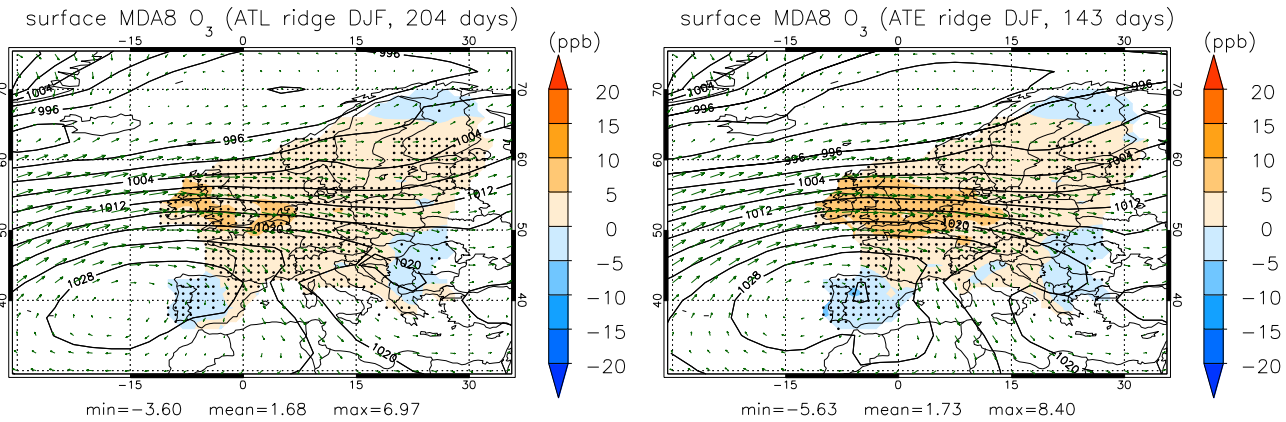
Figure 12: As Figure 4 but for subropical centres in the Atlantic ( 30^{\circ}-0^{\circ} W, left) and East Atlantic ( 15^{\circ}-0^{\circ} W, right) in winter.
