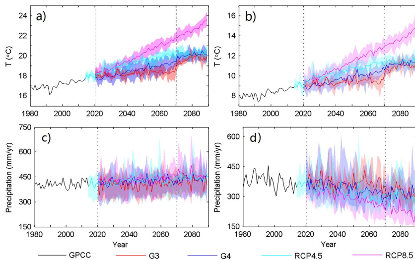
Fig. 3. Time series of summer mean bias-corrected temperature (a, b) and annual precipitation (c, d) averaged over the downscaled grid (section 3.2) in the whole region (a, c) and only in the glaciated region (b, d). Note the different temperature ranges in
