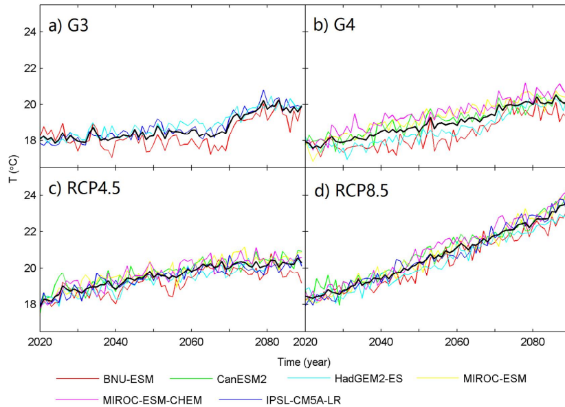
Fig. 2. Time series of summer mean bias-corrected temperature averaged over the downscaled grid in the whole HMA region projected by ensemble members after-model bias correction under climate scenarios G3 (a), G4 (b), RCP4.5 (c) and RCP8.5 (d). Black curve in each plot is the mean of the relevant ensemble (Table 3).
