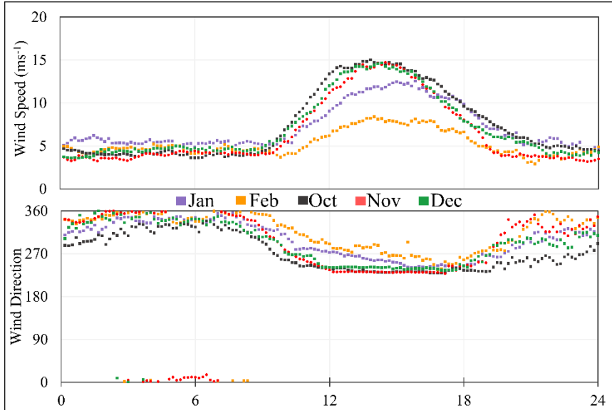
Supplement. Average diurnal variability in wind speed and direction for each month of 2013 at JSM_AWS_2 during the pre-monsoon (upper two panels), post-monsoon (middle two panels), and monsoon (lower two panels) periods.
