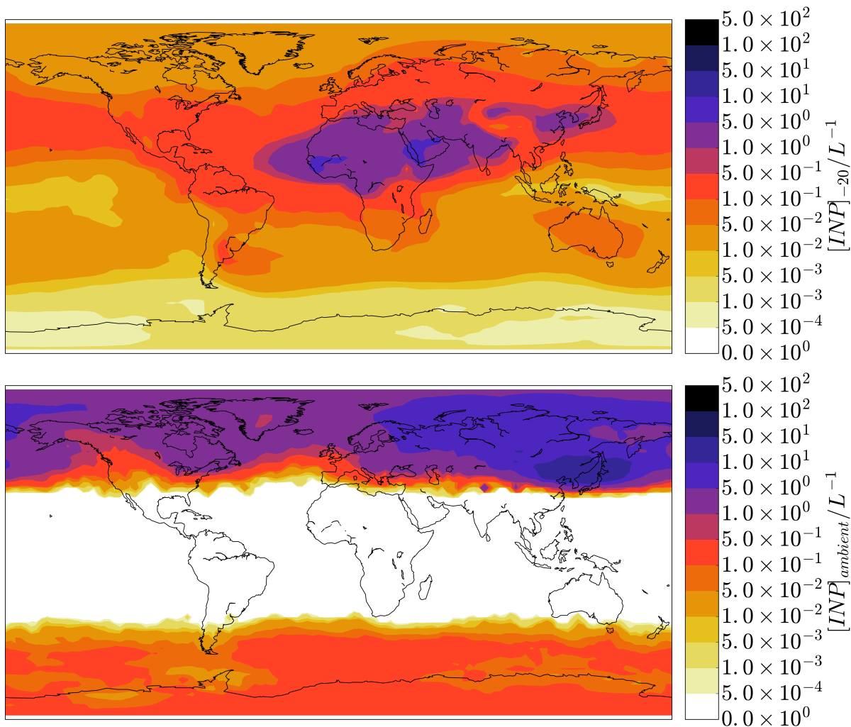
Figure 4. Annual mean K-feldspar INP distribution using GLOMAP-mode at a pressure level of 600hpa. Top panel shows the concentration of ice nucleating particles active at a temperature of -20^\circ C ( [INP]_T ) whereas the bottom panel shows the INP concentration at local ambient temperature ( [INP]_{ambient} ).
