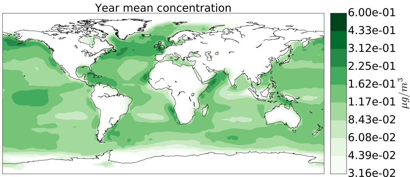
Figure 2. Annual mean mass concentration of sub-micron marine organic aerosol mass at surface level
