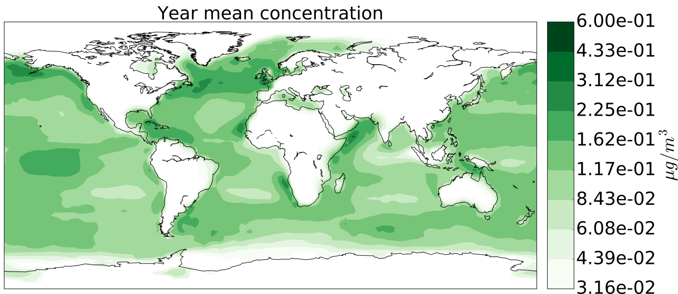
Figure 2. Annual mean surface mass concentration of sub-micron marine organic aerosols (WIOM) aerosol mass at surface level
