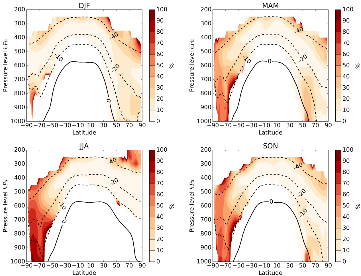
Figure 7. Percentage of days when [INP]_{\text{ambient}} from marine organic aerosols is greater than from K-feldspar. The number of days have been calculated only for times and locations where the total [INP]_{\text{ambient}} concentration is larger than 0.1m^{-3} . The black contour lines represent seasonal mean isotherms in degrees centigrade.
