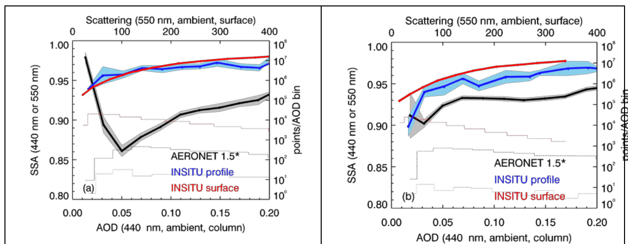
Figure 9. Systematic variability of SSA as a function of loading for (a) BND and (b) SGP for AERONET 1.5* AOD and SSA (black lines), AOD and SSA from in-situ profiles (blue lines) and in-situ scattering and SSA from surface measurements (red lines). Solid lines indicate mean values of SSA and AOD for each 0.05 AOD bin ( 10 \text{ Mm}^{-1} scattering bin). Shaded areas represent mean standard error (mean standard error for surface data is within thickness of red line). Histograms indicate the number of points in each AOD (or scattering) bin. Plot based on BND and SGP AERONET data (date range: 1996-2012) and BND INSITU profile data (date range: 2006-2012); SGP INSITU profile data (date range: 2006-2007). Surface data (orange lines) are for 550 nm, low RH, hourly in-situ data from the surface sites at BND (date range: 1997-2013) and SGP (date range: 1998-2013). AERONET 1.5* is from Level-1.5 retrievals with a corresponding Level-2 almucantar retrieval.
