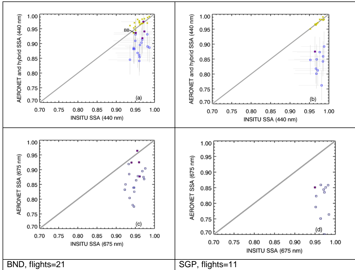
Figure 6. SSA comparison, (a) BND at 440 nm (b) SGP at 440 nm; (c) BND at 675 nm; and (d) SGP at 675 nm. Blue line is linear fit for all points shown; gray line is 1 to 1 line. Thin gray lines associated with each data point represent measurement uncertainties. Blue points show the average of all AERONET Level-1.5 AOD retrievals for which there was a successful AERONET Level-2 almucantar retrieval within \pm 3 hours of end of profile. Purple points indicate the few points for which there are AERONET Level-2 almucantar retrievals and where the average AERONET AOD 440 for those retrievals was greater than 0.2. The yellow points represent the 'hybrid SSA' which utilizes the AERONET AOD and the in-situ AOD to derive SSA as described in the text. The in-situ uncertainty lines here represent SSA uncertainty of 0.06 which is the worst case uncertainty.
