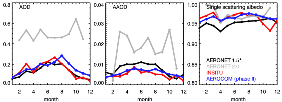
Figure 8b. Monthly medians of SGP aerosol optical properties at 440 nm. AERONET medians are for 1996-2011. In-situ data are for September 2005-December 2007. AERONET AOD medians are for observations with Level-2 almucantar retrievals, with corresponding AAOD and SSA retrievals at Level-1.5 (black) or Level-2 (gray). AERONET Level-2.0 almucantar AOD and AAOD values are biased high by definition, because of the AOD_{440} > 0.4 constraint. AERONET 2.0 direct sun retrievals (not shown) are similar to the AERONET 1.5 AOD values. In-situ values are derived from 322 flights over SGP. AeroCom Phase II median model results cover various time periods (depending on the model) and are reported at 550 nm.
