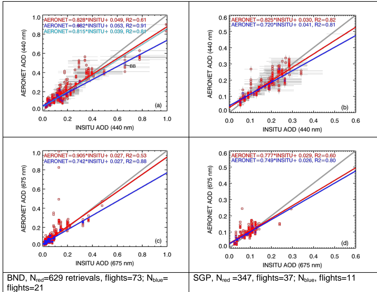
Figure 4. AOD comparison (a) BND at 440 nm; (b) SGP at 440 nm; (c) BND at 675 nm; and (d) SGP at 675 nm; thick gray line is 1 to 1 line. Thin gray lines associated with each data point represent measurement uncertainties. Red points and fit line represent all AERONET direct sun Level-2 AOD measurements within +/-3 hours of end of profile. Blue points and fit line represent the average of AERONET Level-2 AOD measurements with successful almucentar retrievals within +/-3 hours of end of profile. The light blue dashed line is the fit if the BB point is excluded. Note: two BND direct sun AOD440 points corresponding to the two highest AOD675 points in the figure below are off the scale of the plot and not shown. The third high AOD440 point is partly obscured by the legend.
