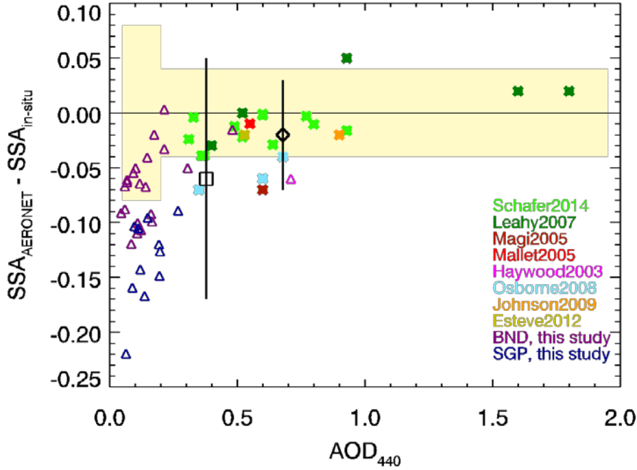
Figure 7. AOD_{440} vs [SSA_{AERONET} - SSA_{INSITU}] for direct comparisons studies listed in Table 4. Open symbols are for SSA_{440} difference; filled symbols are for SSA_{550} difference. AOD_{440} values for Leahy2007, Osborne2008, Johnson2009 use the Level-2 values reported on the AERONET webpage for the locations and dates of the specific profile. Shading indicates the combined standard uncertainty of AERONET SSA values as function of AOD as reported in Table 4 of Dubovik et al. (2000) and uncertainty in the in-situ SSA based on Figure 2. The black square and black diamond with vertical black lines represent, respectively, the mean and 2*standard deviation for all direct comparisons (including BND and SGP) and for literature direct comparisons only.
