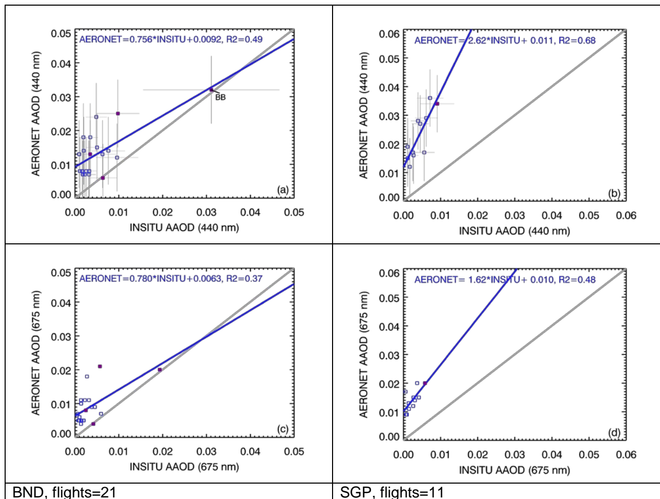
Figure 5. AAOD comparison, (a) BND at 440 nm; (b) SGP at 440 nm ; (c) BND at 675 nm; and (d) SGP at 675 nm. Blue line is linear fit for all points shown; gray line is 1 to 1 line. Thin gray lines associated with each data point represent measurement uncertainties. Points show the average of AERONET Level-1.5 AAOD retrievals for which there was a successful AERONET Level-2 almucantar retrieval within +/-3 hours of end of profile. Purple points indicate the few comparisons points for which there are AERONET Level-2 almucantar retrievals and where the average AERONET AOD 440 for those retrievals was great than 0.2.
