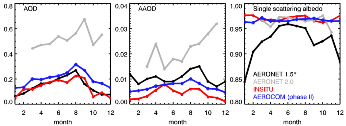
Figure 8a. Monthly medians of BND aerosol optical properties at 440 nm. AERONET medians are for 1996-2011. AERONET AOD medians are for observations with Level-2 almucantar retrievals, with corresponding AAOD and SSA retrievals at Level-1.5 (black) or Level-2 (gray). In-situ data are for June 2006-September 2009. AERONET Level-2.0 almucantar AOD and AAOD values are biased high by definition, because of the AOD_{440} > 0.4 constraint. AERONET 2.0 direct sun retrievals (not shown) are similar to the AERONET 1.5 AOD values. In-situ values are derived from 365 flights over BND. AeroCom Phase II median model results cover various time periods (depending on the model) and are reported at 550 nm.
