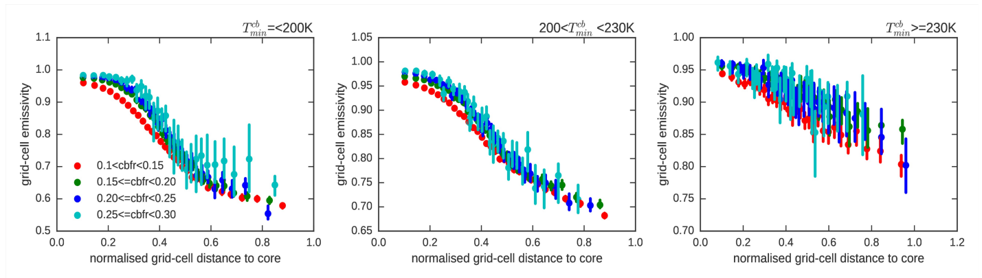
Figure 6. Emissivity within single core mature cloud systems as a function of the normalized distance to the convective core for four subintervals of convective fraction, separated in three groups wrt to convective intensity; Left: systems with T_{cb}^{min} \leq 200K , middle: 200 < T_{cb}^{min} \leq 230K and right: T_{cb}^{min} > 230K .
