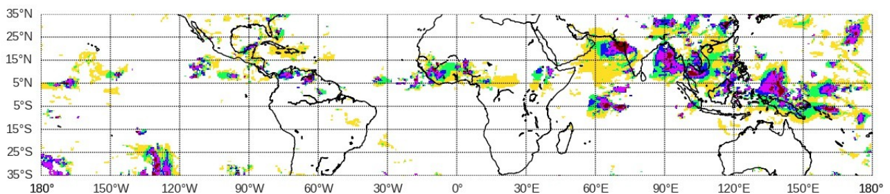
Figure 3. Geographical map of AIRS UT cloud emissivity for the 1 st of July 2007 AM, with each color indicating an emissivity class: \epsilon > 0.98 , \epsilon: 0.92-0.98 , \epsilon: 0.80-0.92 , \epsilon: 0.60-0.80 , \epsilon: 0.10-0.60 .
