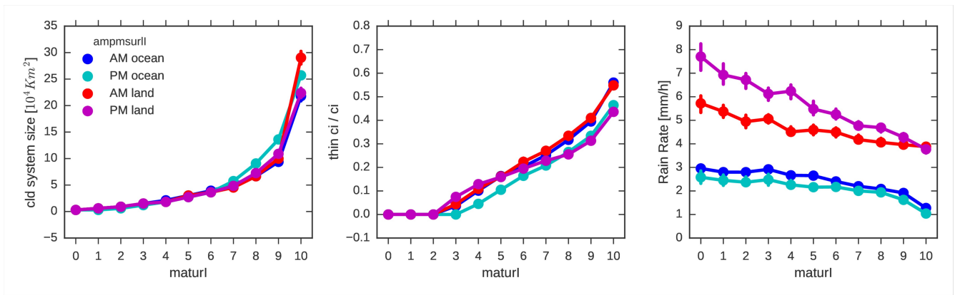
Figure 2. Median cloud system size (left), ratio of thin cirrus versus cirrus anvil (middle) and convective core average rain rate (right) as a function of maturity steps, including single and multi-core systems.
