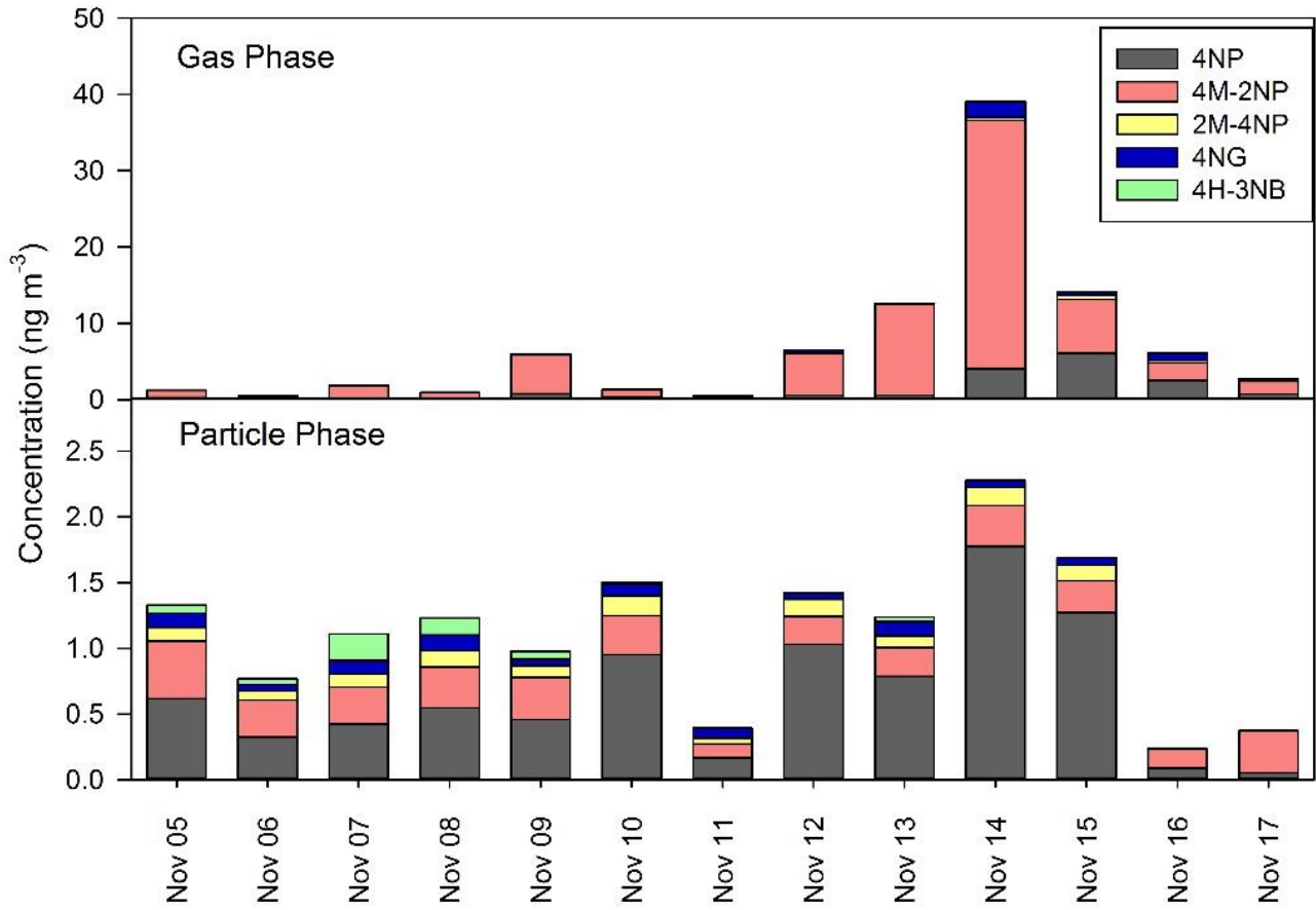
Figure S3: Daily gas and particle concentrations of select nitroaromatics detected in Iowa City during fall 2015, including 4-nitrophenol (4NP), 4-methyl-2-nitrophenol (4M-2NP), 2-methyl-4-nitrophenol (2M-4NP), 4-nitroguaiacol (4NG), and 4-hydroxy-3-nitrobenzyl alcohol (4H-3NB).
