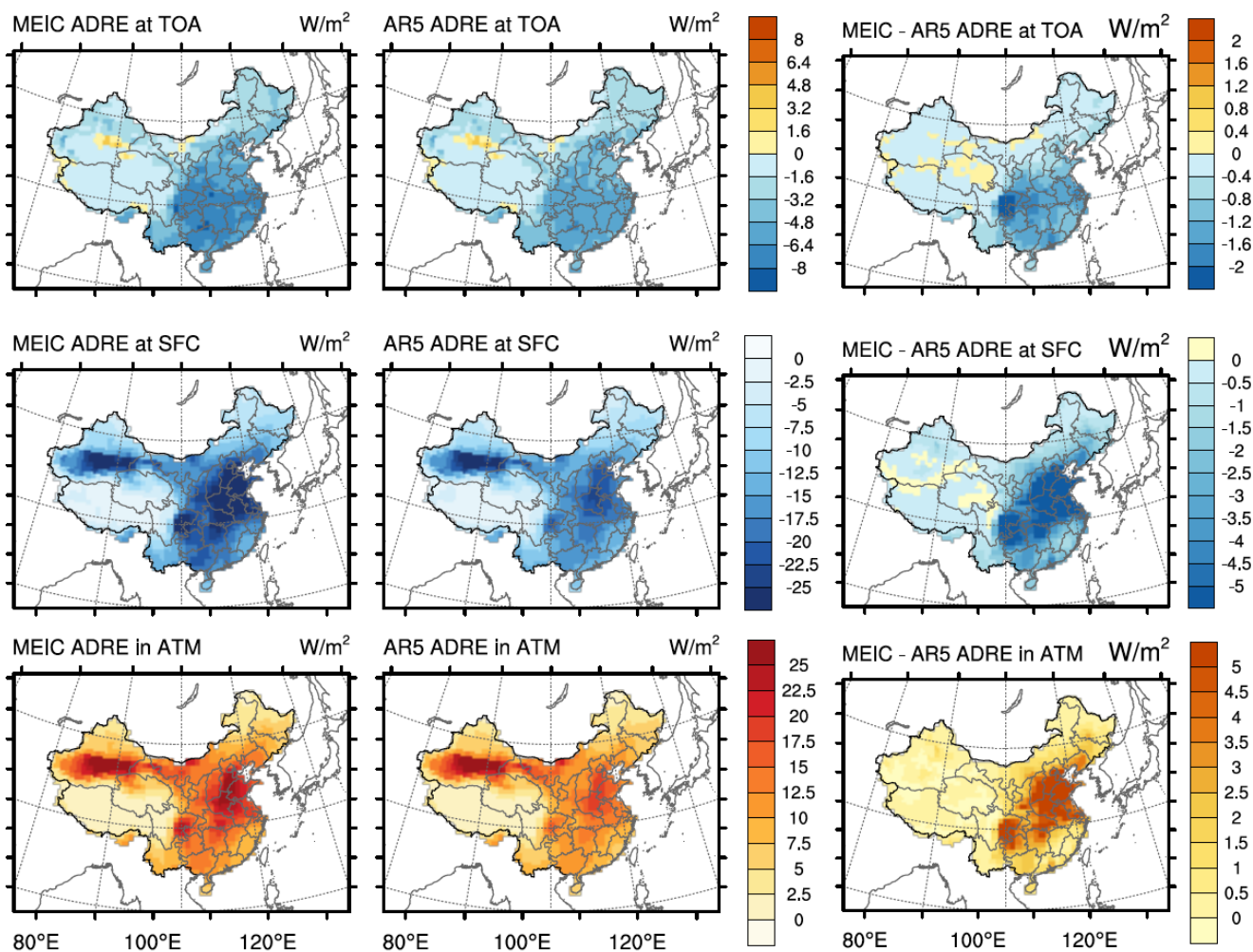
735 Figure 12. Spatial distributions of the annual averaged aerosol direct radiative effects (ADREs) at TOA, surface (SFC) and in the atmosphere (ATM) using the MEIC and the AR5 emissions and their differences.
