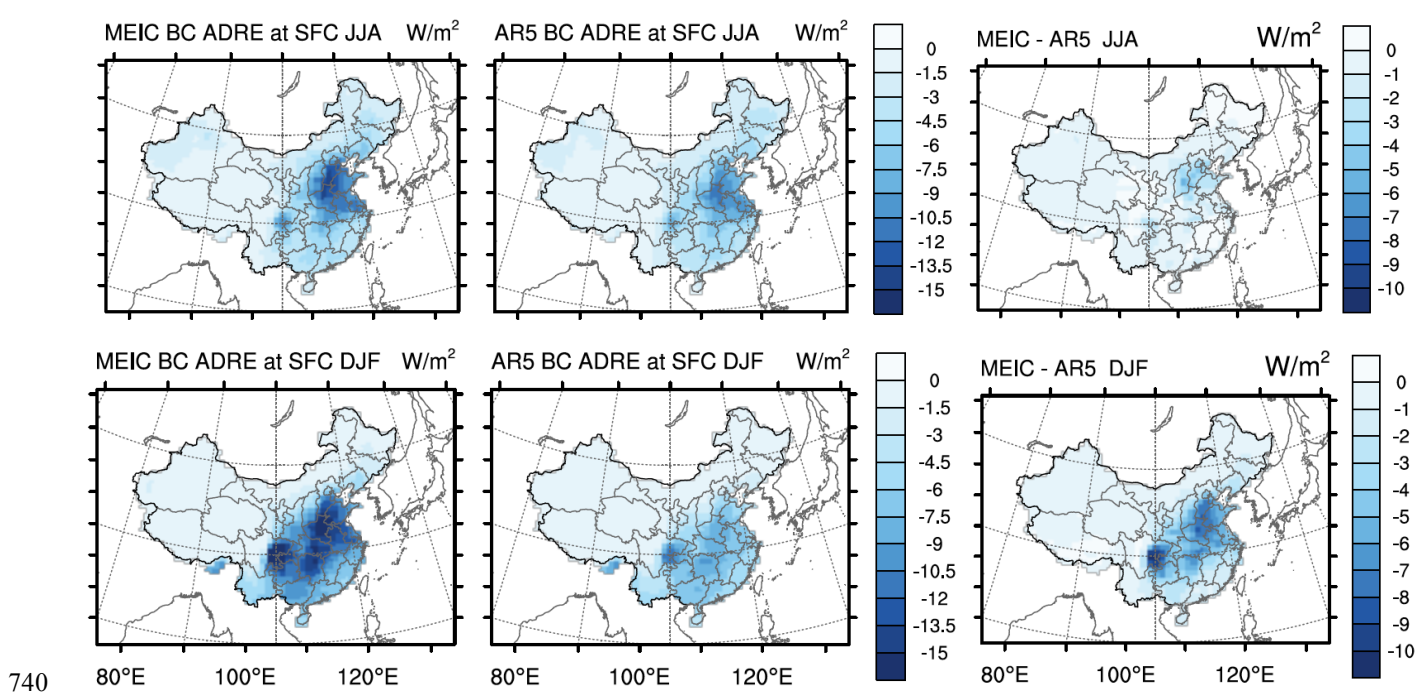
Figure 13. Spatial distributions of ADREs of BC in summer (June, July, August) and the winter (December, January, February) at the surface (SFC).
