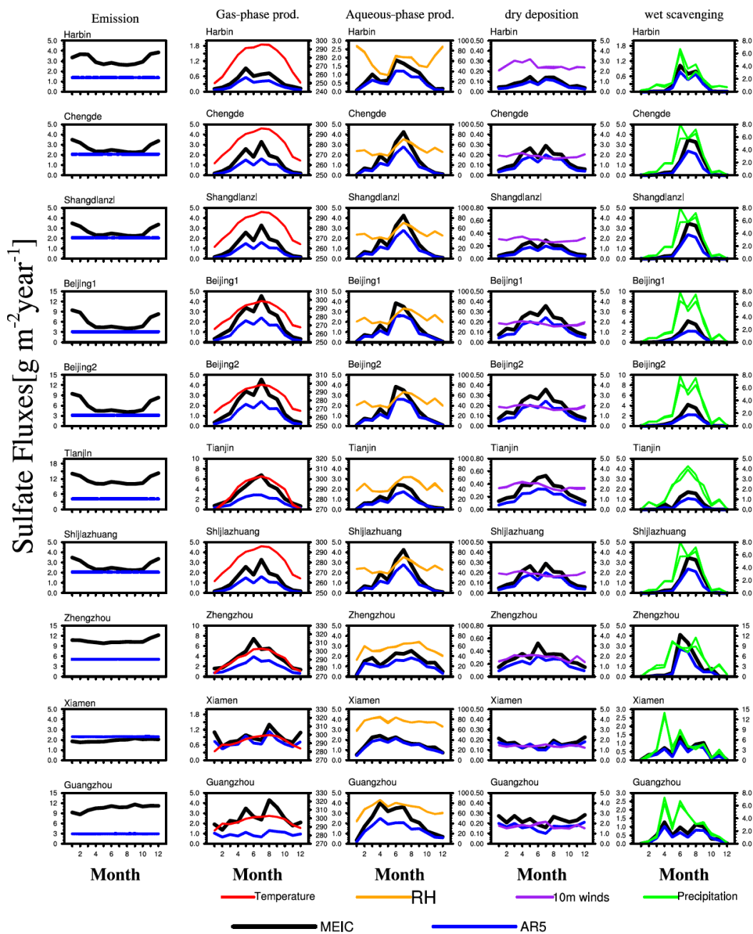
Figure 9. From left to right columns: (1) SO 2 emission rates from the MEIC (black) and the AR5 (blue) emission inventories, model simulations of (2) gas-phase chemistry production rates in the simulations by MEIC and AR5 and the surface temperature (red), (3) aqueous-phase production rates and the relative humidity at surface (yellow), (4) dry deposition rates and the 10-meter wind speed (purple), and (5) wet scavenging rates and the precipitation rate (green).
