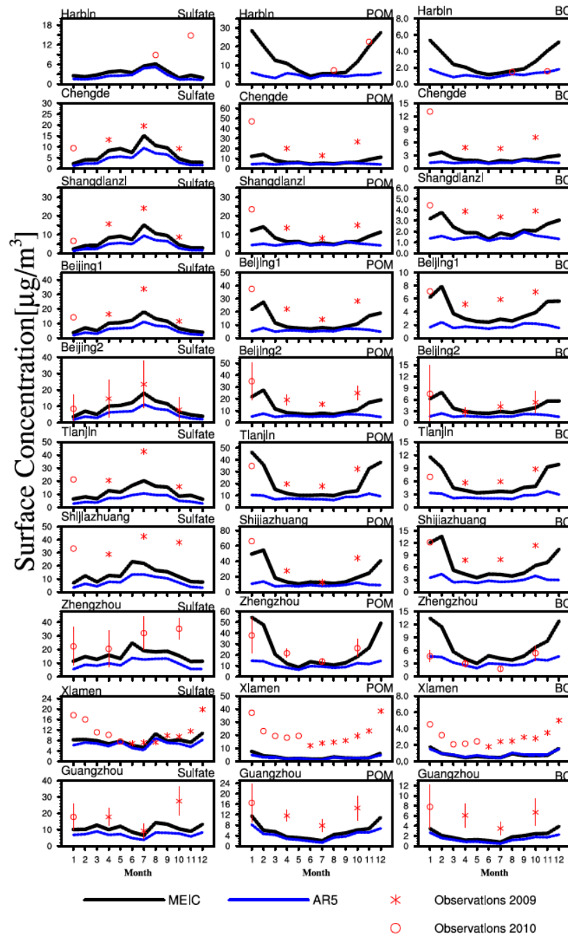
Figure 8. The seasonal variations of monthly averaged surface concentrations of sulfate, POM, and BC modeled by CAM5-MAM3 using the MEIC and the AR5 emissions compared with the observations. Error bars stand for one standard deviation.
