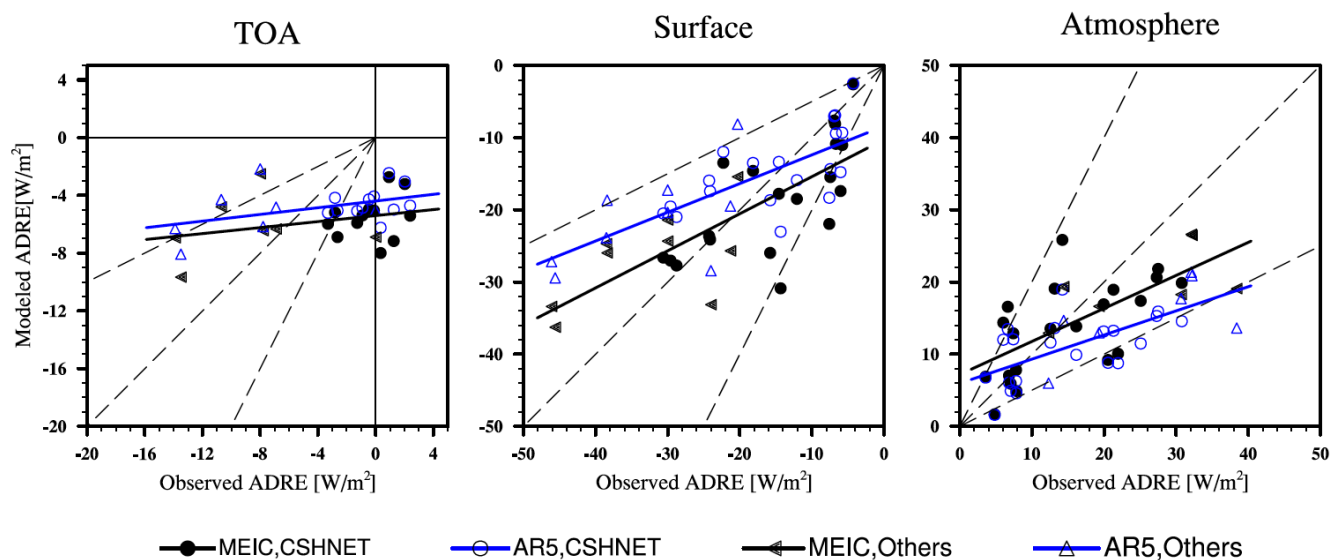
Figure 15. ADREs at TOA, surface, and atmosphere modeled by CAM5-MAM3 using the MEIC and the AR5 emissions compared with ADRE observations from CSHNET and other observations in China (Table S3).
