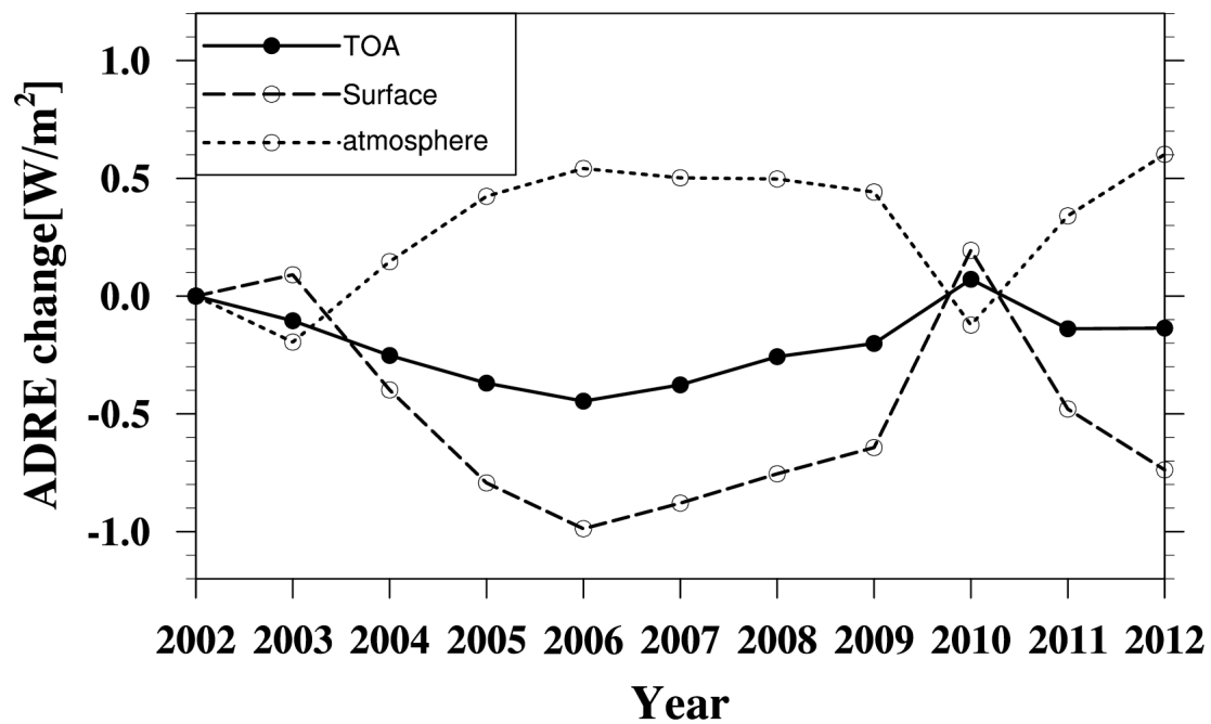
760 Figure 16. The change of ADREs at TOA, surface and in the atmosphere relative to year 2002 due to the emission change from 2002 to 2012 in eastern China estimated by the MEIC development team.
