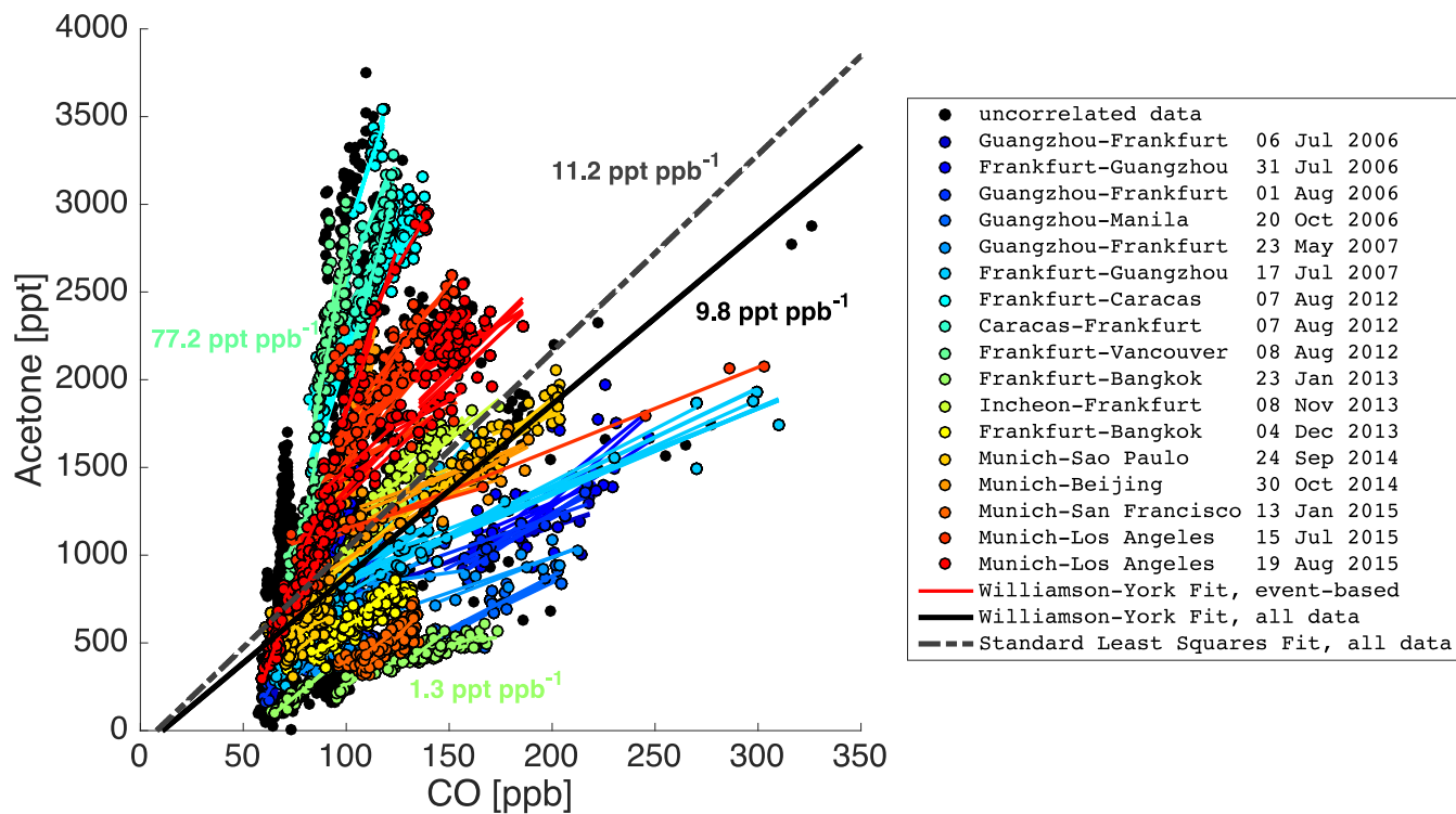
5 Figure 3: Scatter plot of tropospheric acetone and CO data of 17 selected CARIBIC flights. Detected correlations are shown as regression lines plotted in the range of the underlying data. Colorcoding denotes to which flight data and correlations belong to. Data, which did not fall into our event-based correlation criteria, are shown as filled black circles regardless of their flight affiliation. The solid black and the grey dashed line represent the results of a Williamson-York fit (EnR: 9.8 ppt ppb -1 ) and of a standard least-squares fit (EnR: 11.2 ppt ppb -1 ), respectively, applied to all data of the 17 flights. The minimum, mean and maximum value of the event-based EnRs are 1.3, 18.6 and 77.2 respectively (all values in ppt ppb -1 ).
