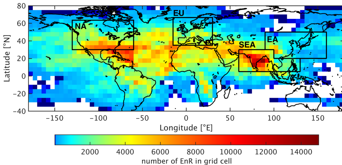
Figure 8: Geographical distribution of EnRs duplicated along the waypoints of the assigned 5-day back trajectories. Grid cells without data are left blank. Four areas of interest (rectangles) are considered: North America (NA), Europe (EU), Southeast Asia (SEA) or East Asia (EA).
