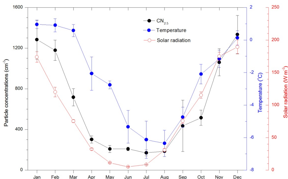
Figure S4. A comparison of monthly variations of CN 2.5 concentrations, temperature, and solar radiation during whole observation period.
