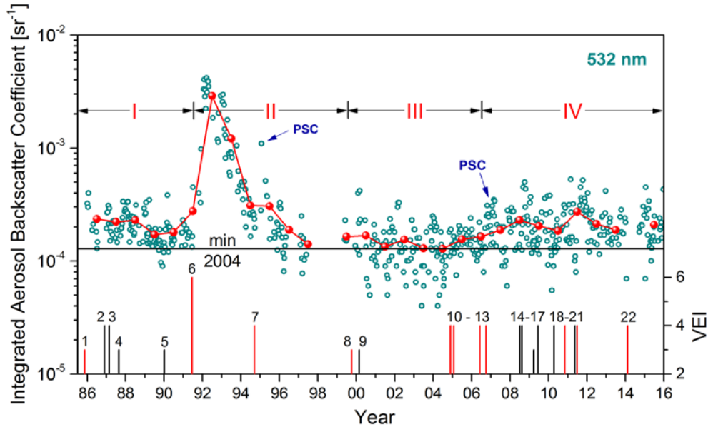
Figure 1. 30-year time series of the integrated stratospheric backscatter coefficient at \lambda = 532 nm over Tomsk between 15 and 30 km.
