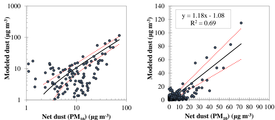
Figure 2_RC1: Regression analysis between net dust calculated through PM 10 regional background data and dust concentrations modelled at surface level by SKIRON/Dust for the city of Athens, in log-log (left) and linear scale (right). The black line corresponds to the linear regression equation, while the red dotted lines are the upper and lower bounds, at 95% confidence interval.
