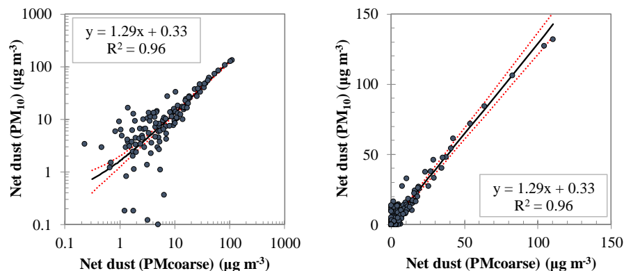
Figure 1_RC1: Regression analysis of Net dust concentrations calculated from regional background PM 10 and PMcoarse (PM 2.5-10 ) concentrations for Athens, in log-log (left) and linear scale (right). The black line corresponds to the linear regression equation, while the red dotted lines are the upper and lower bounds, at 95% confidence interval.
