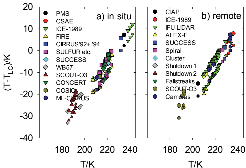
Figure 6 Difference the between ambient temperature ( T ) and the threshold temperature ( T_{LC} ) versus T for a) in-situ and for b) remote-sensing contrail observations. The larger symbols depict T - T_{LC} when T_{LC} is computed for the measured or estimated humidity, the smaller symbols when computed for assumed liquid saturation. The symbols refer to the same projects as in Figures 1 and 2 (WB-57 refers to CRYSTAL-FACE and CR-AVE, which both used this aircraft).
