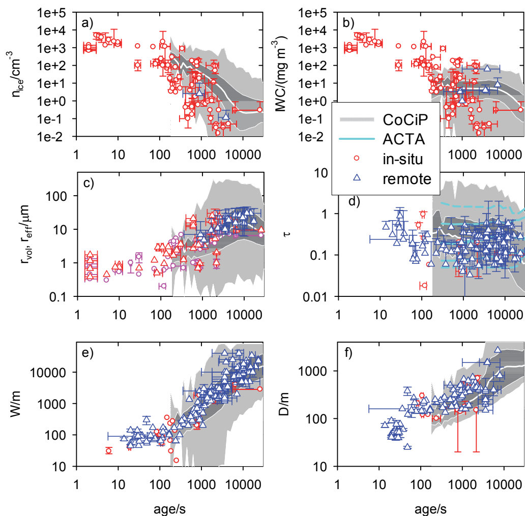
Figure 3 Local contrail parameters from all observations collected in COLI versus contrail age, together with results from a model simulation (CoCiP percentiles) as in Figure 1 . a) n_{ice} , b) IWC, c) r_{vol} (purple symbols), r_{eff} (red and blue symbols), d) \tau , e) W , f) D . The red (and purple) symbols are from in-situ measurements. The blue symbols are from remote sensing.
