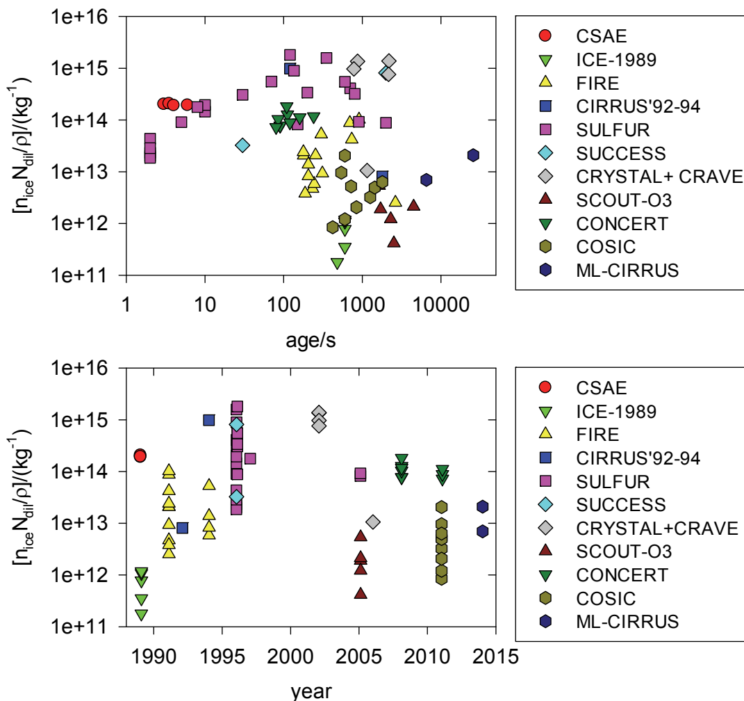
Figure 8 Particle concentrations n_{ice} normalized to density and an empirical dilution law, approximating an apparent particle emission index, PEI_{ice} (the number of ice particles in the contrail per burnt fuel mass). b) Same quantity versus year of measurement.
