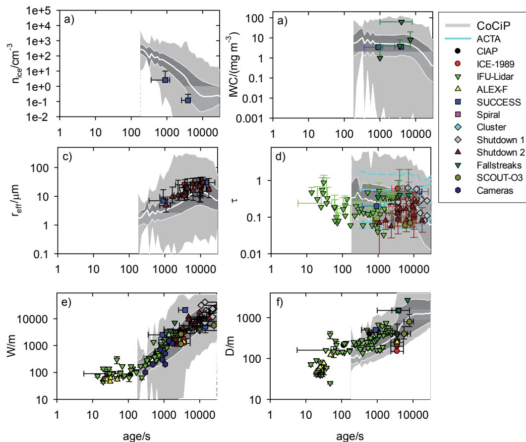
Figure 2 Same as Figure 1 for remote-sensing data. Panel a) ice particle concentration n_{ice} , b) IWC, c) effective radius r_{eff} , d) optical depth \tau at solar wavelengths, e) width W , f) depth D . The cyan lines in panel d) depict mean values of optical depth \tau derived from 25600 ACTA results (0, 10, 50, 90, 100 percentiles)
