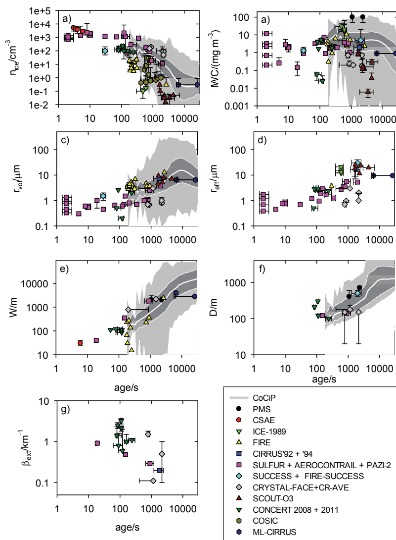
Figure 1 Contrail parameters from in-situ observations versus contrail age, together with results from a model simulation (CoCiP). Panel a) Number concentration of ice particles n_{ice} in cm^{-3} , b) ice water content IWC in mg\ m^{-3} , c) volume mean radius r_{vol} in \mu m , d) effective radius r_{eff} in \mu m , e) contrail width W in m , f) total contrail depth D in m , g) optical extinction \beta_{ext} in km^{-1} . The grey-shadowed white lines depict mean CoCiP results (0, 10, 50, 90, 100 percentiles); the thick white line is the median value (50%). Various symbols denote various observation projects (or group of projects), see Table 7. Error bars, as far as available, indicate estimated ranges of variability during the measurements and reflect uncertainties (e.g., in age).
