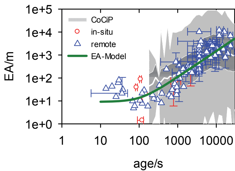
Figure 9 Total extinction EA versus time: Data (symbols as before) and a simple model (full dark green curve).
