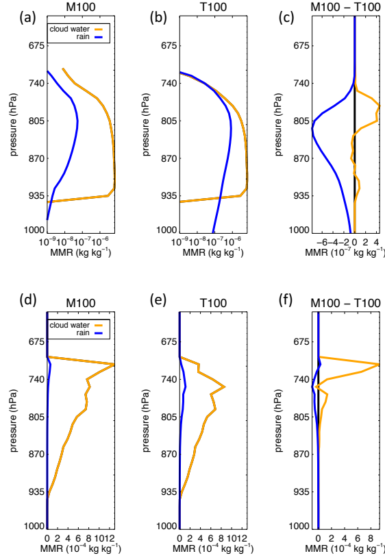
Figure 11. RICO case: Mean vertical profiles of hydrometeor mass mixing ratios (MMR), as Figure 6, averaged over the 24 h of the RICO simulation. (a) RICO-M100 domain-mean, (b) RICO-T100 domain-mean, (c) RICO-M100 domain-mean minus RICO-T100 domain-mean, (d) RICO-M100 condensate-mean over each hydrometeor class, (e) RICO-T100 condensate-mean, (f) RICO-M100 condensate-mean minus RICO-T100 condensate-mean. Note that because the rain amounts are very small, especially in M100, (a) and (b) are shown with a logarithmic horizontal axis.
