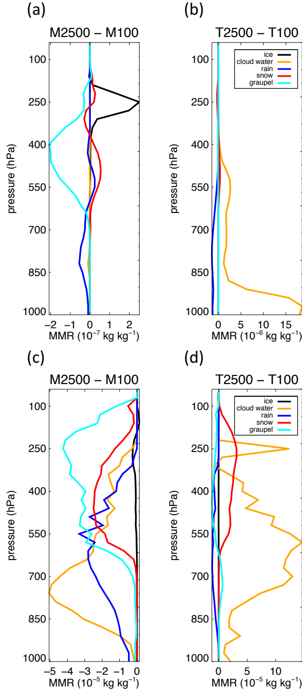
Figure 7. Congo case: Difference in the mean hydrometeor mixing ratio profiles under polluted and pristine conditions averaged over the period 1–10 August 2007. (a) CONGO-M2500 domain-mean minus CONGO-M100 domain-mean, (b) CONGO-T2500 domain-mean minus CONGO-T100 domain-mean, (c) CONGO-M2500 mean over all condensed points of each hydrometeor class minus CONGO-M100 mean over all condensed points, and (d) CONGO-T2500 mean over all condensed points minus CONGO-T100 mean over all condensed points.
