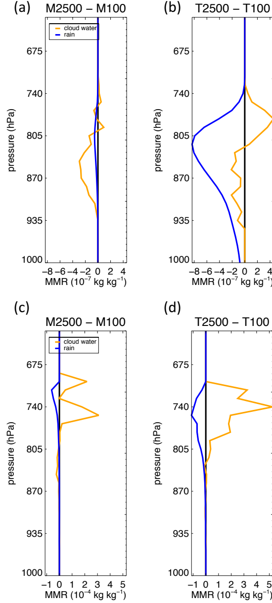
Figure 12. RICO case: difference in the mean hydrometeor mixing ratio profiles under polluted and pristine conditions, as Figure 7, averaged over the 24 h of the RICO simulation. (a) RICO-M2500 domain-mean minus RICO-M100 domain-mean, (b) RICO-T2500 domain-mean minus RICO-T100 domain-mean, (c) RICO-M2500 condensate-mean over each hydrometeor class minus RICO-M100 condensate-mean, (d) RICO-T2500 condensate-mean minus RICO-T100 condensate-mean
