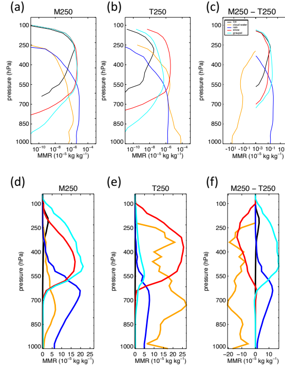
Figure 6. Congo case: Mean vertical profiles of hydrometeor mass mixing ratios (MMR) averaged over the period 1–10 August 2007. (a) CONGO-M250 domain-mean, (b) CONGO-T250 domain-mean, (c) the difference in the domain-mean hydrometeor mixing ratio profiles (CONGO-M250 minus CONGO-T250), (d) CONGO-M250 mean over condensed points only, (e) CONGO-T250 mean over condensed points only for each hydrometeor class, and (f) the difference in the condensate-mean hydrometeor mixing ratio profiles (CONGO-M250 minus CONGO-T250). Note the logarithmic horizontal axis used in (a), (b) and (c) due to the total difference between the hydrometeor classes simulated by the two schemes spanning several orders of magnitude.
