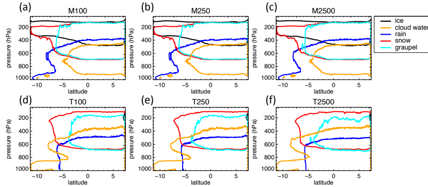
Figure 4. Congo case: Zonal mean vertical sections of hydrometeor classes (colour contours) from 01 to 10 August 2007. Hydrometeor mass mixing ratios are contoured at 10^{-6} \text{ kg kg}^{-1} .
