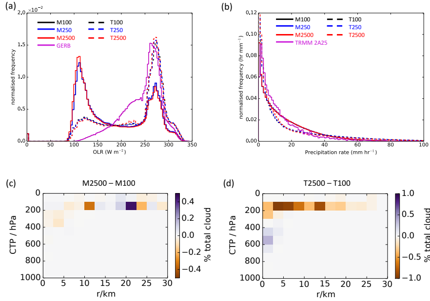
Figure 2. Congo case: (a) frequency distributions of OLR from the WRF simulations and observations from GERB over the period 01 to 10 August 2007 , (b) self-weighted precipitation rate distributions from the WRF simulations and observations from the ungridded TRMM 2A25 product, which has a similar spatial resolution to the 4 km model grid length, (c) difference in the joint distribution of cloud top pressure in updraughts (identified by masking points where the maximum vertical velocity exceeds 1 \text{ ms}^{-1} , and then applying a connected-components labelling algorithm to identify unique updraught areas ) and horizontal radius of updraughts when CDNC is increased from 100 to 1000 \text{cm}^{-3} using the Morrison microphysics scheme, (d) difference in the joint distribution of cloud top pressure in updraughts and horizontal radius of updraughts when CDNC is increased from 100 to 1000 \text{cm}^{-3} using the Thompson microphysics scheme
